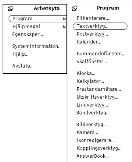
Figur 1-13 Undermenyn Program
