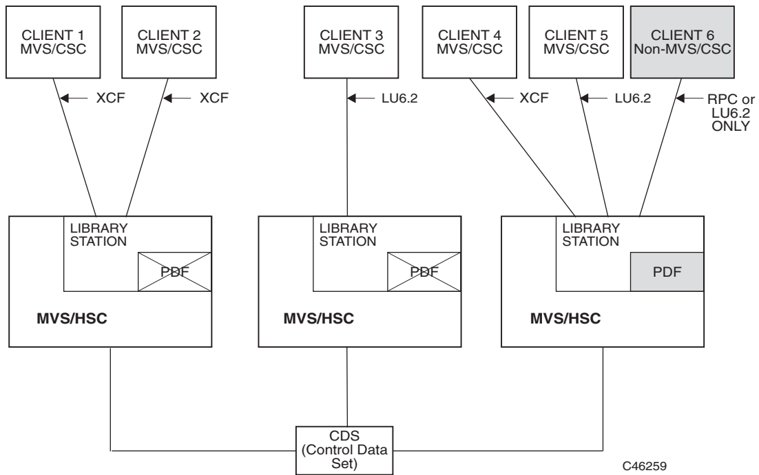
FIGURE 2-6 Sysplex Environment with Heterogeneous Support
