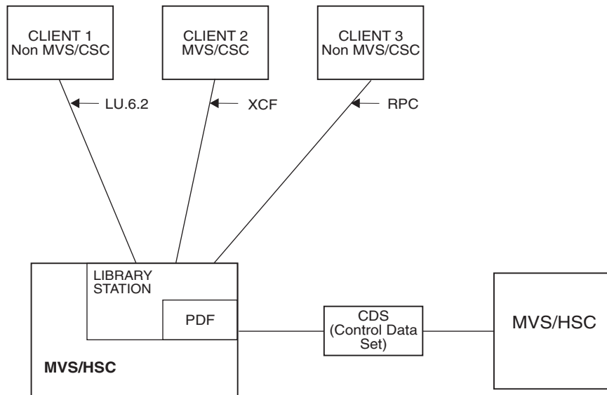
FIGURE 2-4 Heterogeneous Environment
