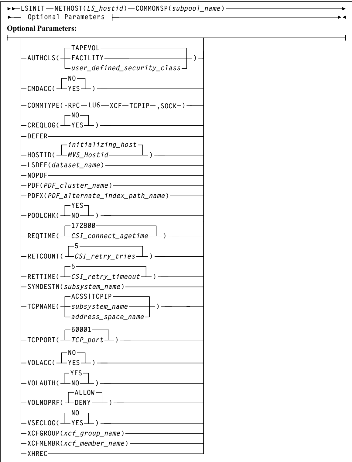
FIGURE 2-12 LSINIT Control Statement Syntax
