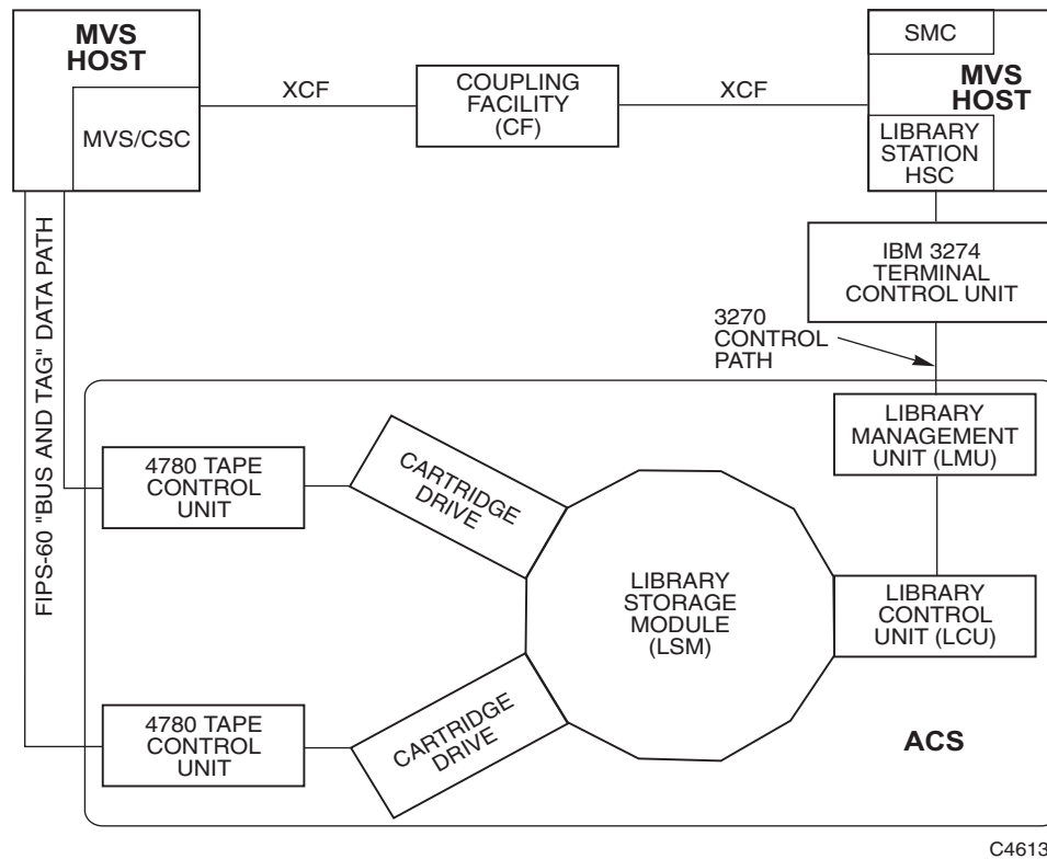
FIGURE 2-3 Typical LibraryStation Sysplex Configuration
