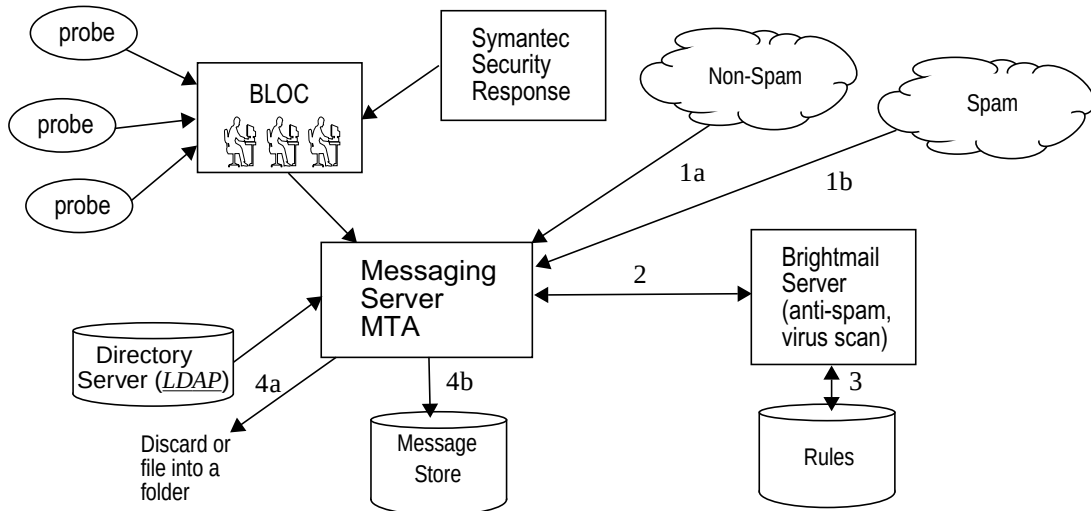
Figure 11-1 Brightmail and Messaging Server Architecture
