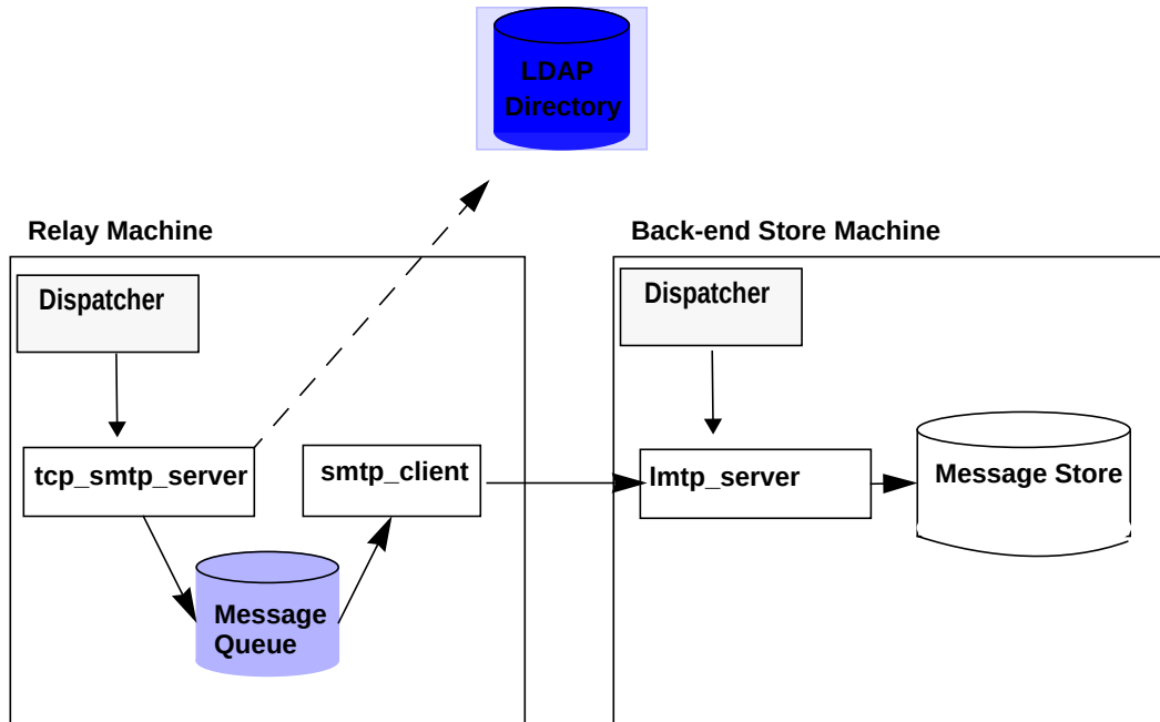
Figure 12-2 Two Tier Deployment With LMTP
