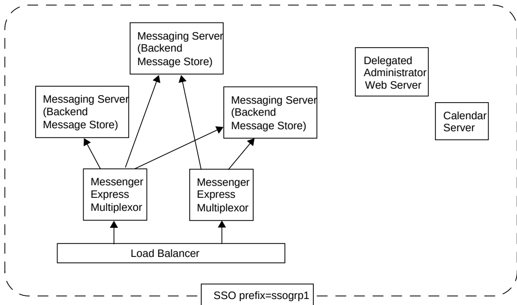
Figure 4-2 Complex SSO Deployment
