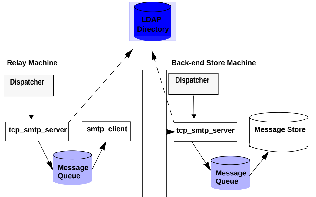
Figure 12-1 Two Tier Deployment Without LMTP
