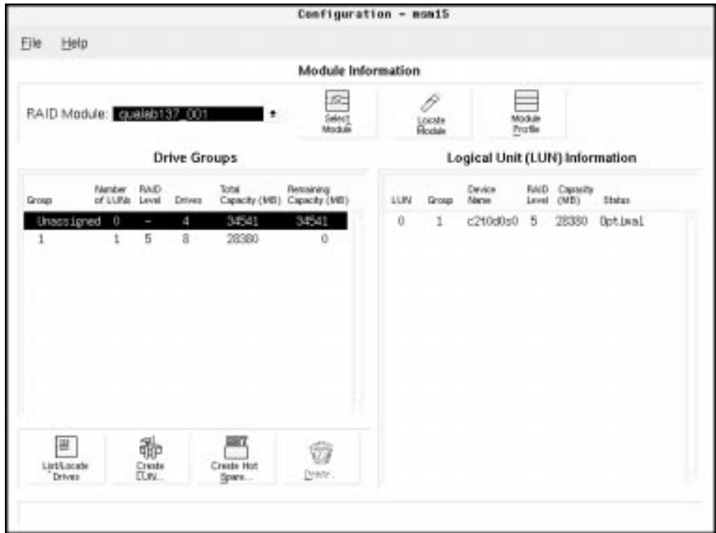
FIGURE 2-4 Main Configuration Screen
