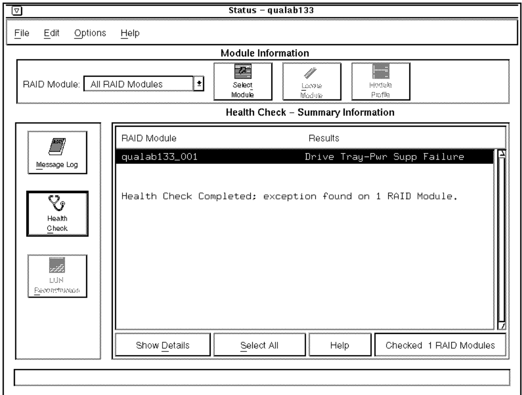
FIGURE 2-3 Health Check Screen
