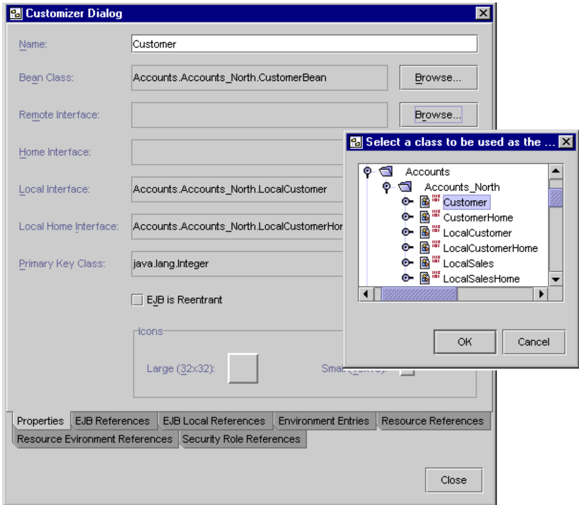
FIGURE 9-5 Customizer for Adding an Interface Class to a Bean
