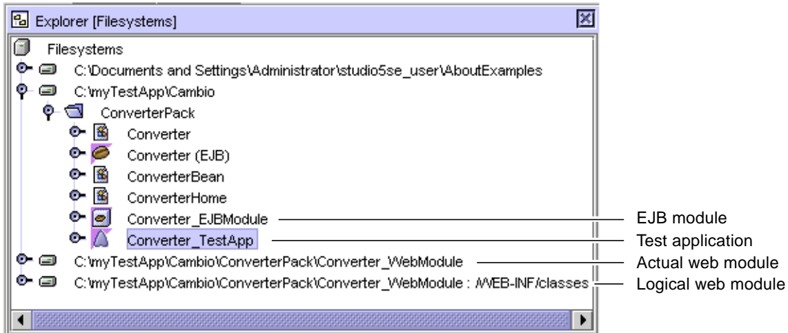
FIGURE 9-2 Example of Test Objects Generated for Enterprise Beans
