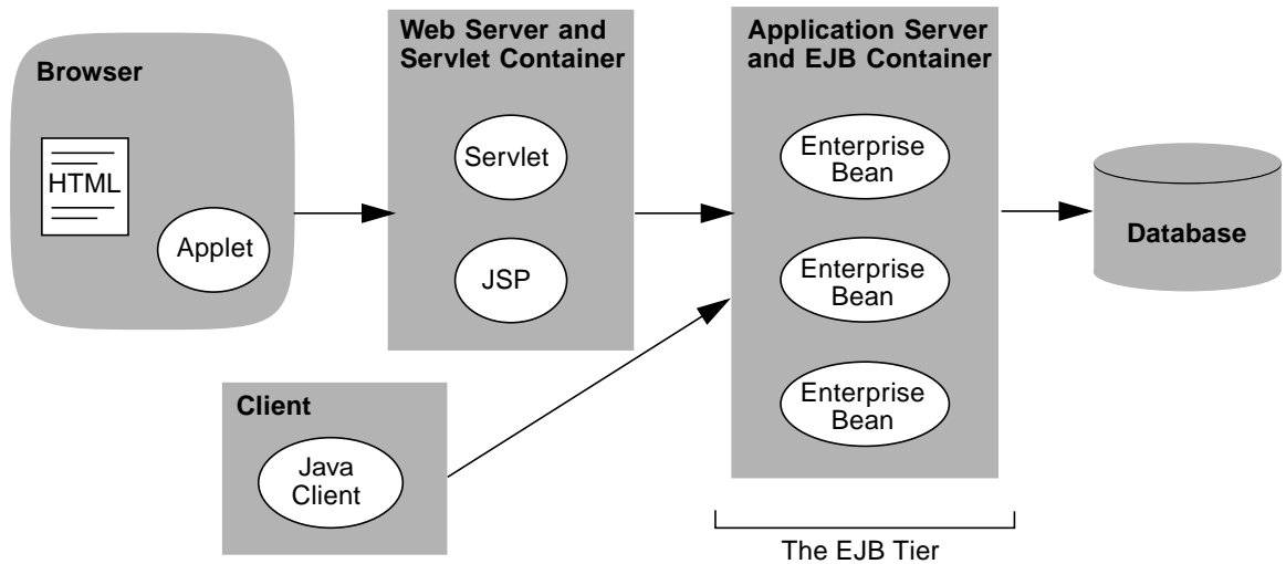
FIGURE 1-1 Model J2EE Application as Supported by the Sun ONE Studio 5 IDE
