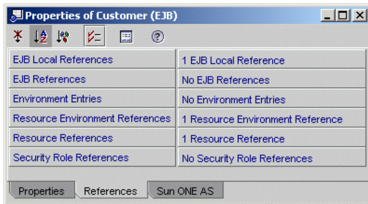
FIGURE 8-1 References Tab of the Properties Dialog Box for a CMP Entity Bean
