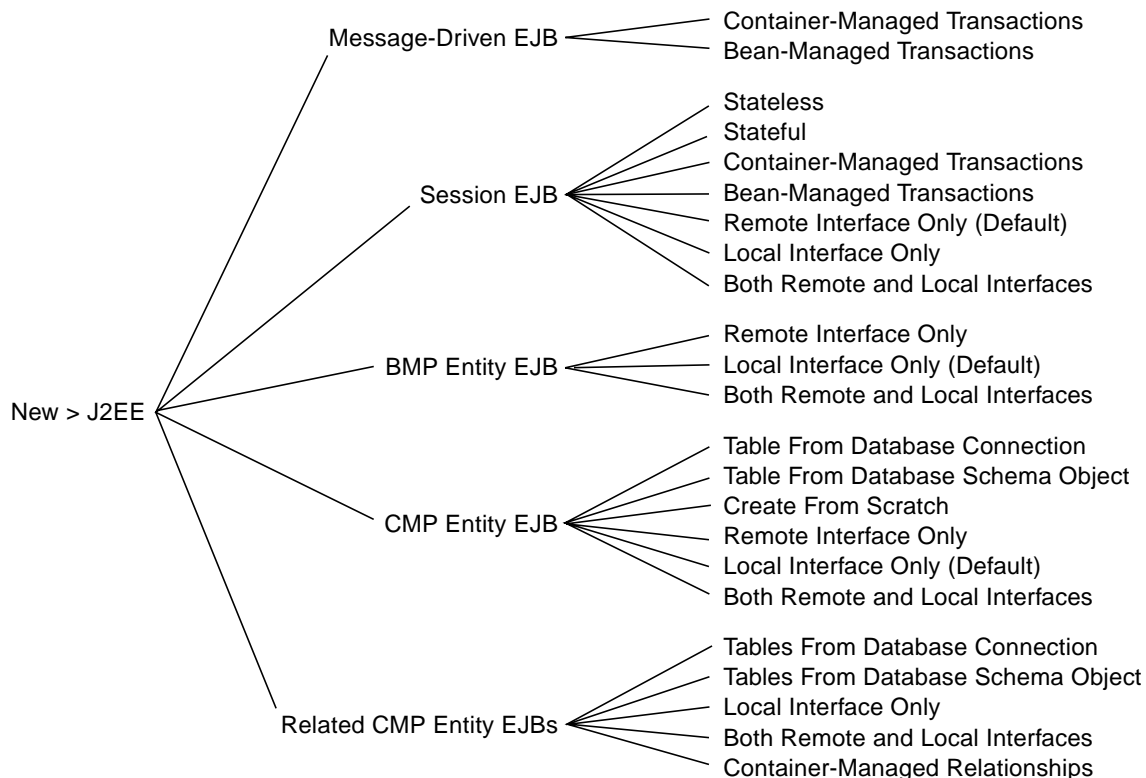
FIGURE 2-1 Basic Choices About Enterprise Beans in the Sun ONE Studio 5 IDE
