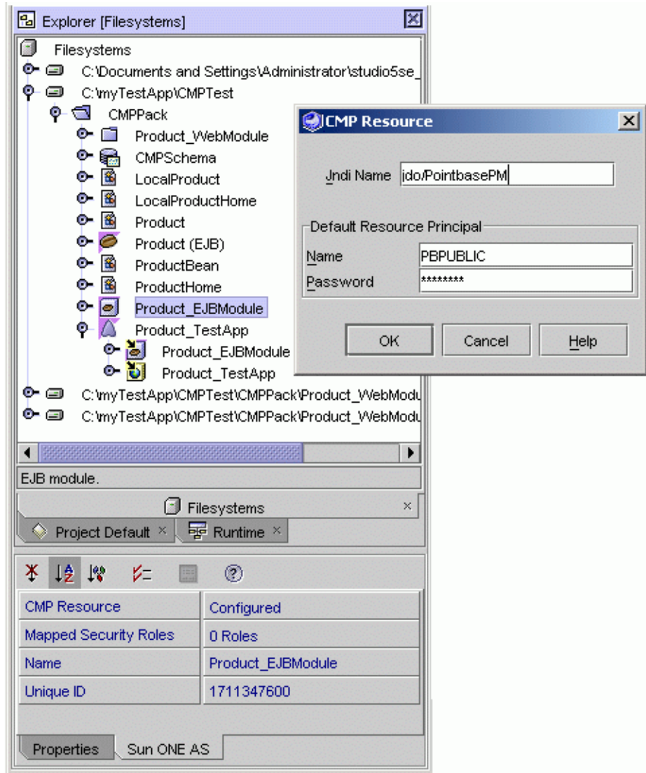
FIGURE 9-4 How to Specify a Database Connection for a CMP Entity Bean
