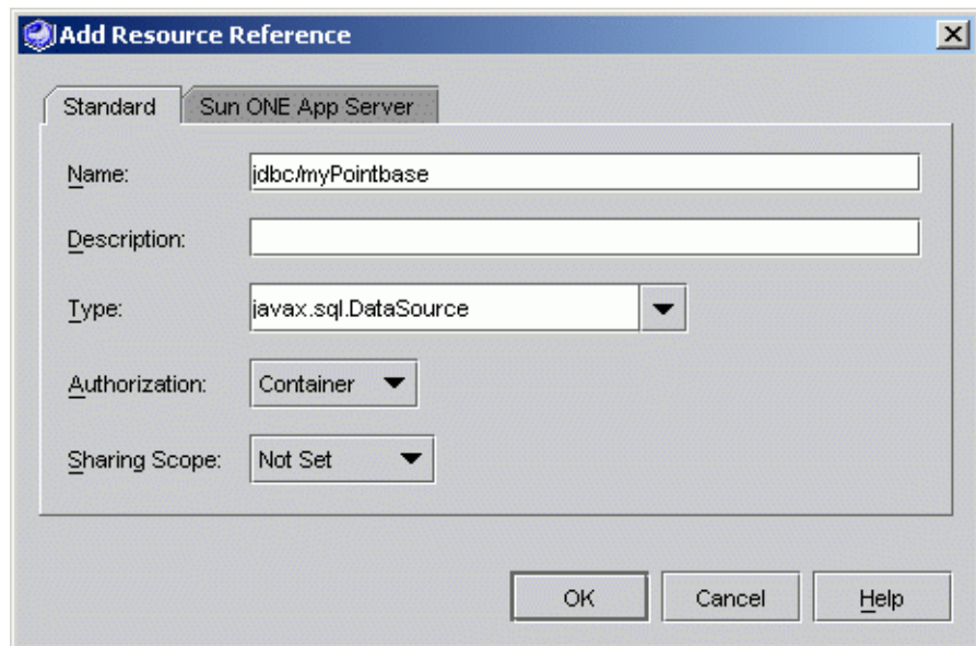
FIGURE 8-2 Standard Tab of the Resource Reference Property Editor for an Entity Bean
