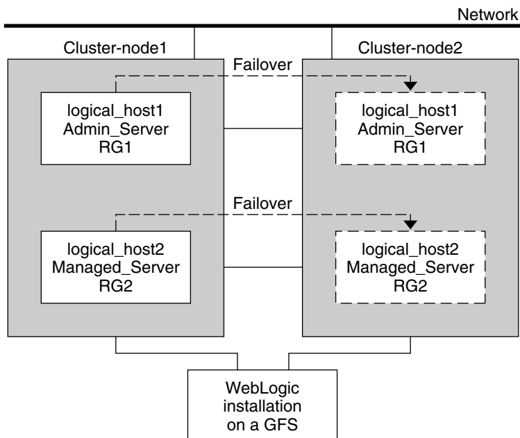
FIGURE 1 Sun Cluster HA for BEA WebLogic Server Simple Configuration
