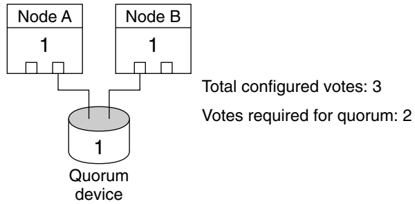
FIGURE 3-2 Two-Node Configuration
