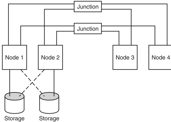
FIGURE 2-3 Pair+N Topology
