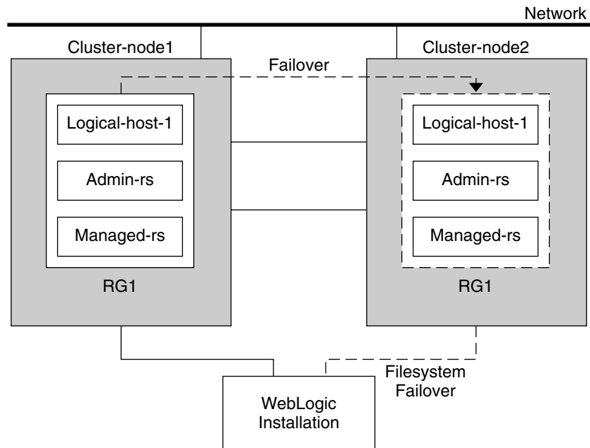
FIGURE 2 Sun Cluster HA for BEA WebLogic Server File System Failover Configuration
