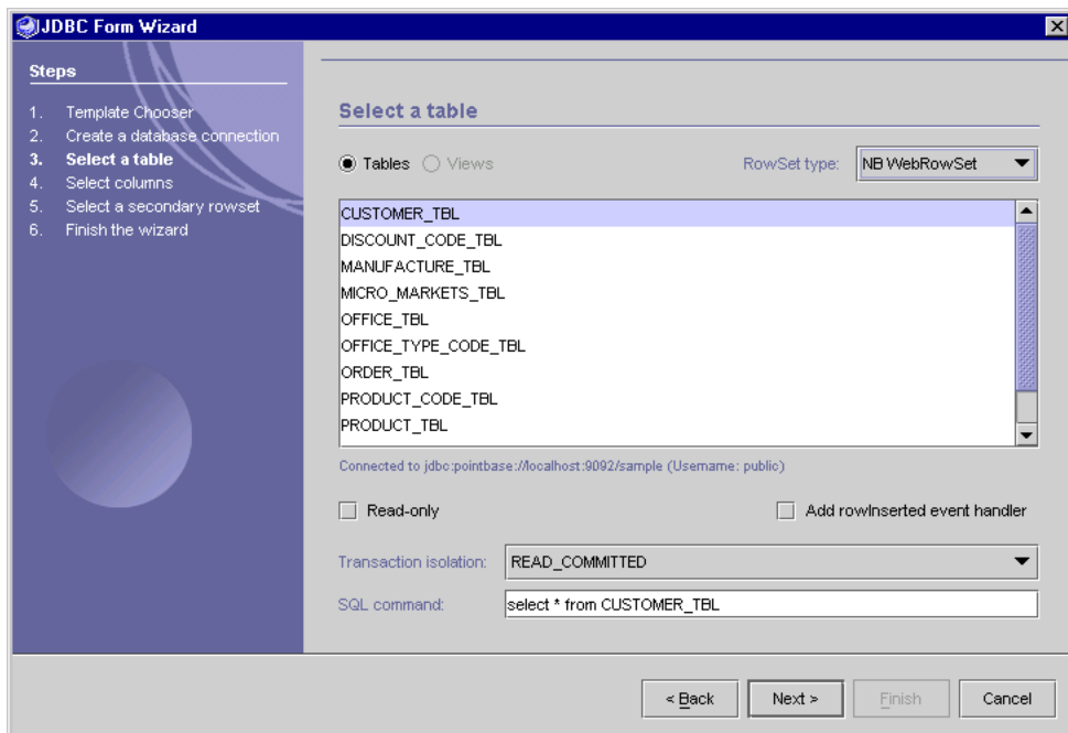
FIGURE 3 JDBC Form Wizard, Select a Table
