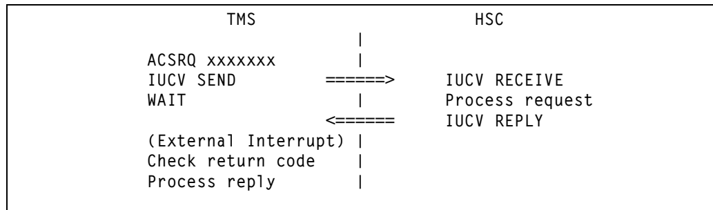
Figure 14. Process flow for the ACSRQ Macro
