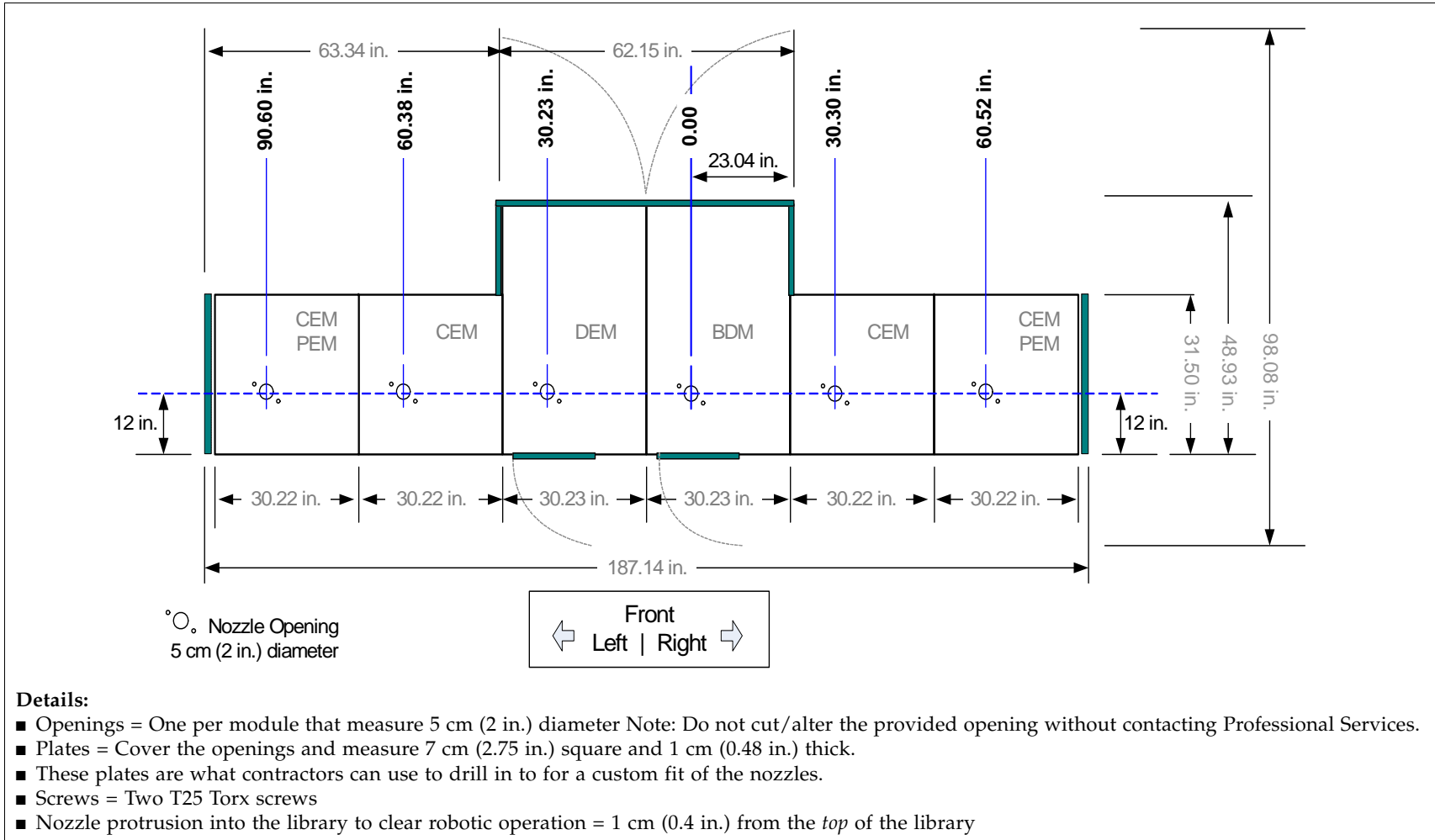
FIGURE 3-6 Fire Suppression Ceiling Access (Viewed from the top of the library)
