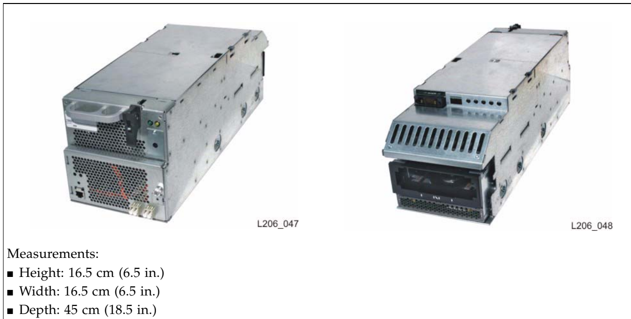
FIGURE 1-11 SL3000 Tape Drive Trays
