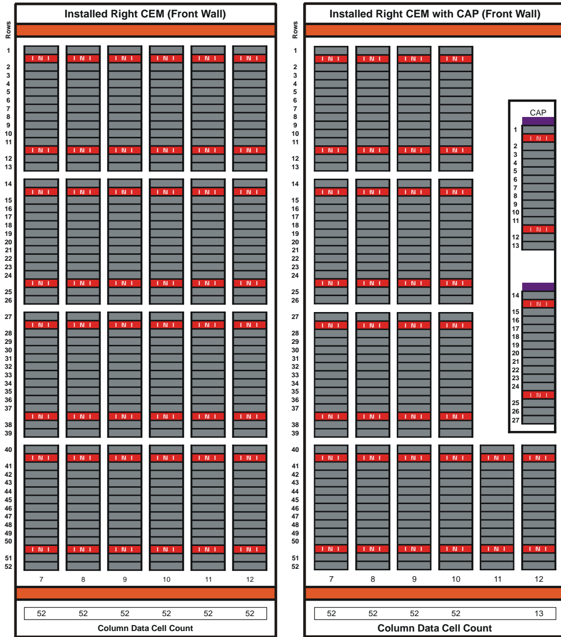
FIGURE A-20 SL3000 Slot Map—Cartridge Expansion Module, Installed on the Right
