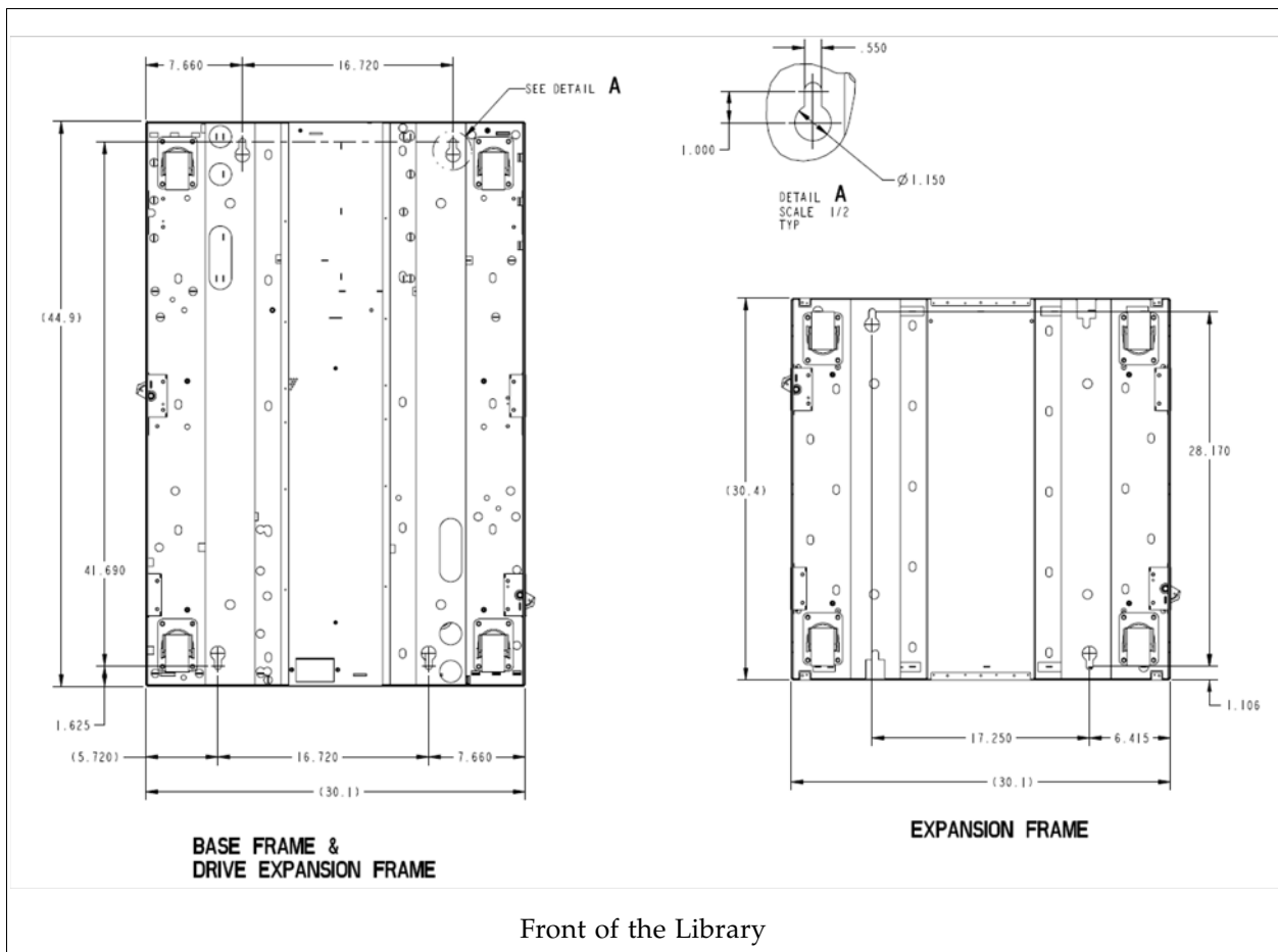
FIGURE 3-10 Seismic Mounting Locations
