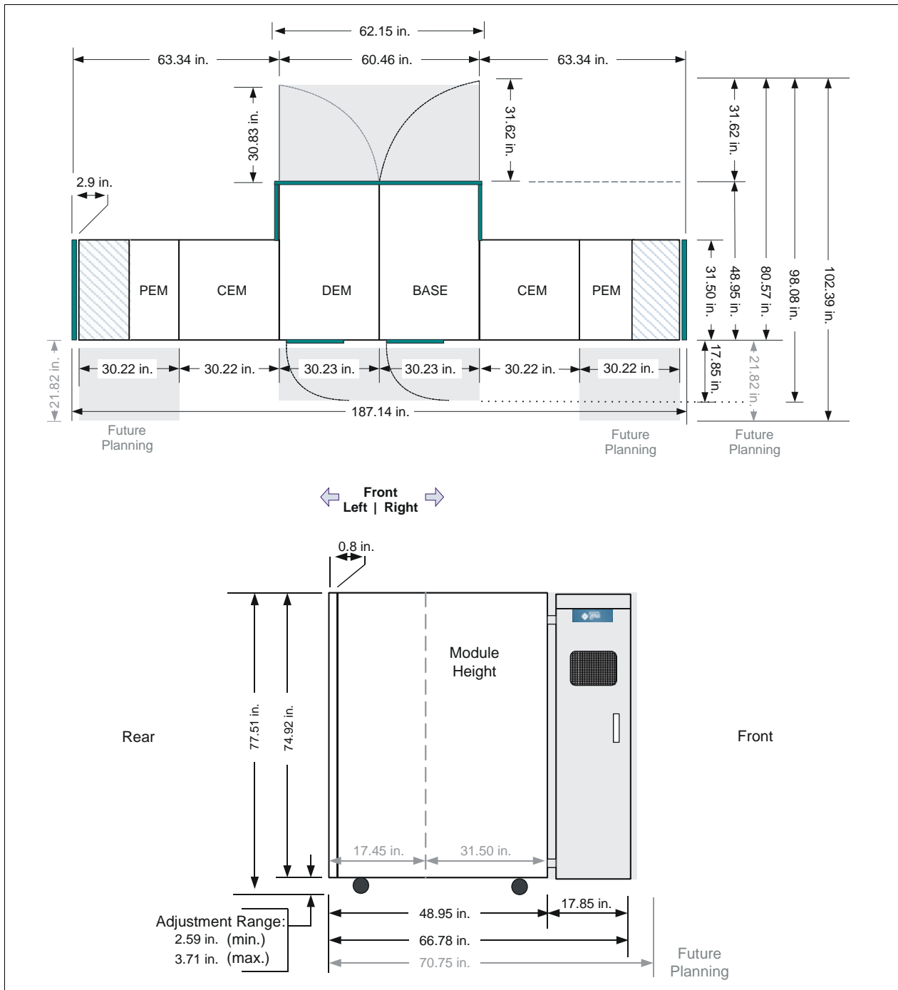
FIGURE 3-3 Standard Dimensions
