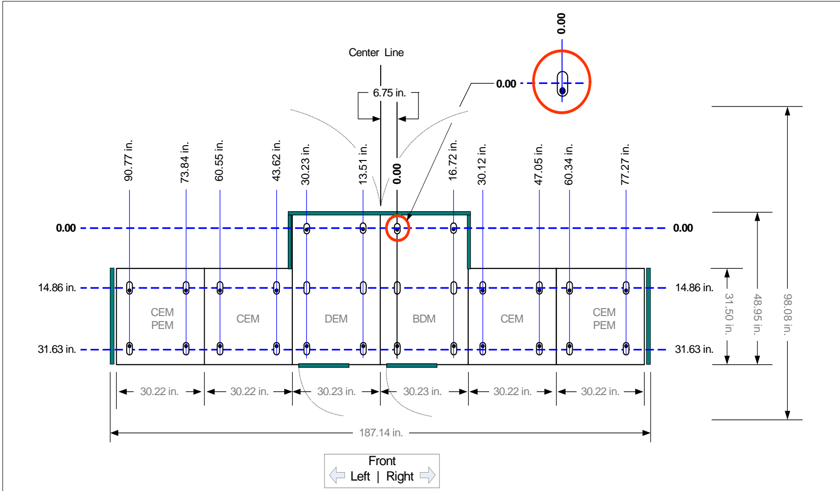
FIGURE 3-5 Floor Loading—Load Pads
