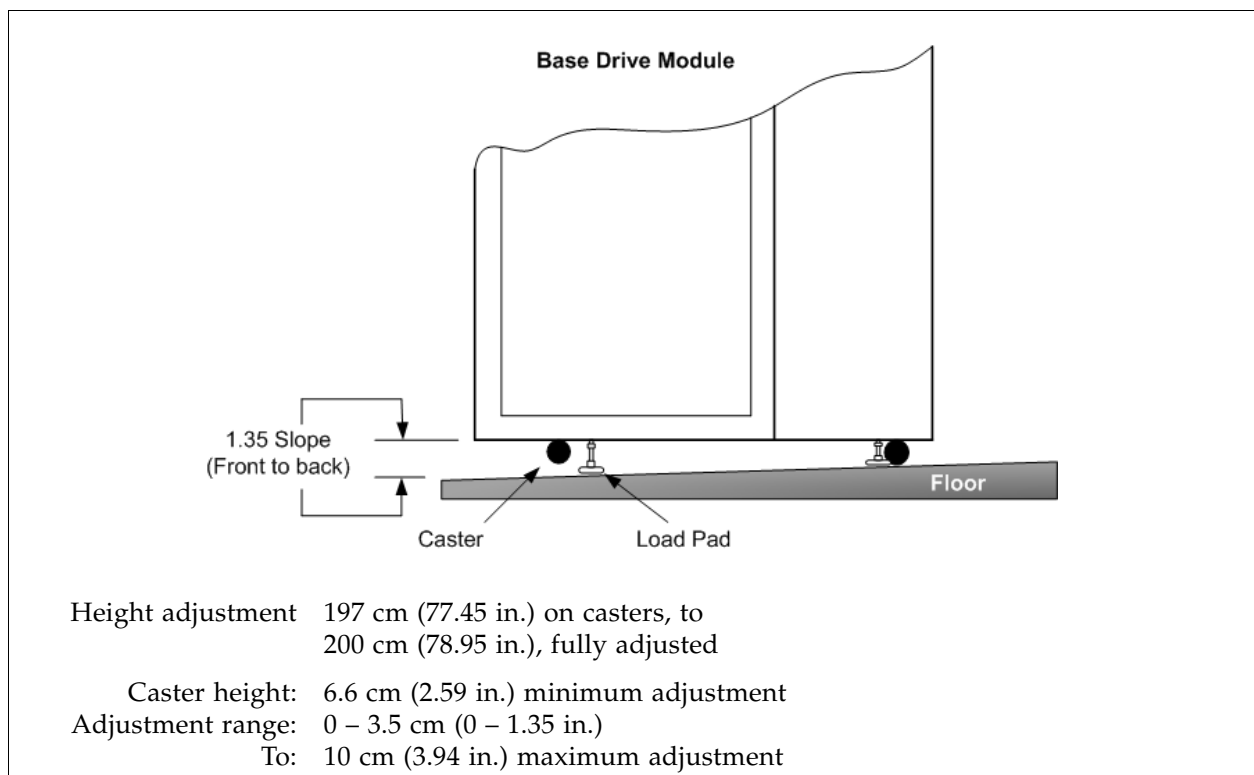
FIGURE 3-8 Floor Slope
