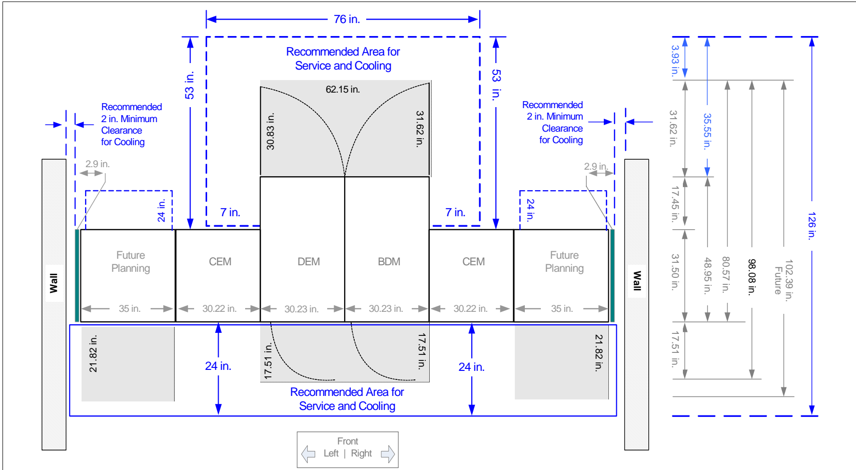
FIGURE 3-4 Service Clearances—Minimum and Recommended
