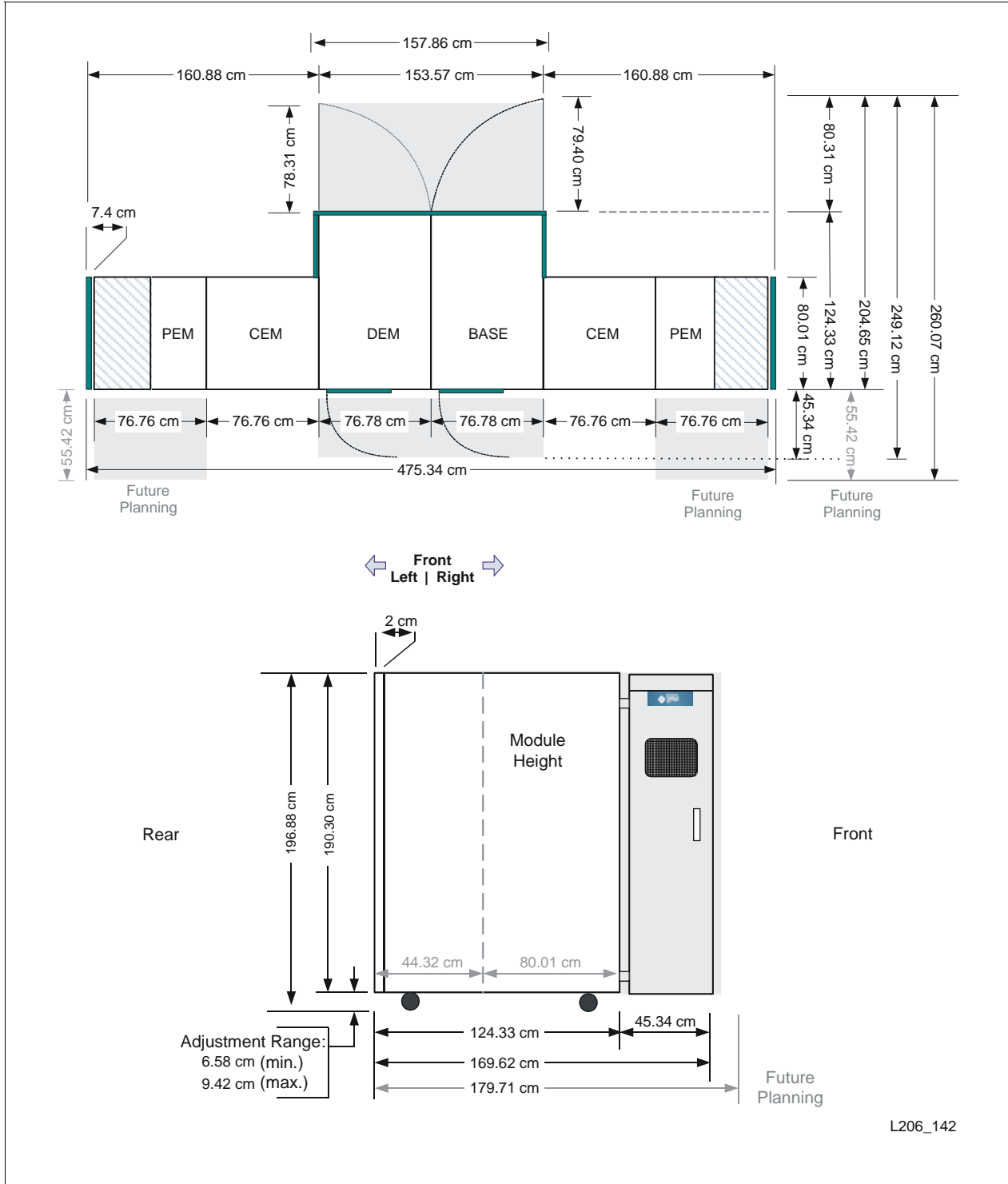
FIGURE 3-2 Metric Dimensions
