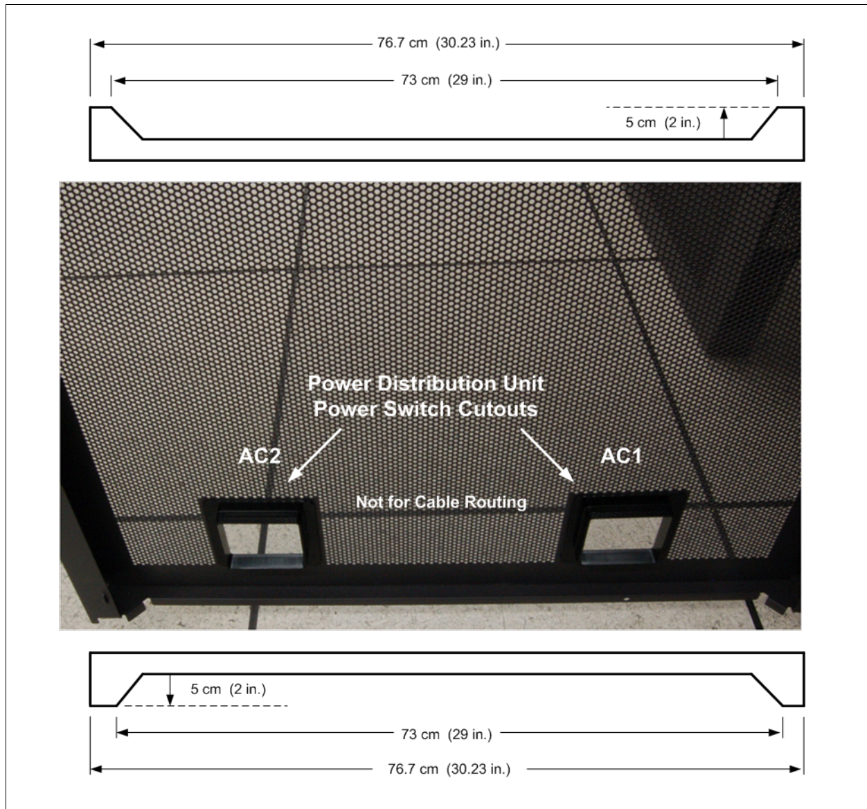
FIGURE 3-9 Cable Routing
