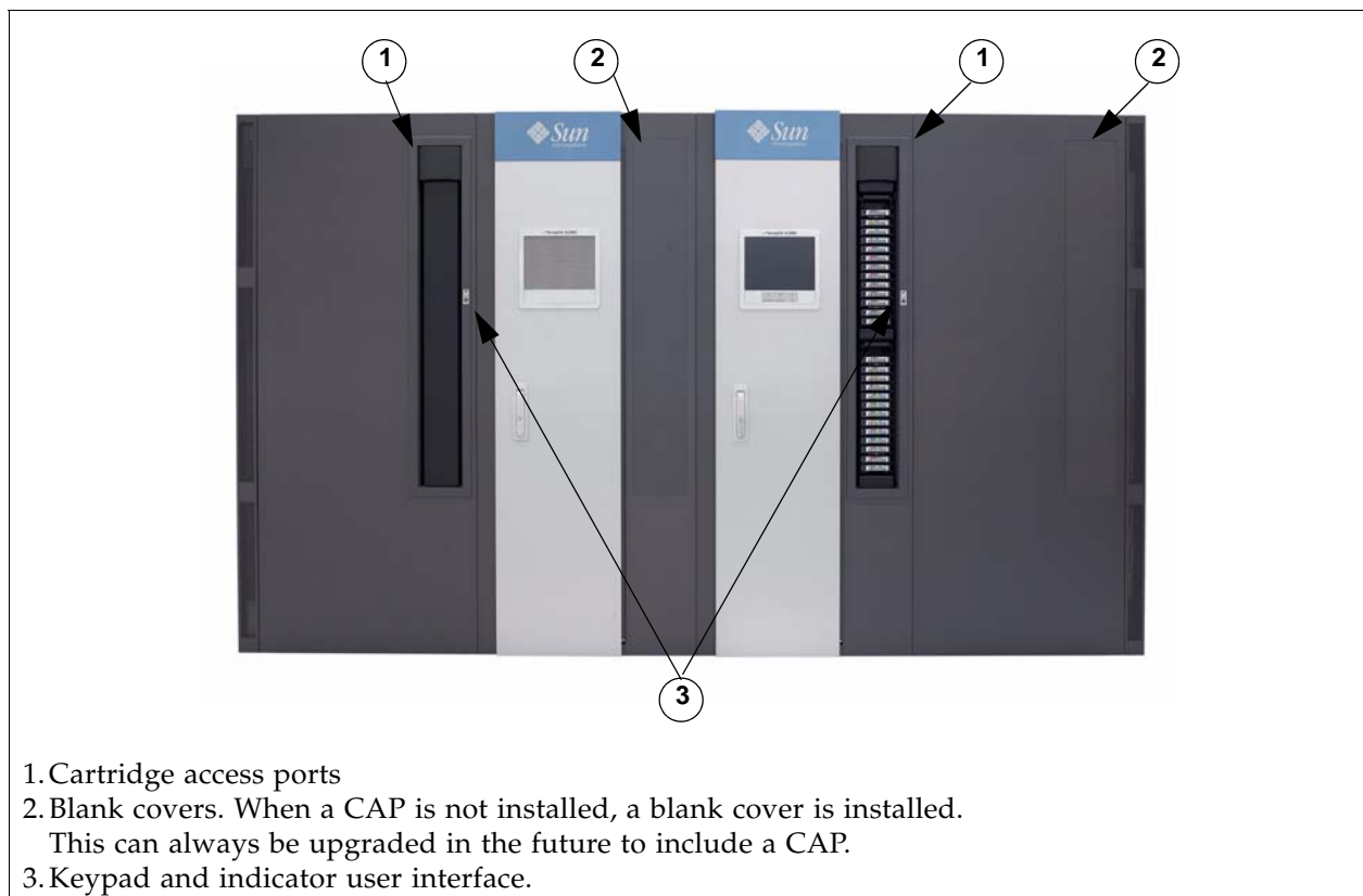
FIGURE 1-10 Cartridge Access Port and Key Pad
