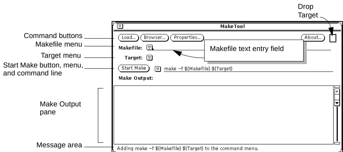
Figure 1-2 MakeTool Base Window
