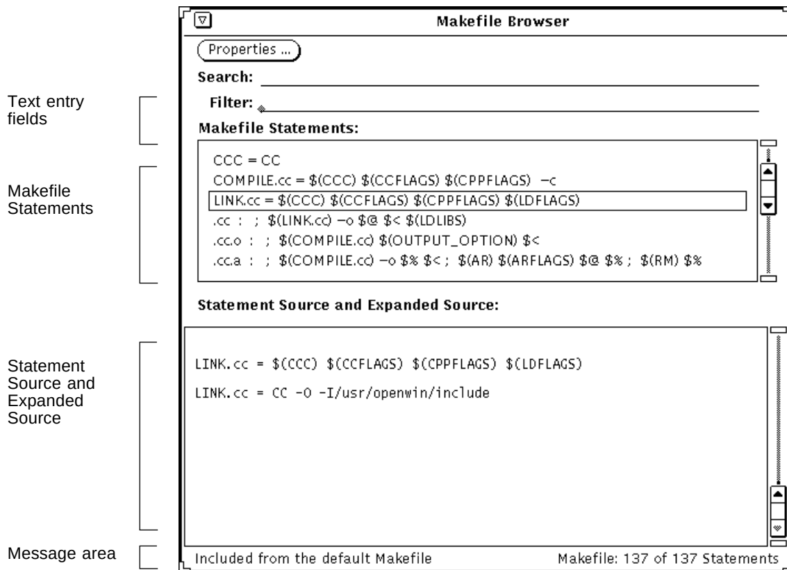
Figure 3-1 Makefile Browser Window
