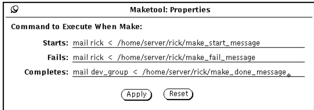
Figure 2-3 MakeTool Properties Window With mail Commands
