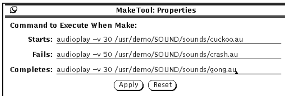
Figure 2-4 MakeTool Properties Window With audioplay Commands
