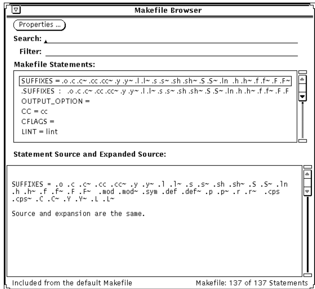
Figure 1-3 Makefile Browser Window
