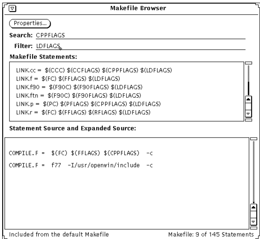
Figure 3-4 Browser Window with LDFLAGS Filter
