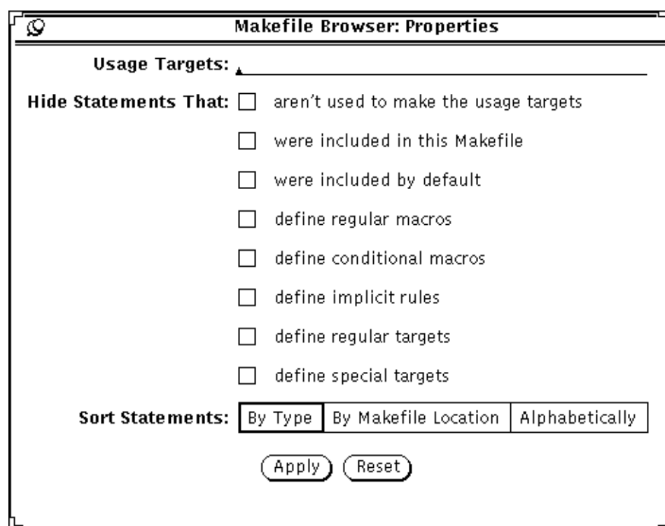
Figure 3-2 Makefile Browser Properties Window
