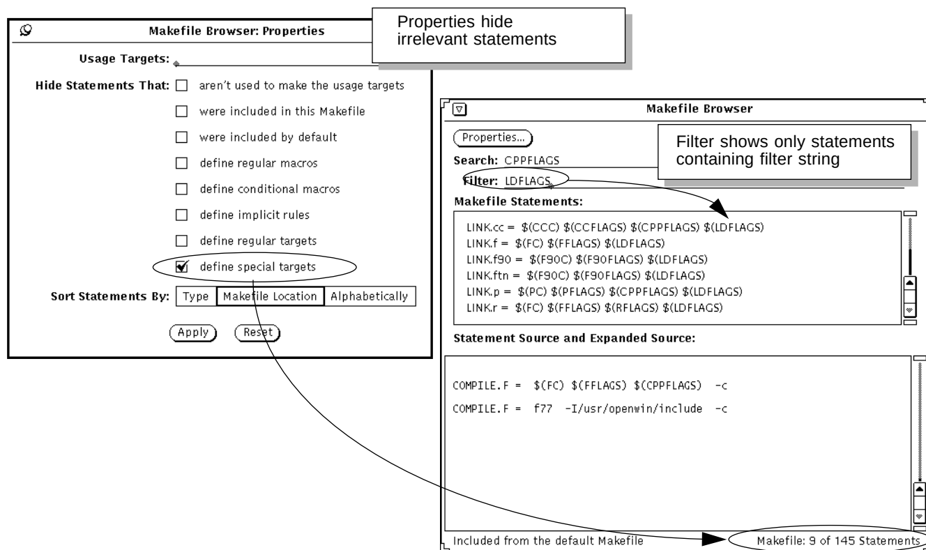
Figure 3-5 Setting Properties to Hide Statements
