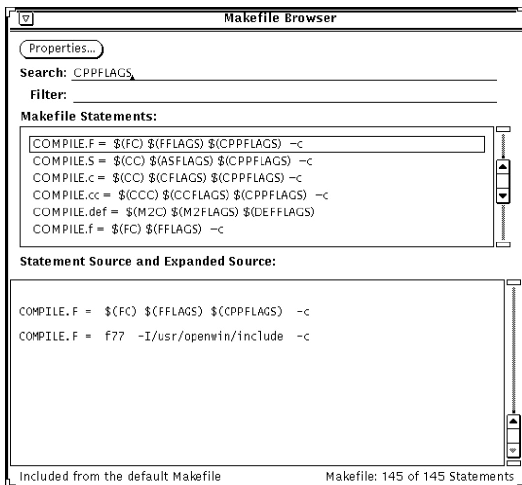
Figure 3-3 Makefile Browser Window with CPPFLAGS Search String
