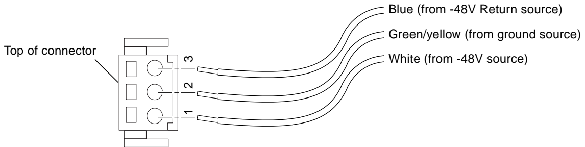
FIGURE 2-8 Assembling the DC Input Power Cable
