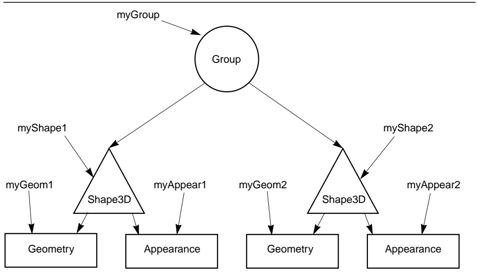
Figure 2-1 A Simple Scene Graph
