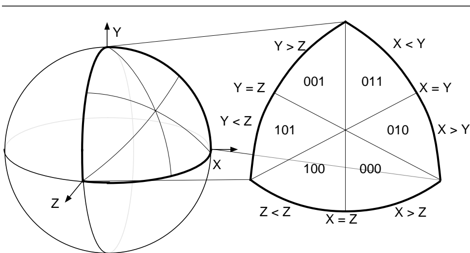
Figure B-3 Encoding of the Six Sextants of Each Octant of a Sphere
