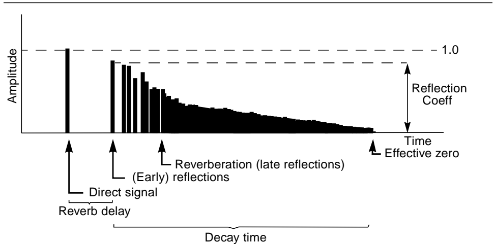
Figure 8-2 Sound Reverberation Parameters
