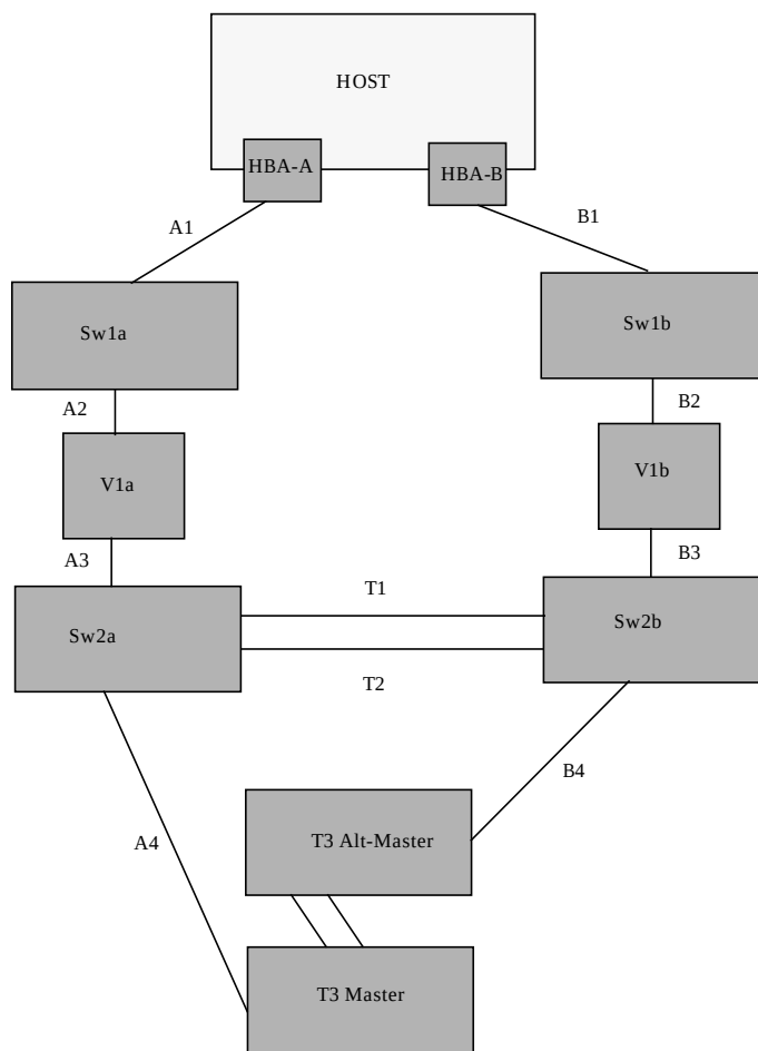
FIGURE 2-2 Sun StorEdge 6900 Series Fibre Channel Link Diagram
