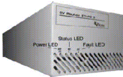
FIGURE 7-1 Virtualization Engine Front Panel LEDs
