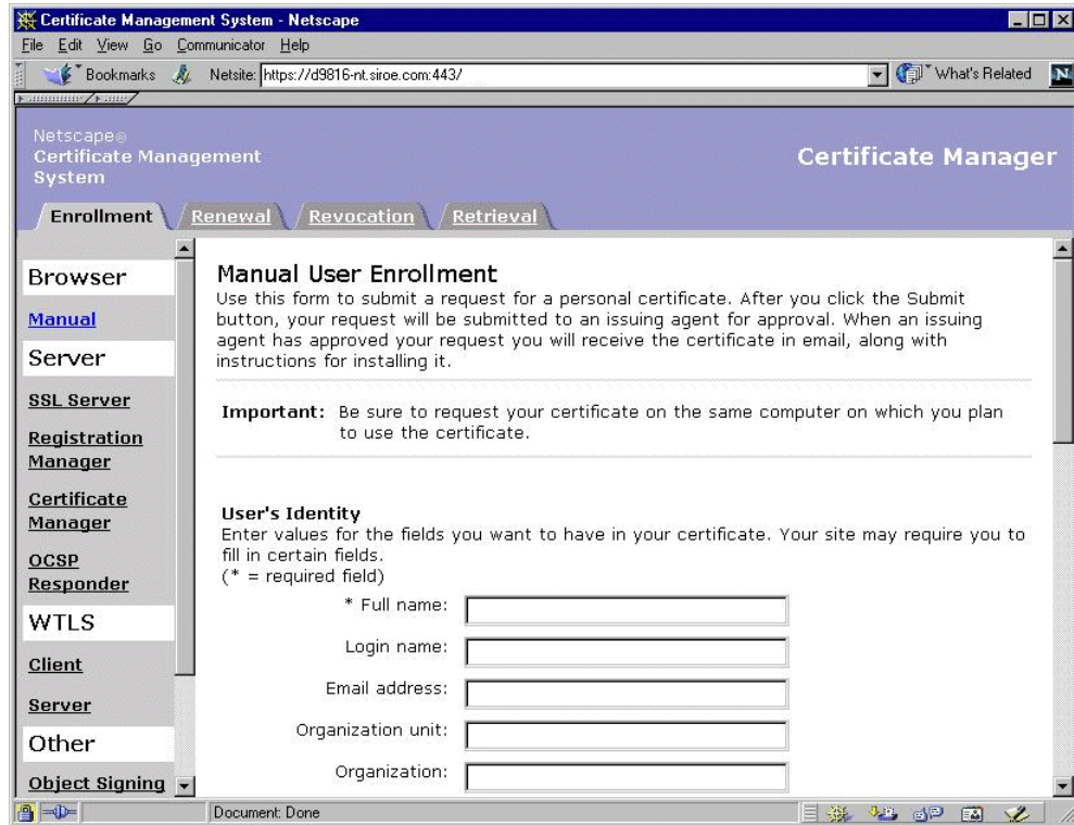
Figure 2-1 End-entity services interface
