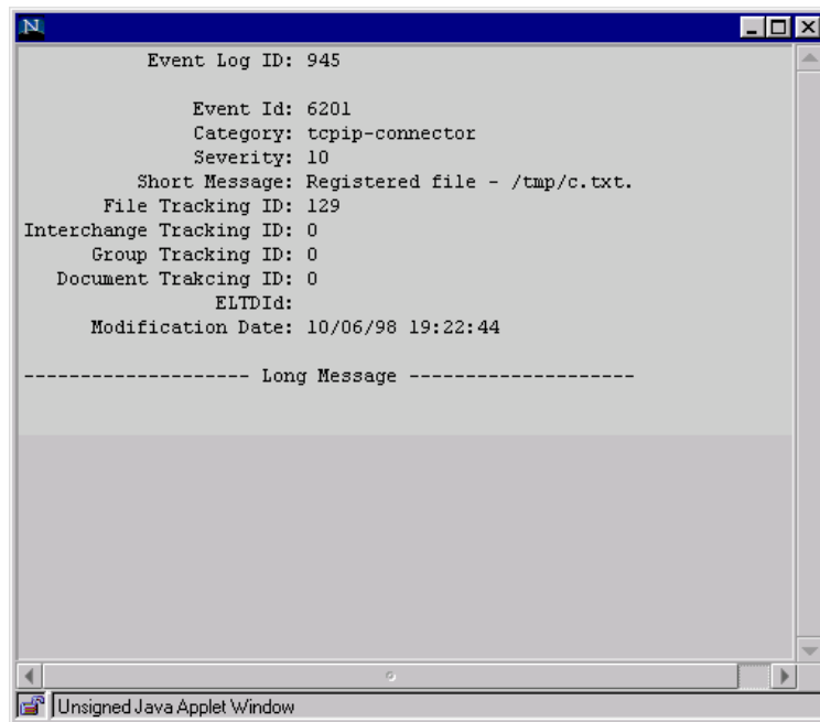
Figure 7-30 Detailed information for a selected EventLog entry
