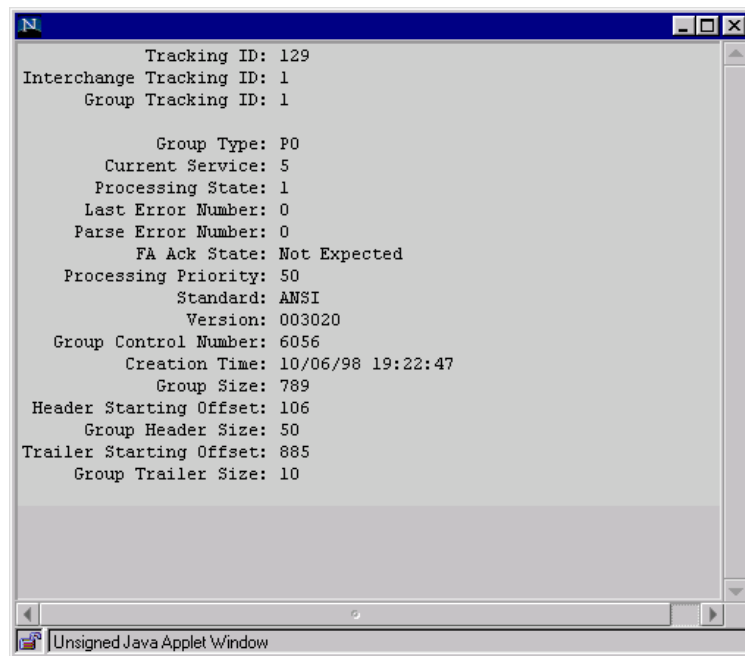
Figure 7-20 Detailed information for a selected group
