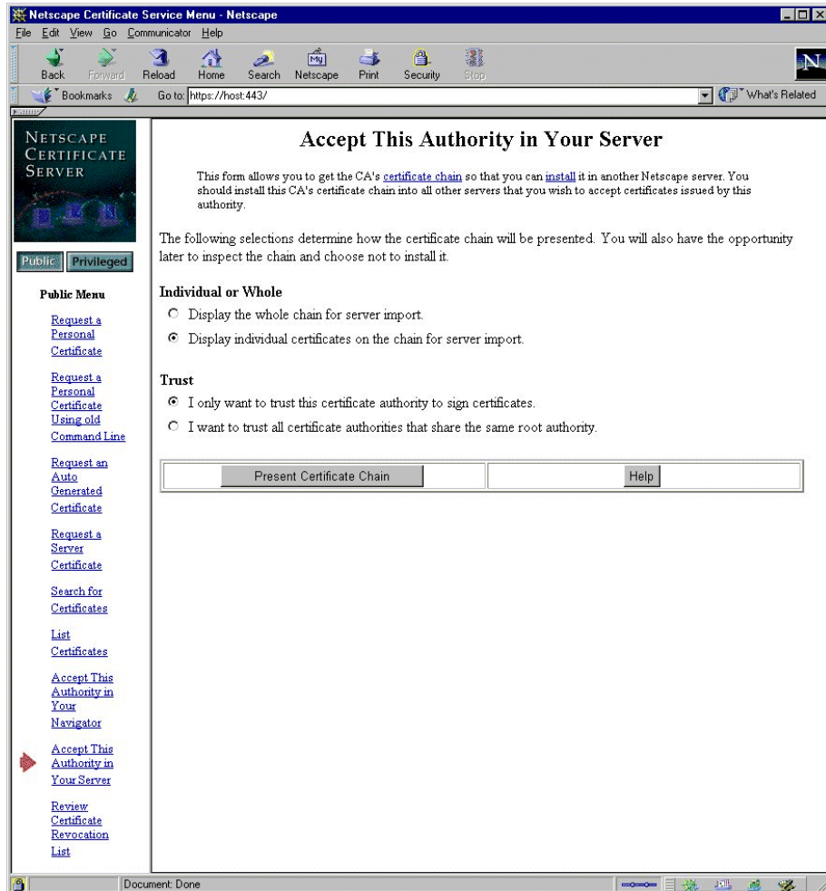
Figure 9-3 iPlanet Certificate Server, Trust option selected
