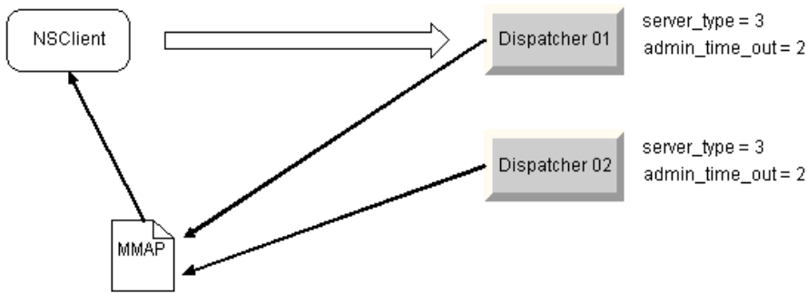
Figure C-2 ECXpert process model
