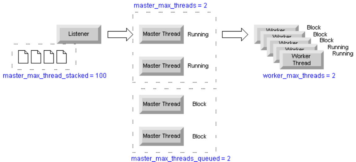
Figure C-1 ECXpert threading model
