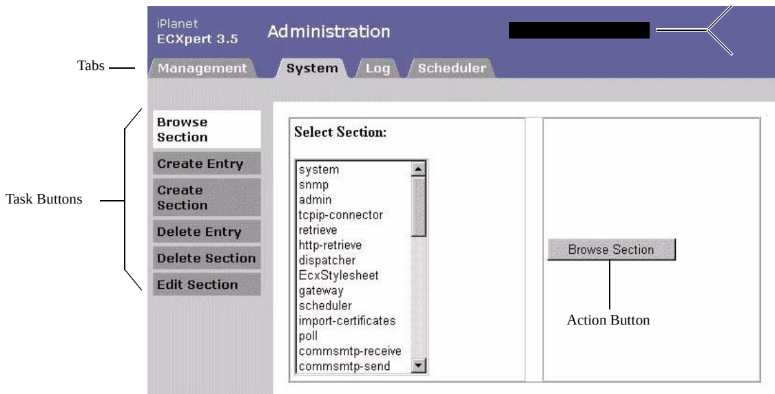
Figure 3-4 Basic layout of ECXpert System Administration Interface screens
