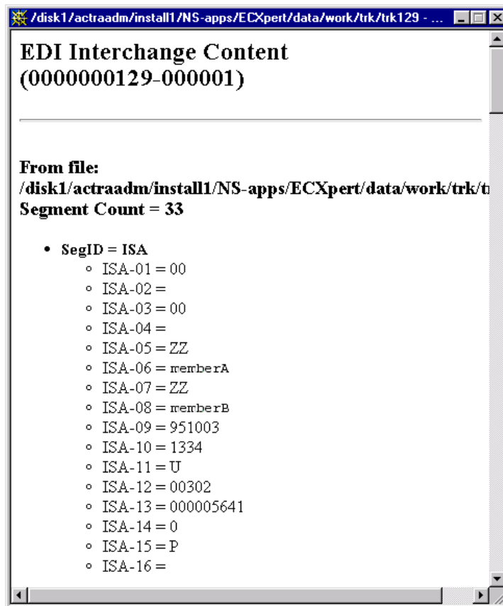
Figure 7-16 EDI data for a selected interchange
