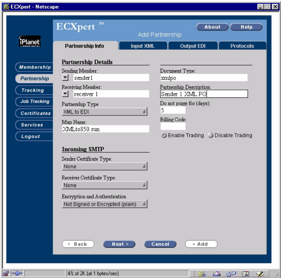
Figure 2-2 Specifying the Partnership Details
