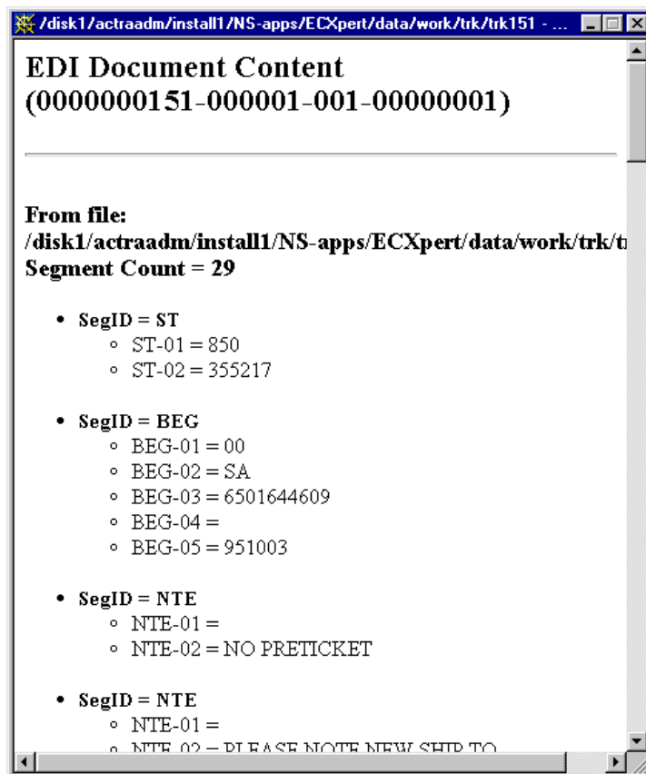
Figure 7-26 EDI data for a selected document
