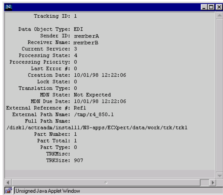
Figure 7-10 Detailed information for a selected file
