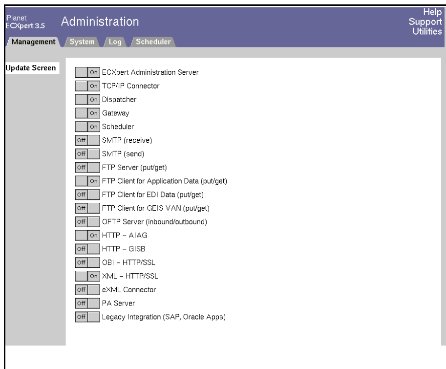
Figure H-3 ECXpert Administrative Interface, Server Management tab
