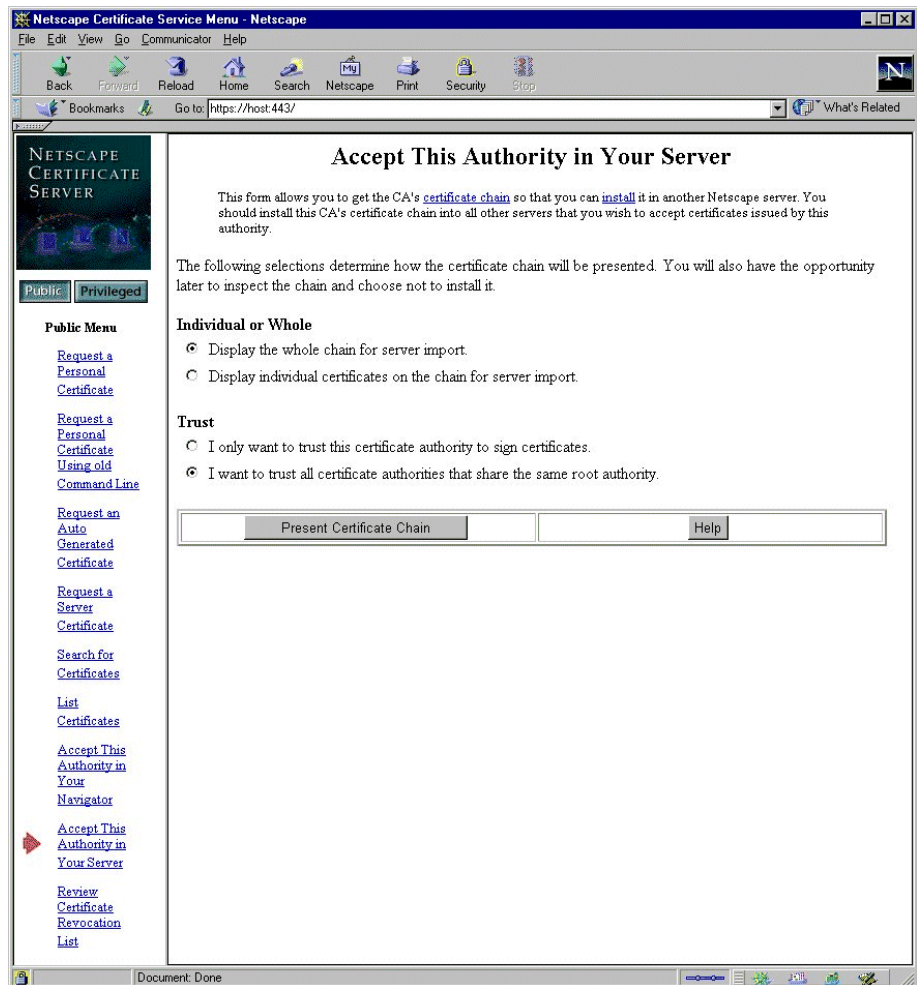
Figure 9-2 iPlanet Certificate Server, Accept This Authority... option selected
