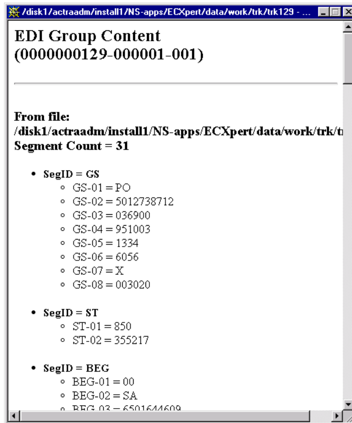
Figure 7-21 EDI data for a selected group
