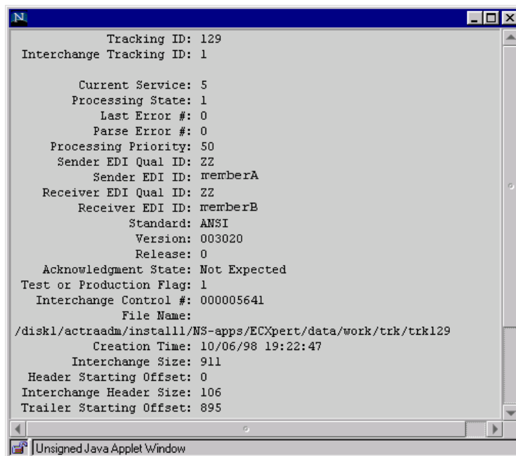
Figure 7-15 Detailed information for a selected interchange
