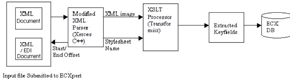
Figure 2-1 XML Parsing Logic
