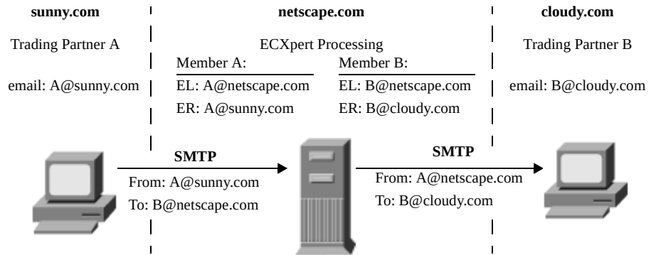
Figure 6-1 ECXpert SMTP to SMTP transaction flow
