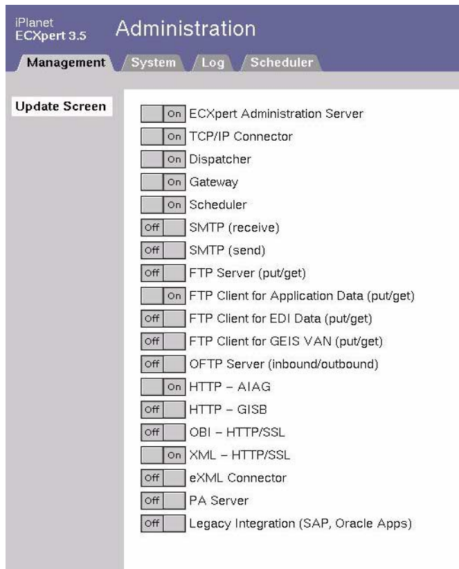
Figure 3-6 Management tab, Administrative Server ON
