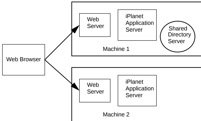
Figure 2-1 A simple iPlanet Application Server cluster configuration
