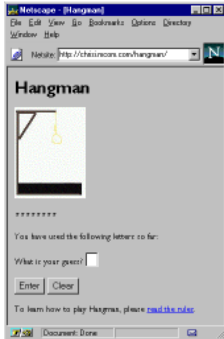
Figure 4-2 Hangman
