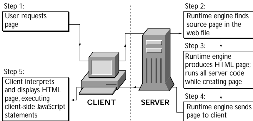
Figure 5-1 Processing a JavaScript page request
