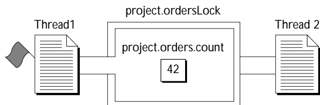
Figure 6-5 Thread 2 waits while thread 1 has the lock
