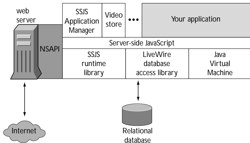
Figure 2-2 Server-side JavaScript in the iPlanet server environment
