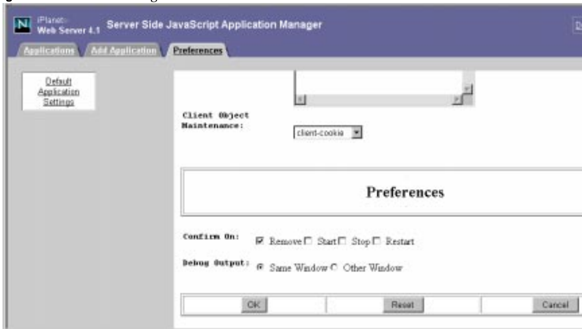
Figure 3-7 Default Settings form with Preferences shown
