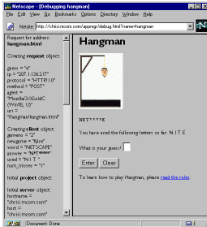
Figure 3-5 Debugging Hangman
