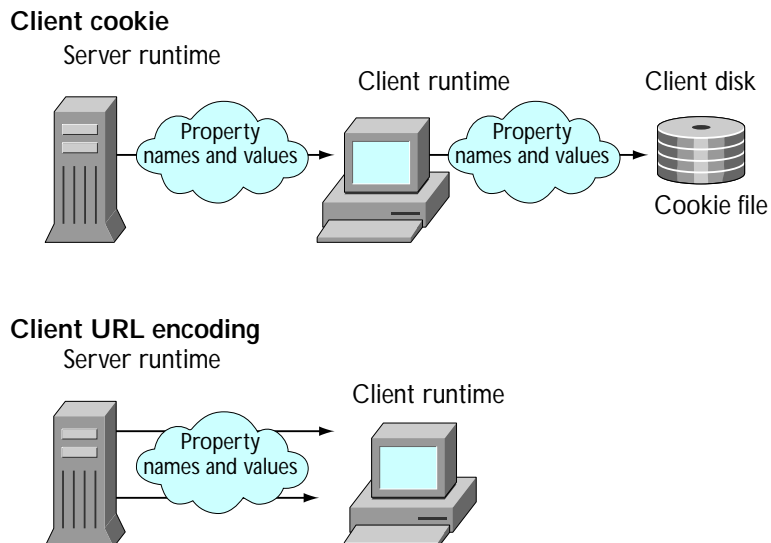
Figure 6-3 Client-side techniques
