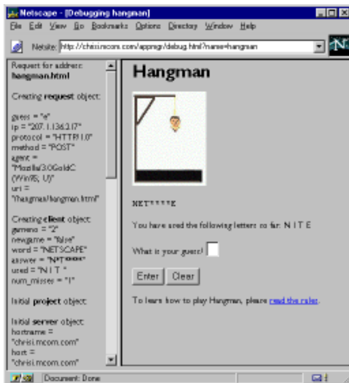
Figure 4-3 Debugging Hangman
