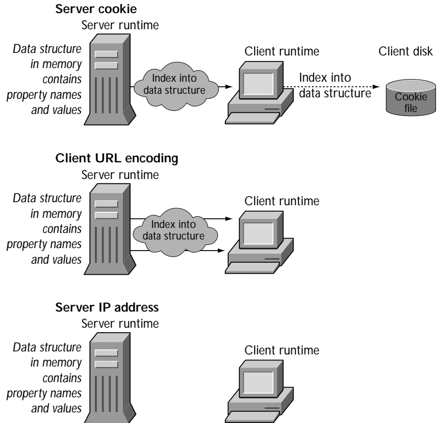
Figure 6-4 Server-side techniques
