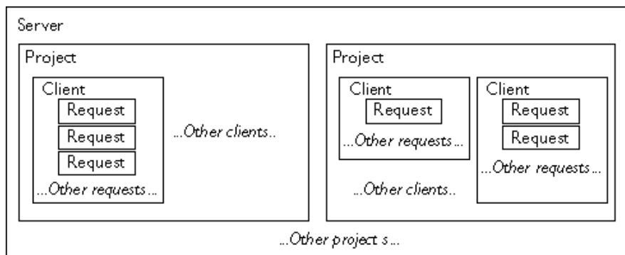
Figure 6-1 Relative availability of session-management objects
