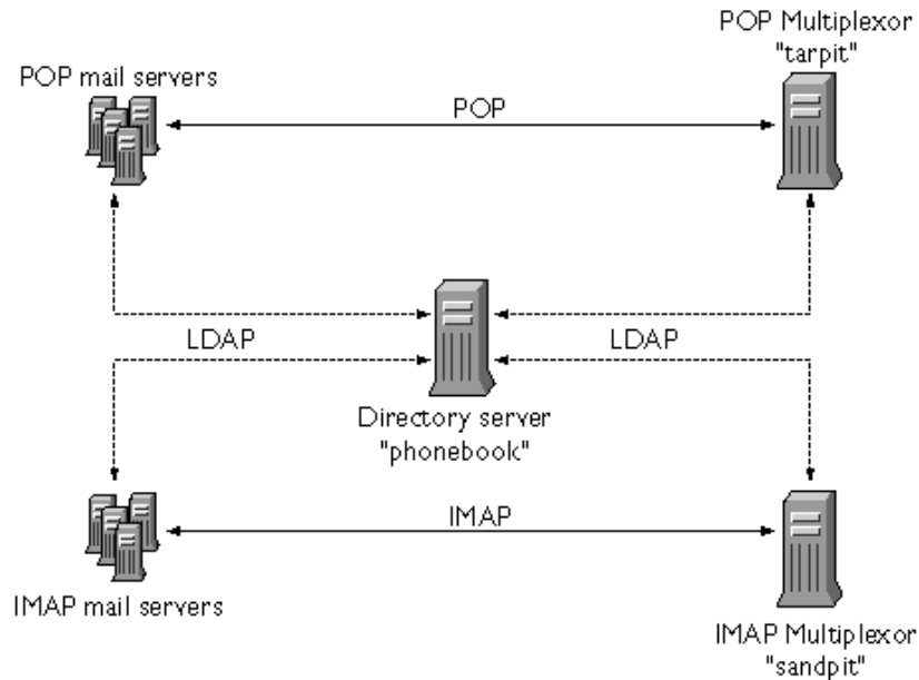
Figure 5-3 Multiple MMPs Supporting Multiple Messaging Servers
