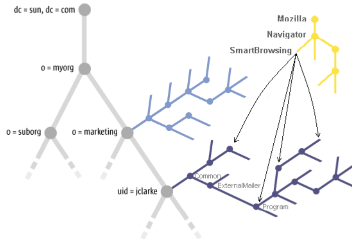
FIGURE 5-1 “Tree of trees”
