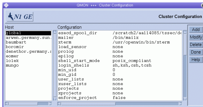
FIGURE 1-6 Cluster Configuration Dialog Box
