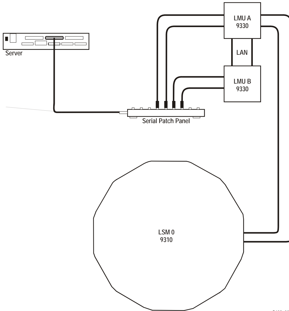
FIGURE 7-4 ACSLS Server in Dual-LMU Configuration
