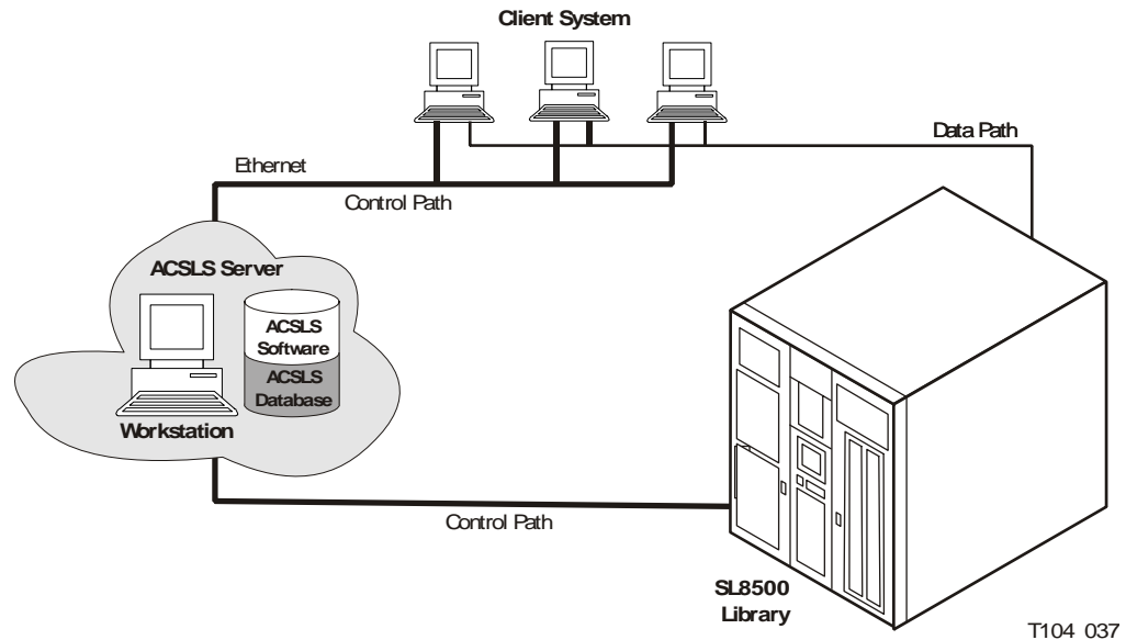
FIGURE B-1 SL8500 and an ACSLS Server
