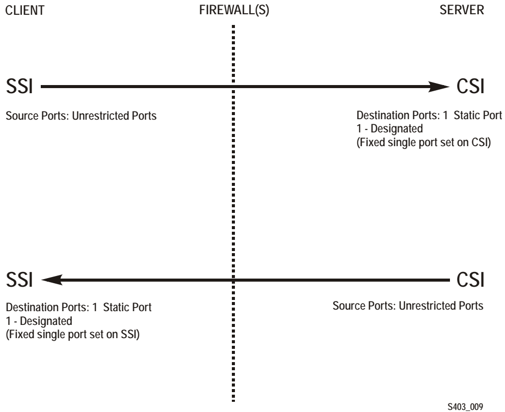
FIGURE J-1 Firewall Security on Client (SSI) and SCALS Server (CSI) without the Portmapper Feature
