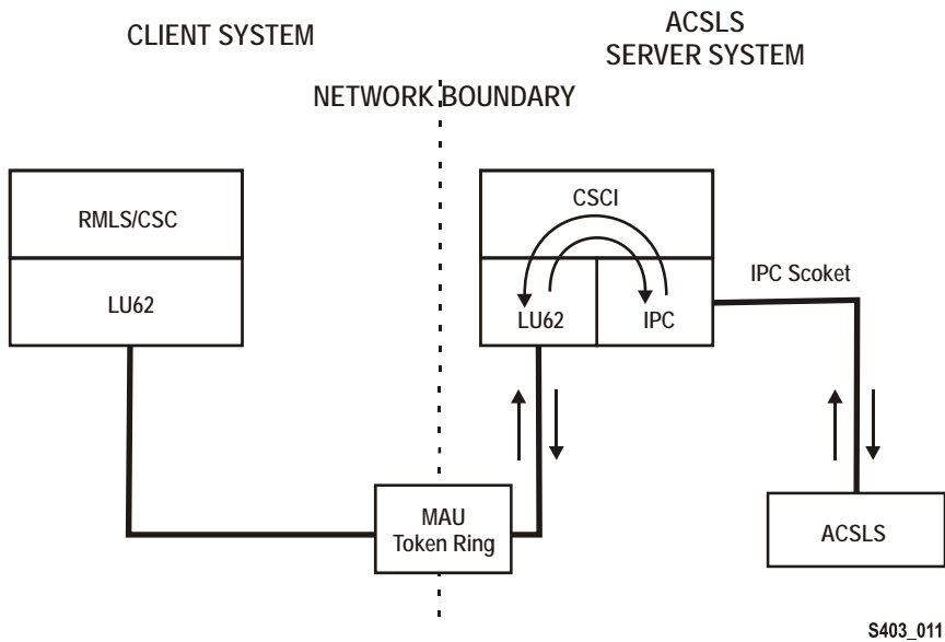
FIGURE L-2 CSCI System with Token Ring Interface
