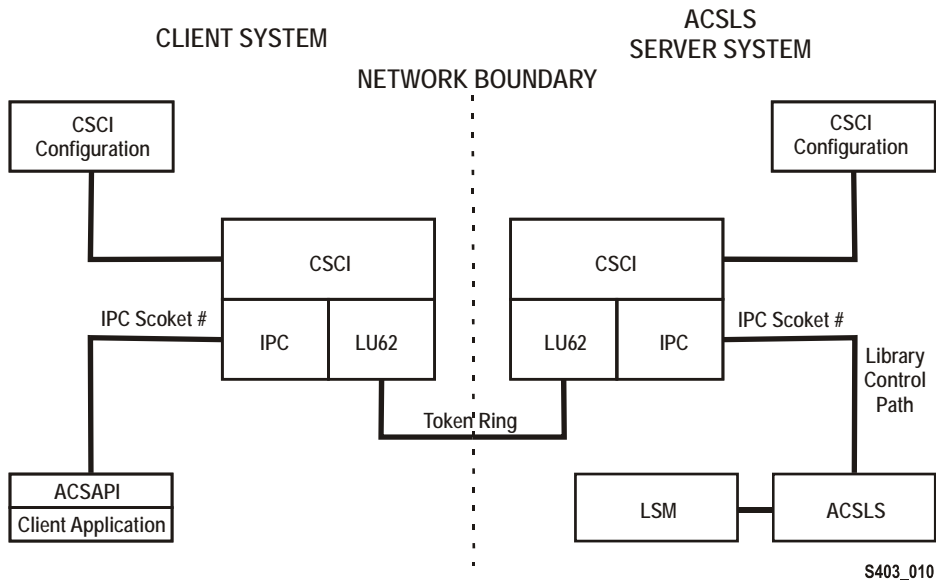
FIGURE L-1 CSCI Architecture and Subsystems
