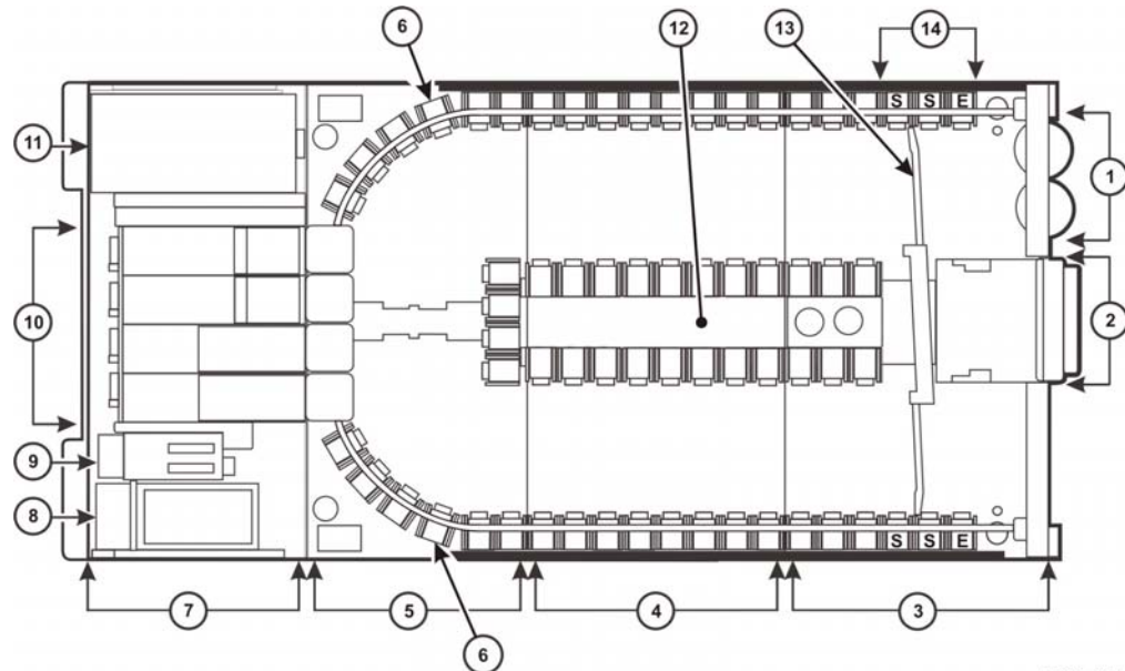
FIGURE B-2 SL8500 Customer Expansion Module
