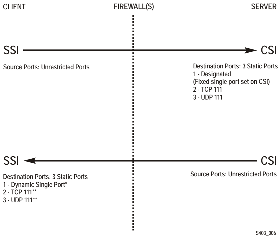
FIGURE 0-1 Firewall security on ACSLS server side (CSI) only
