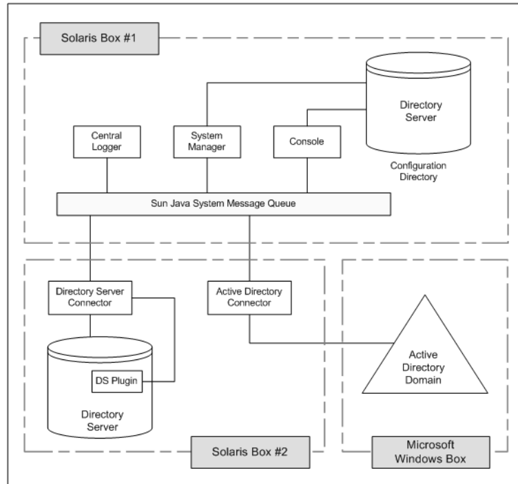
FIGURE 1-2 Directory Server and Active Directory Component Distribution
