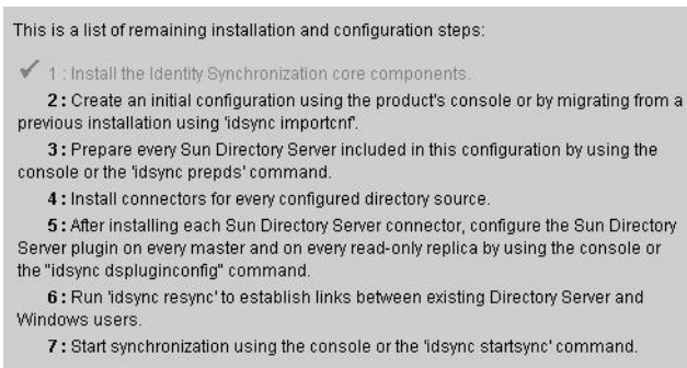
FIGURE 3-7 To Do List for Identity Synchronization for Windows Installation and Configuration
