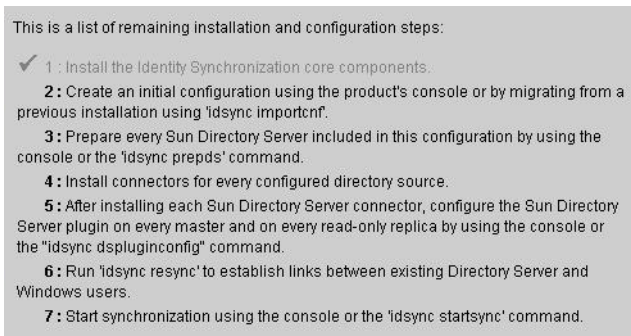
FIGURE 2-2 To Do List for Identity Synchronization for Windows Installation and Configuration
