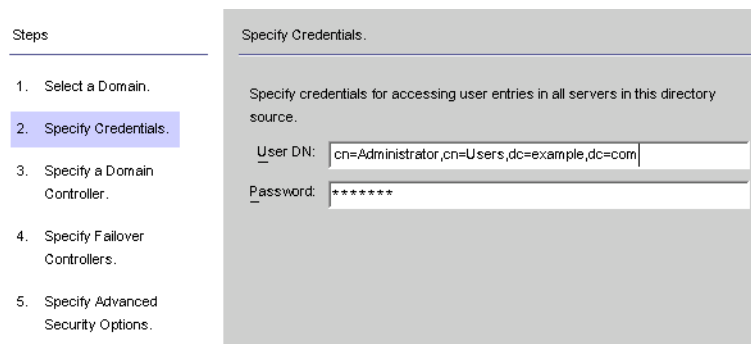
FIGURE 4-19 Specifying Credentials for This Active Directory Source
