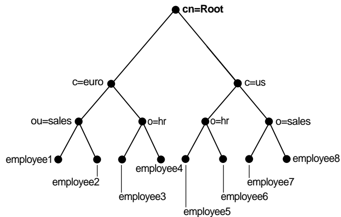
Figure 17–1 Example of a Directory Information Tree
