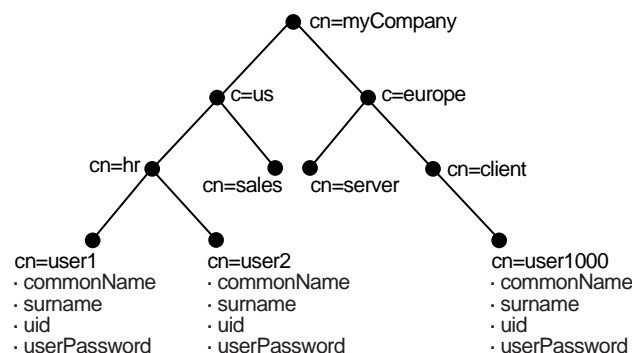
Figure 37-1 A Sample Naming Context
