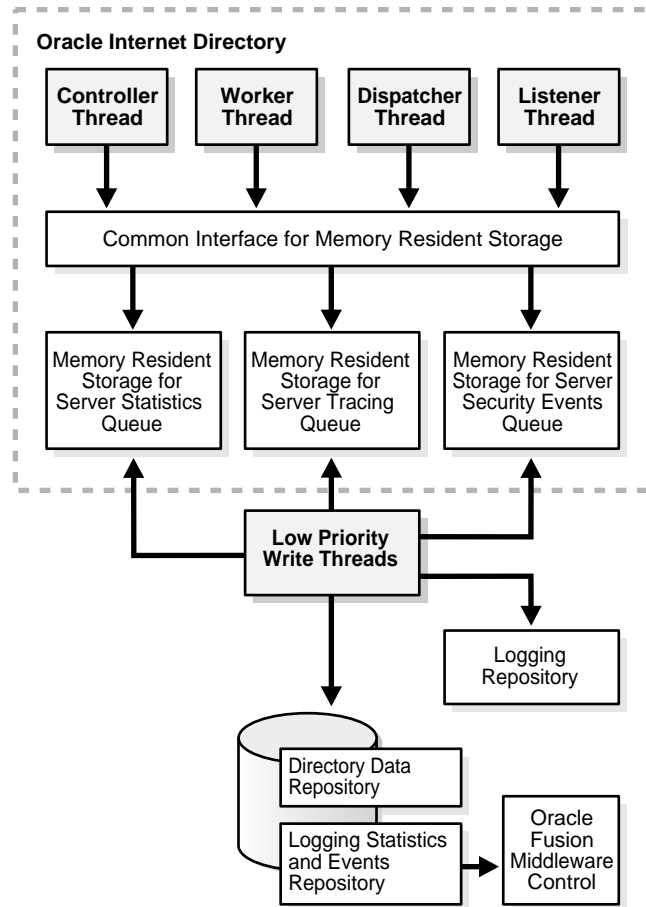
Figure 23–1 Architecture of Oracle Internet Directory Server Manageability
