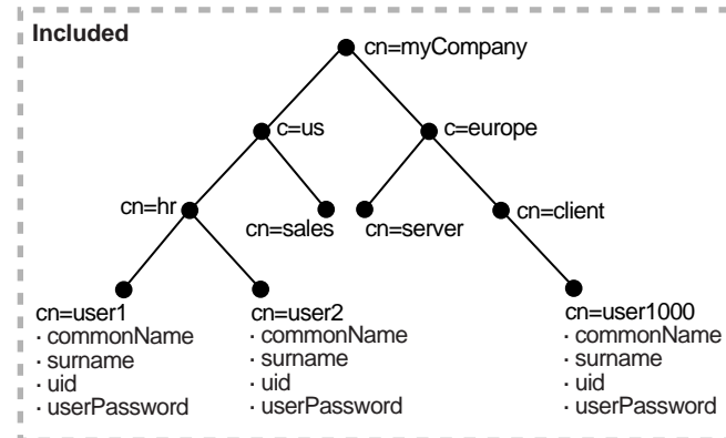
Figure 37-2 Naming Context Object #1
