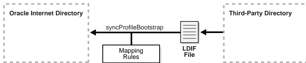
Figure 35–3 Using an LDIF File and syncProfileBootstrap
