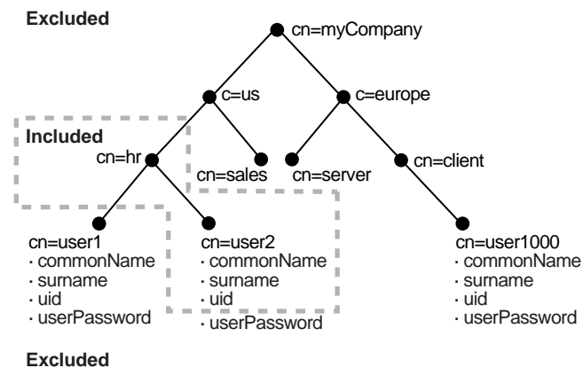
Figure 37-6 Naming Context Object #4
