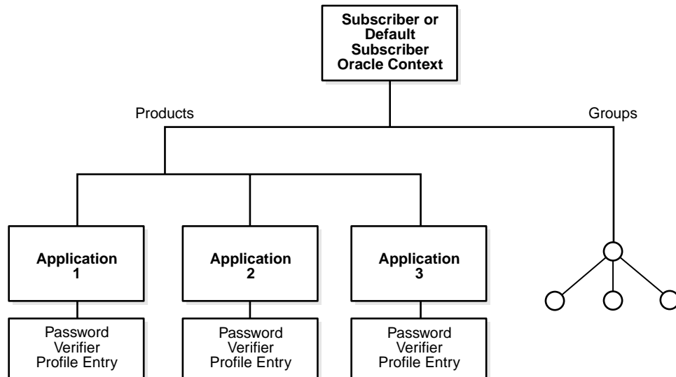
Figure 29–1 Location of the Password Verifier Profile Entry
