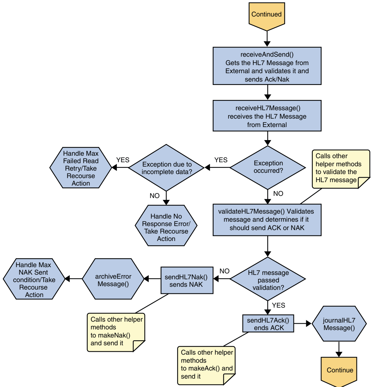
FIGURE 10 Inbound HL7 V2 Collaboration - Part 2
