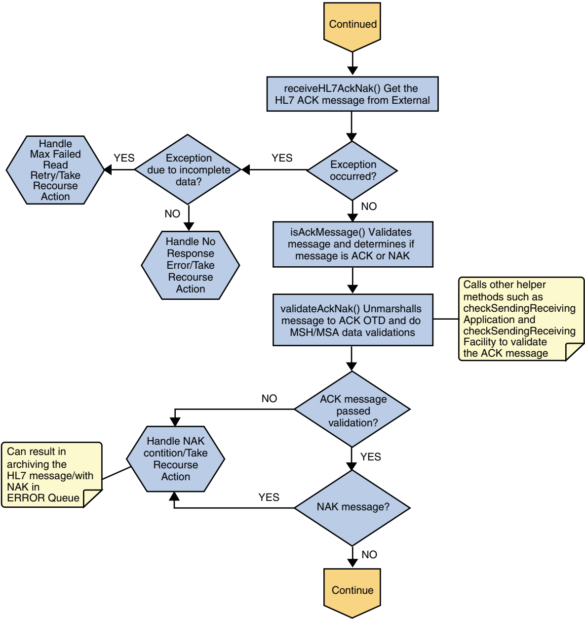
FIGURE 13 Outbound HL7 V2 Collaboration - Part 2
