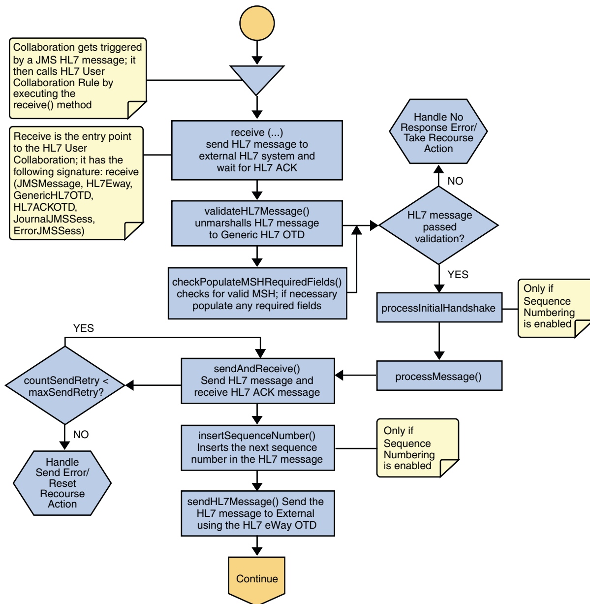
FIGURE 12 Outbound HL7 V2 Collaboration - Part 1
