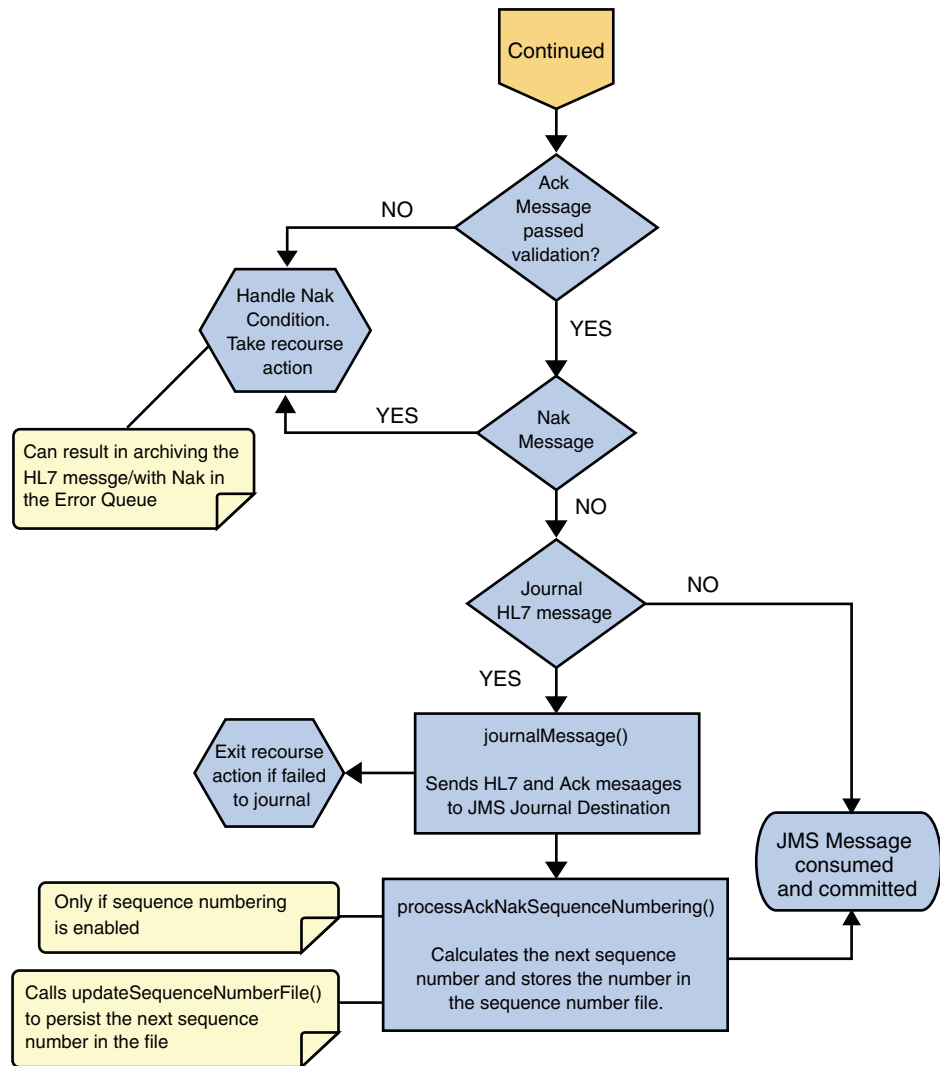
FIGURE 22 Immediate and Deferred Mode of ACK Process — Part 3
