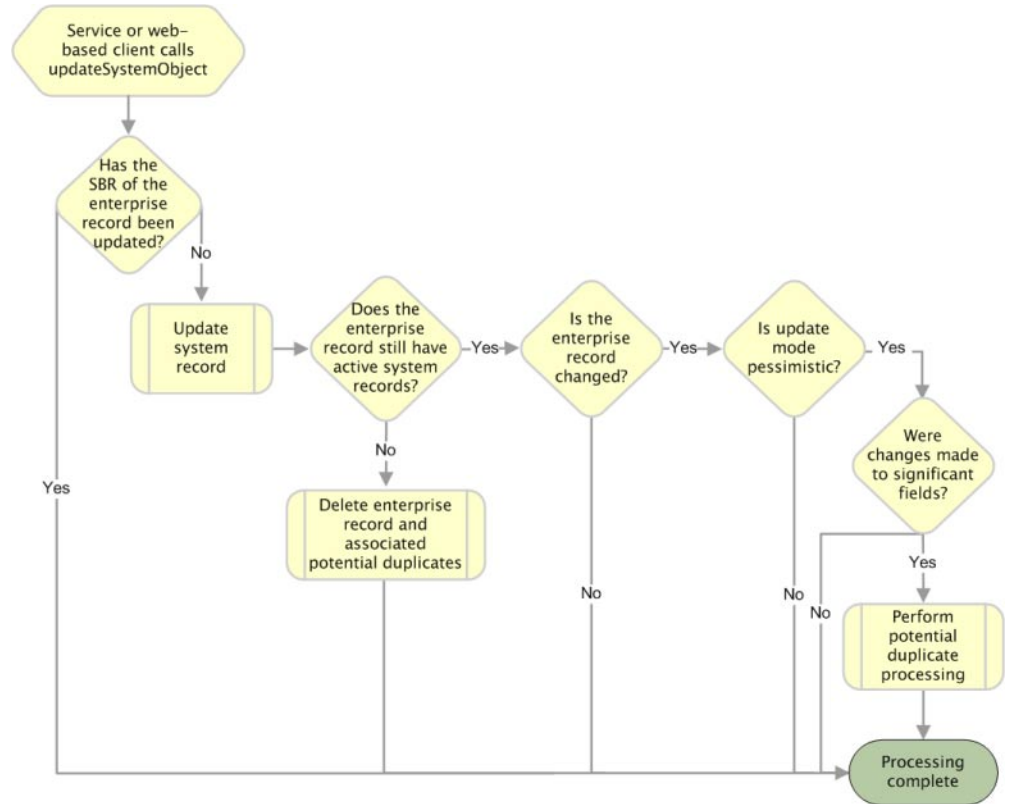
FIGURE 20 updateSystemObject Processing
