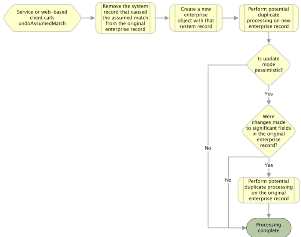
FIGURE 15 undoAssumedMatch Processing
