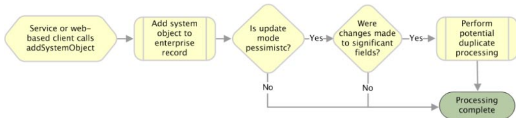
FIGURE 9 addSystemObject Processing
