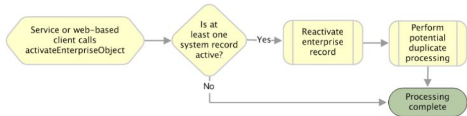
FIGURE 7 activateEnterpriseObject Processing
