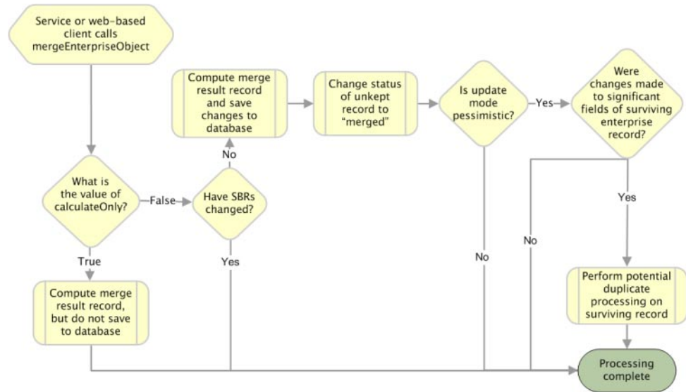
FIGURE 12 mergeEnterpriseObject Processing
