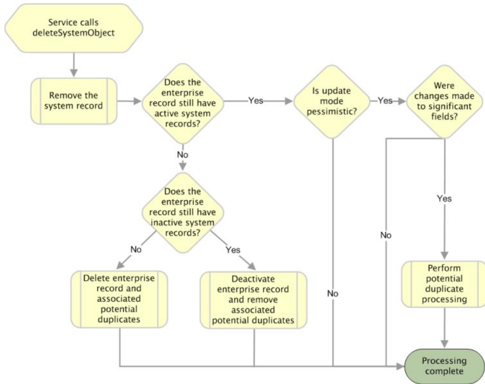
FIGURE 11 deleteSystemObject Processing
