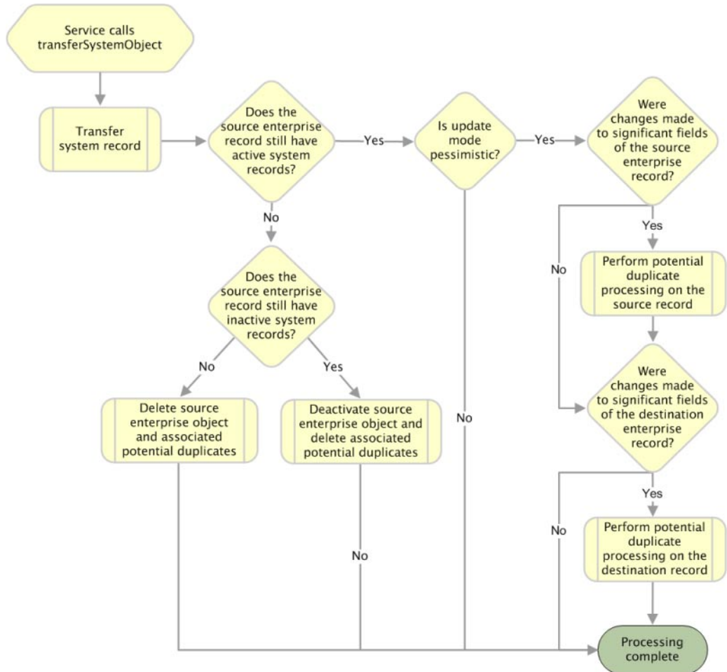
FIGURE 14 transferSystemObject Processing
