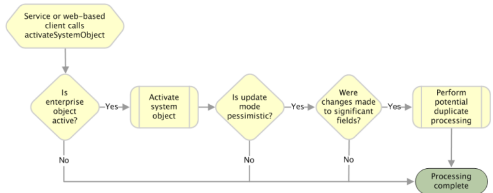
FIGURE 8 activateSystemObject Processing
