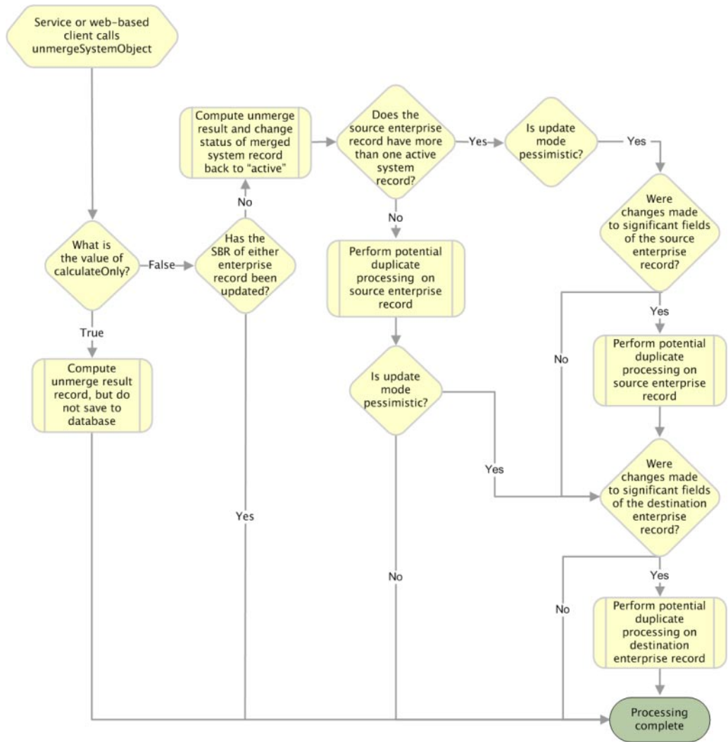
FIGURE 17 unmergeSystemObject Processing
