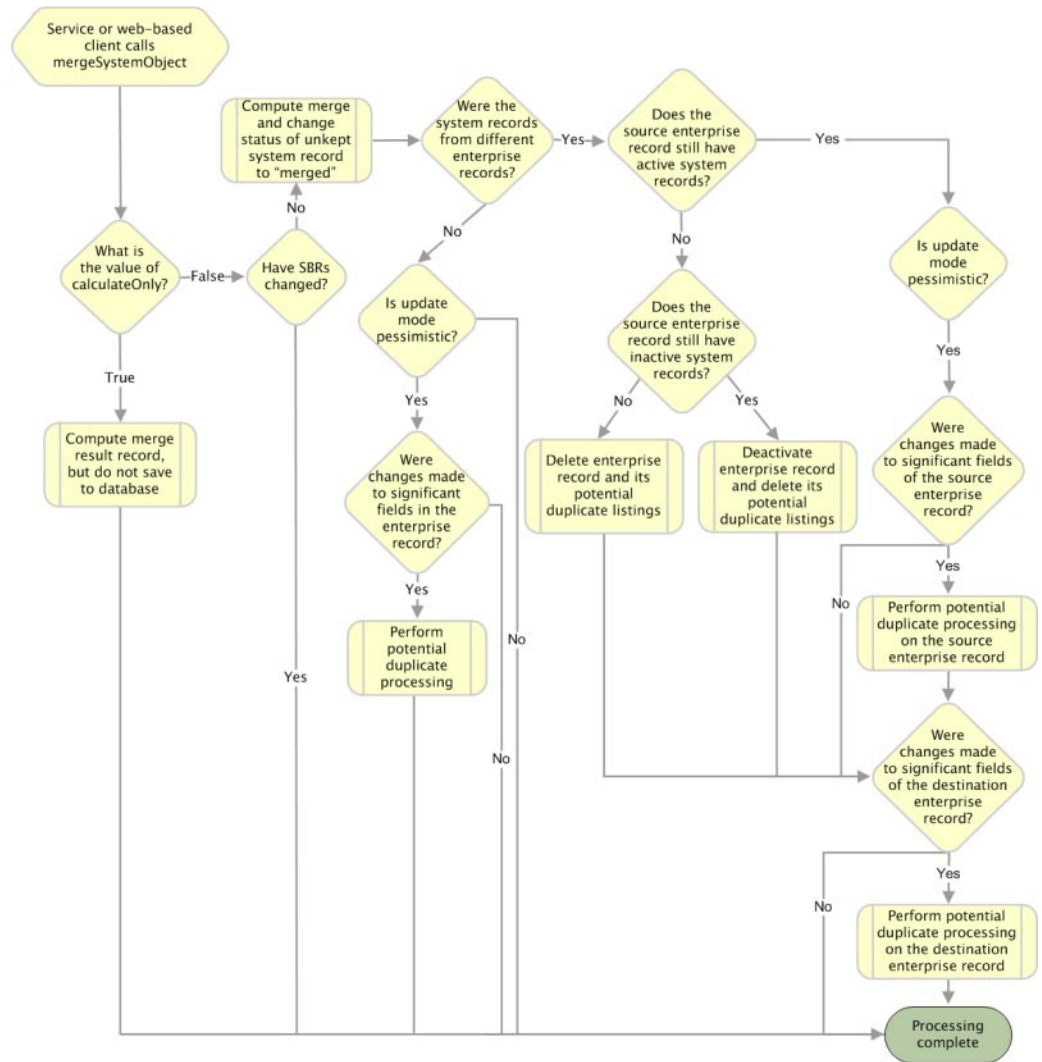
FIGURE 13 mergeSystemObject Processing
