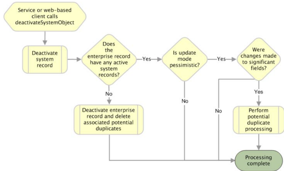
FIGURE 10 deactivateSystemObject Processing
