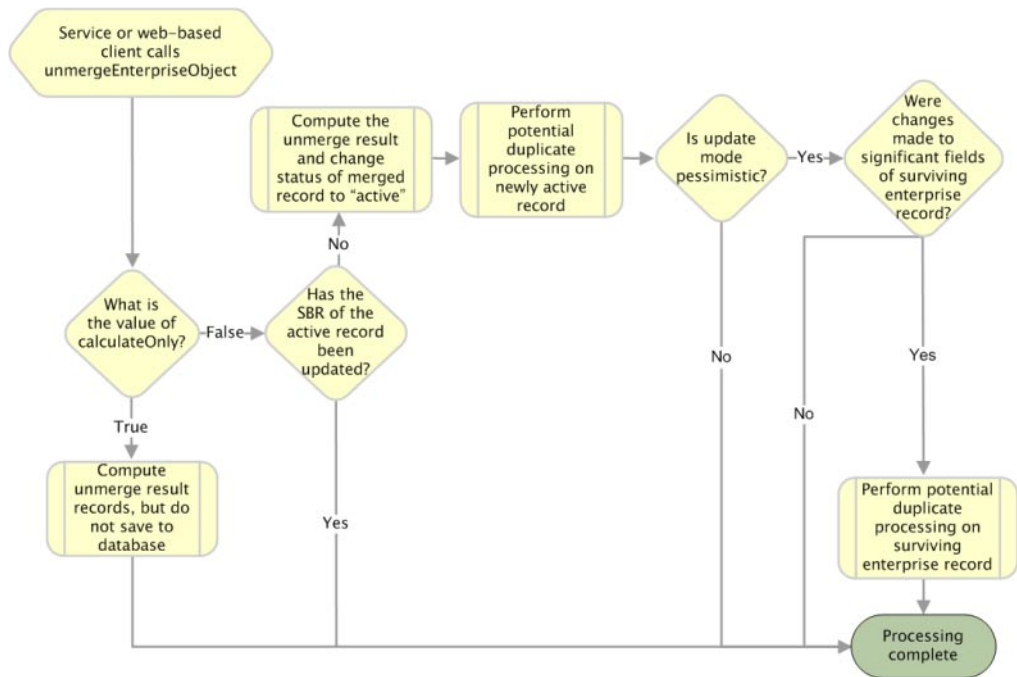
FIGURE 16 unmergeEnterpriseObject Processing
