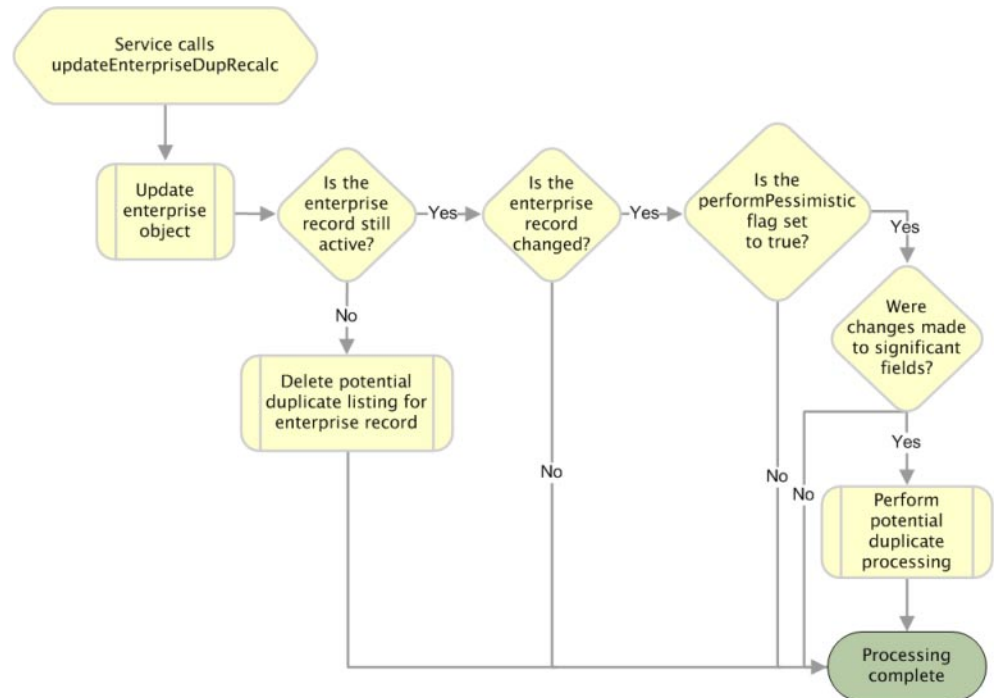
FIGURE 18 updateEnterpriseDupRecalc Processing
