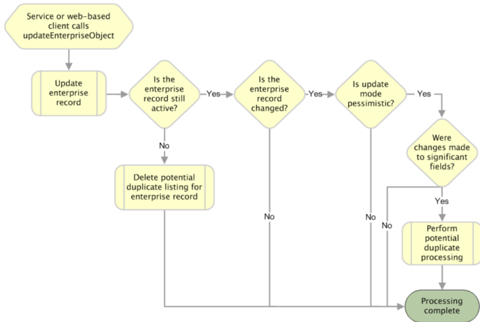
FIGURE 19 updateEnterpriseObject Processing
