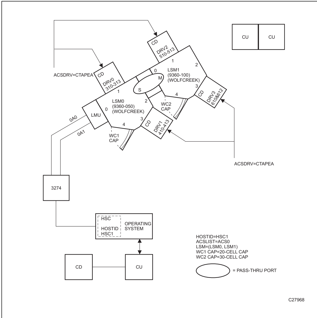
Figure 18. One Host, One ACS, Two 9360 LSM Configuration
