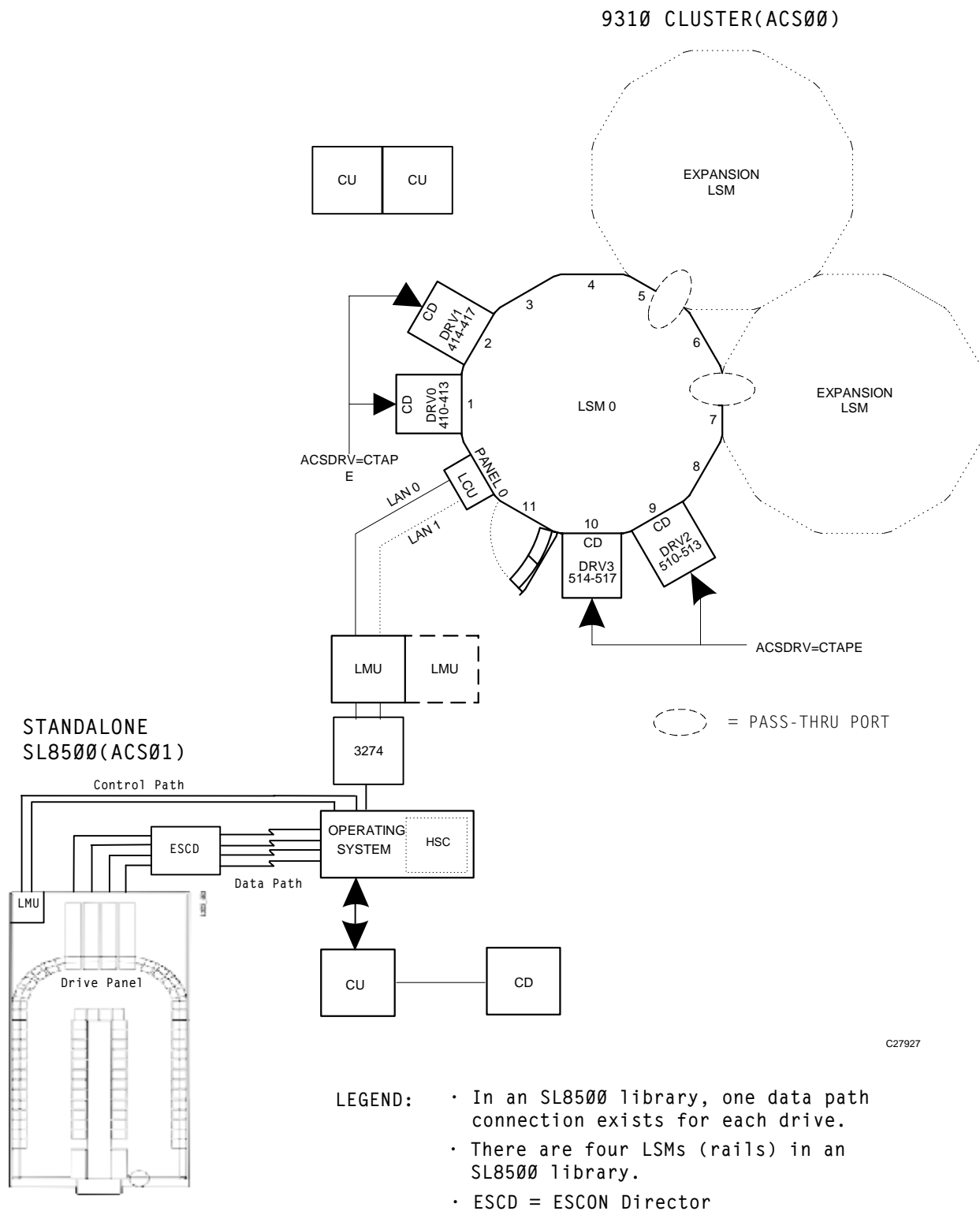
Figure 14. One host, Two ACSs, One 9310 LSM, One SL8500 Library Configuration
