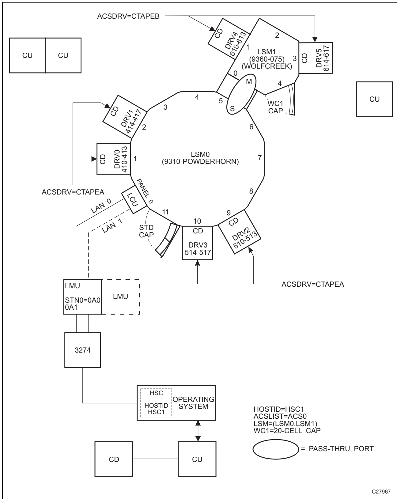
Figure 16. One Host, One ACS, One 9310 LSM, One 9360 LSM Configuration
