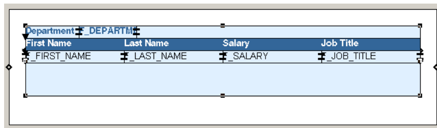
Figure 18-5 Paper Layout View with Expanded R_G_DEPARTMENT_ID Repeating Frame
