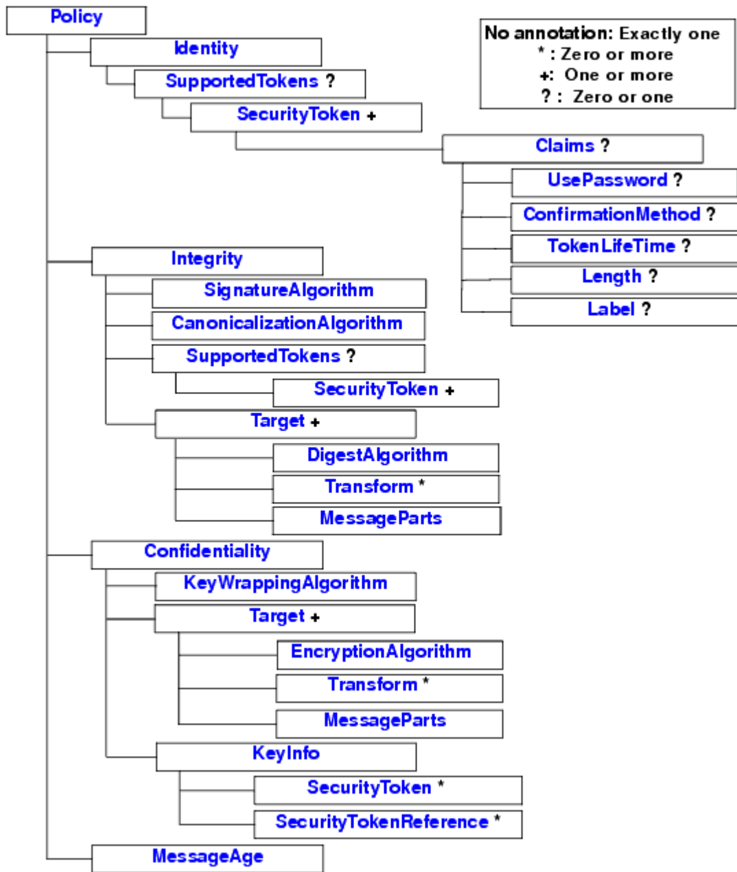
Figure 6-1 Element Hierarchy of Oracle Security Policy Assertions
