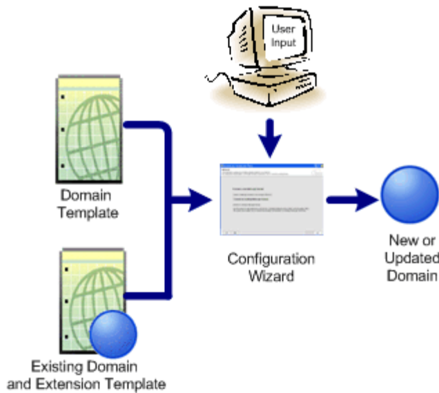
Figure 1–2 Configuration Wizard
