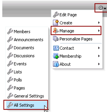
Figure 3–4 Actions Menu
