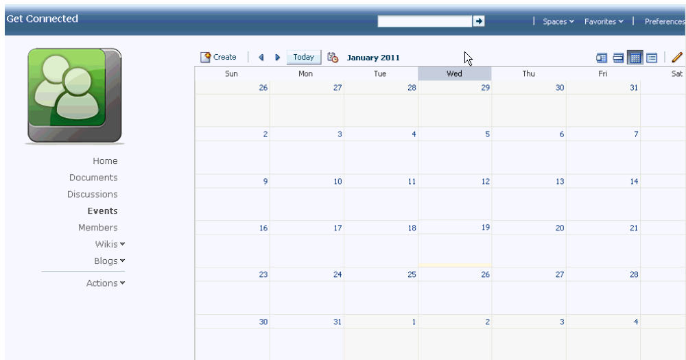
Figure 7-11 Events Calender
