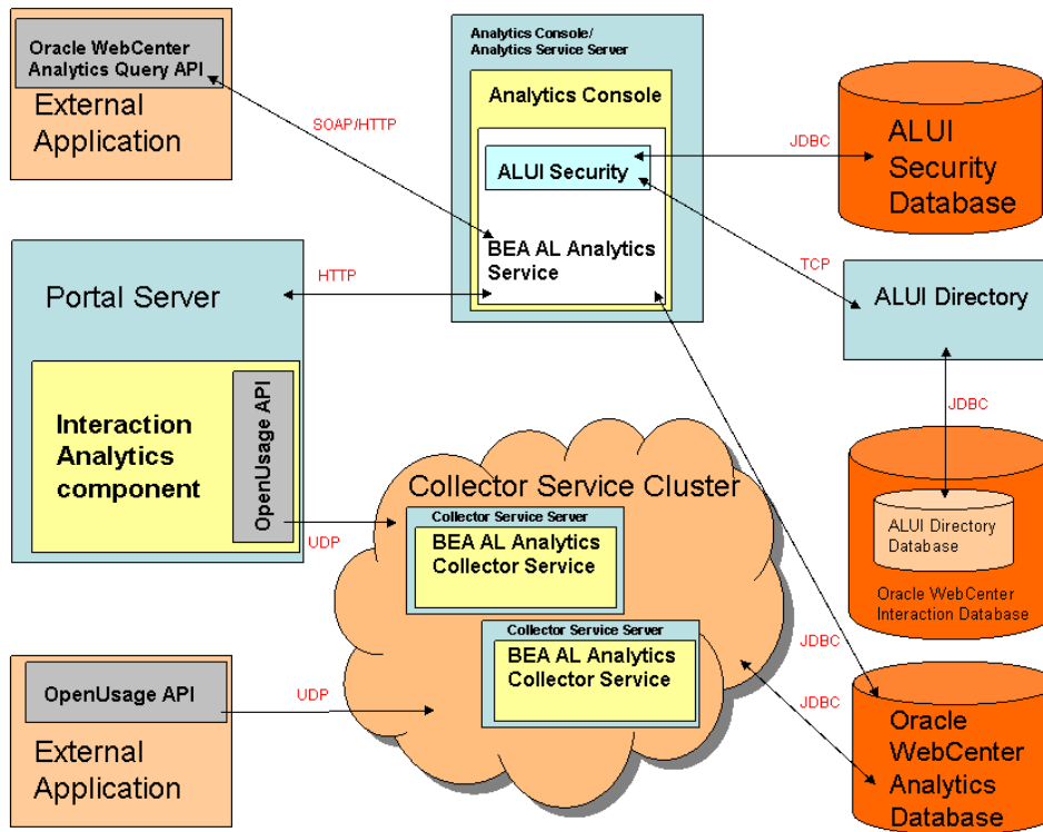
Figure 1–1 Oracle WebCenter Analytics Architecture
