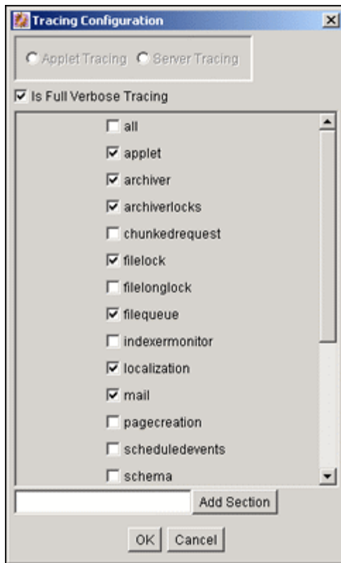
Figure 3–13 Applet-specific Tracing
