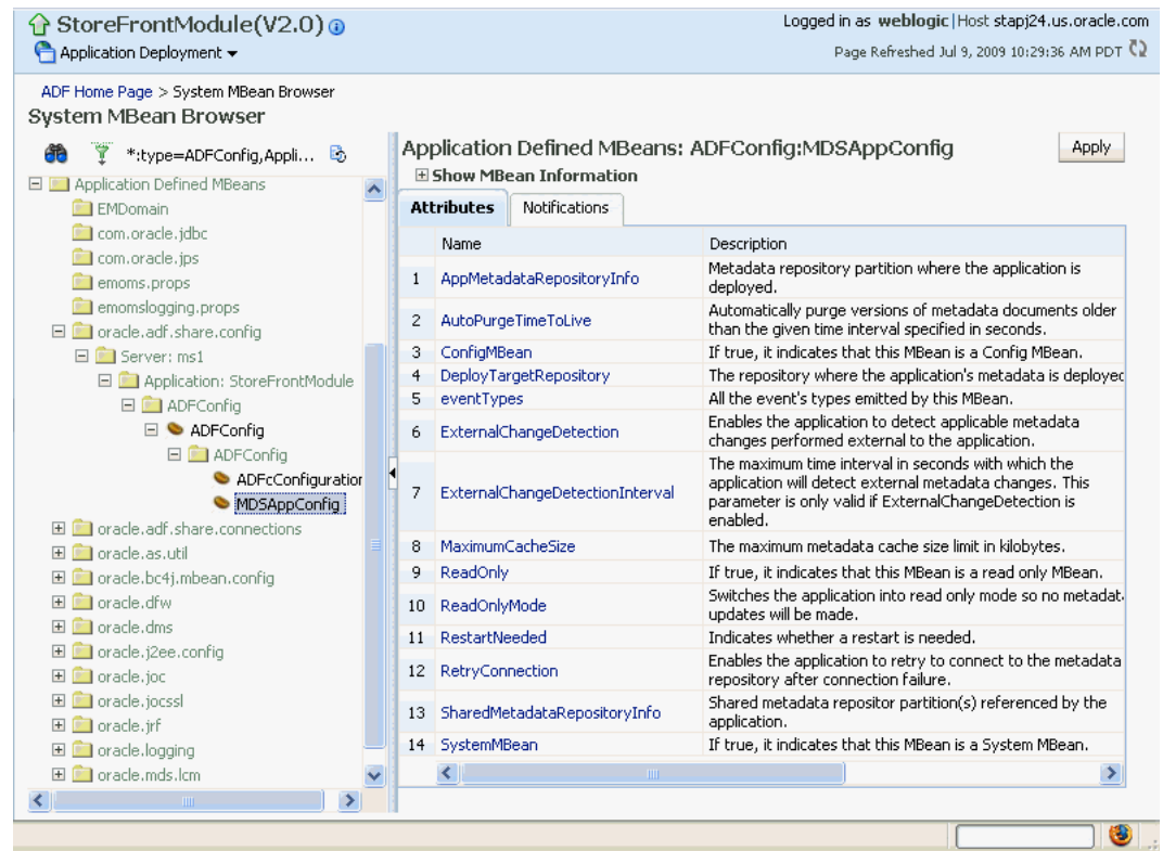
Figure 3–3 MDS MBean
