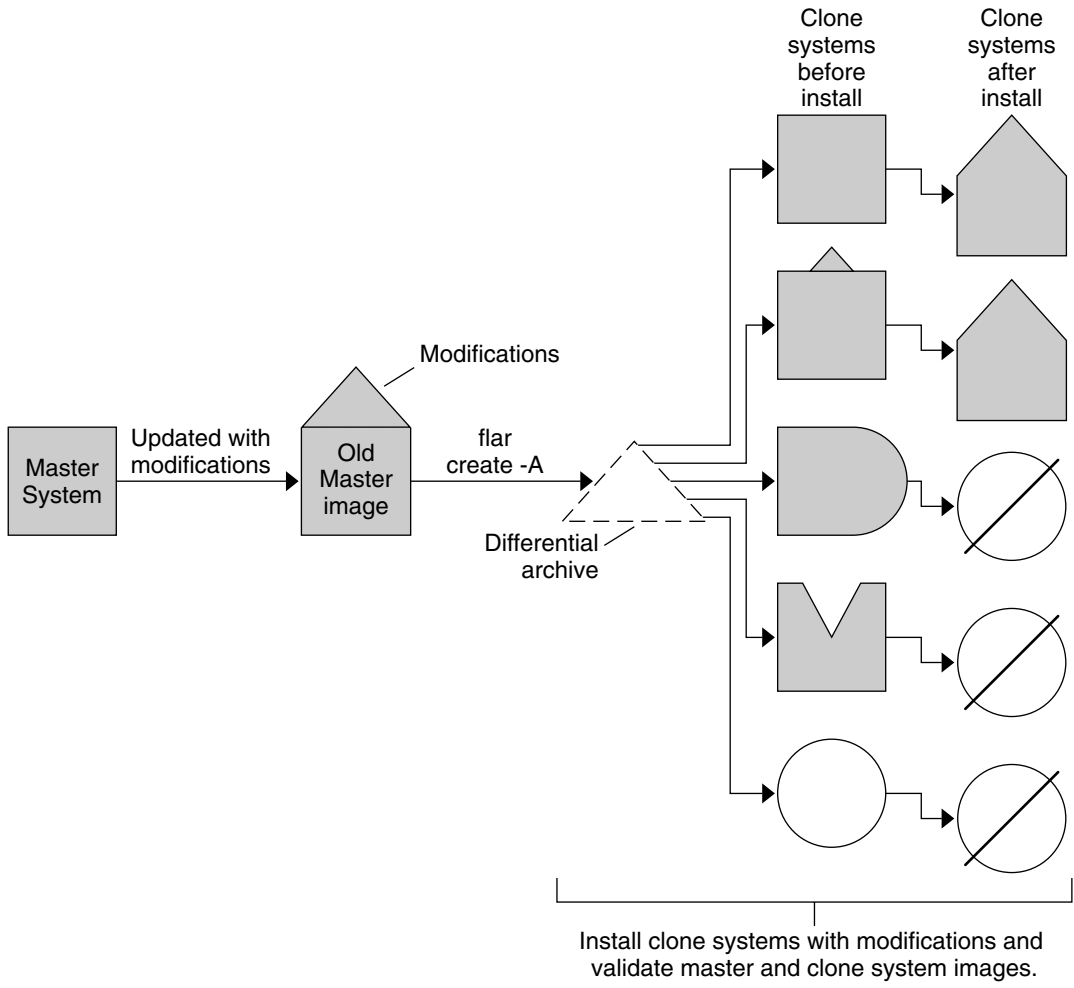
FIGURE 1-2 Solaris Flash Update
