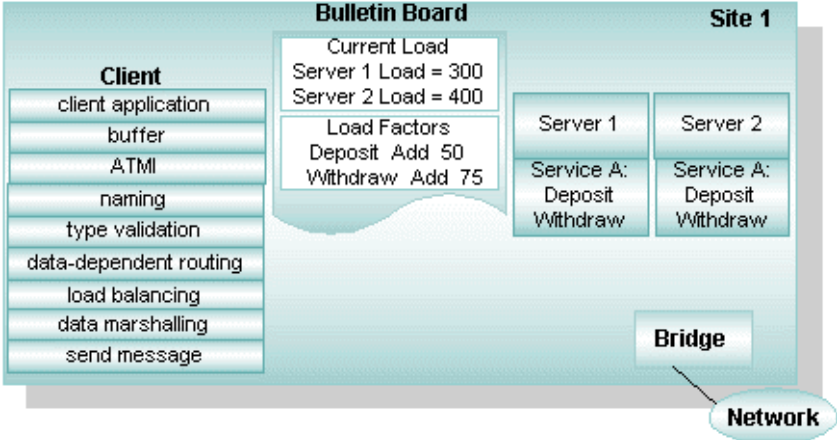
Figure 2-18 Load Balancing
