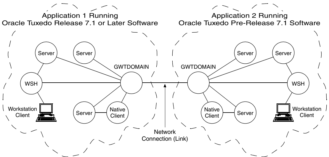
Figure 1-12 Inter-Domain Interoperability
