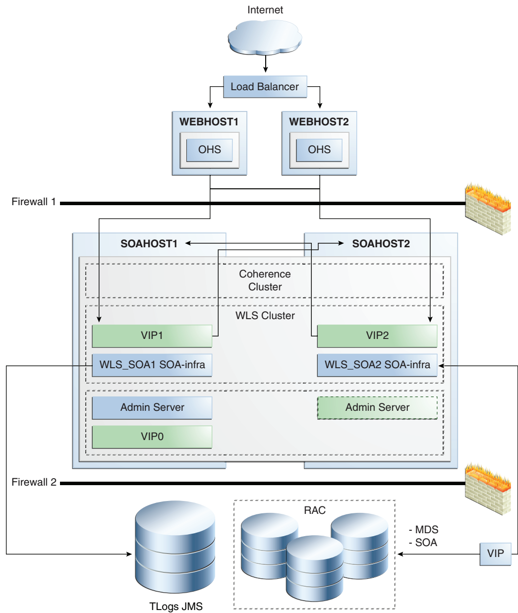
Figure 5–41 Oracle SOA Service Infrastructure High Availability Architecture
