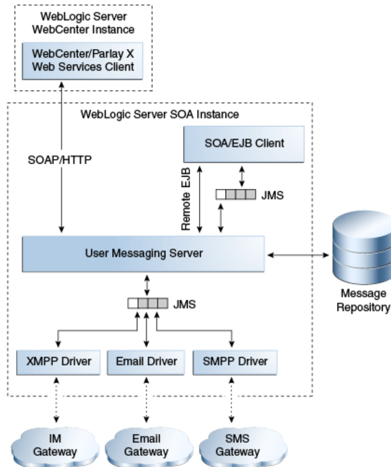
Figure 5–27 Oracle User Messaging Service Single-Instance Architecture
