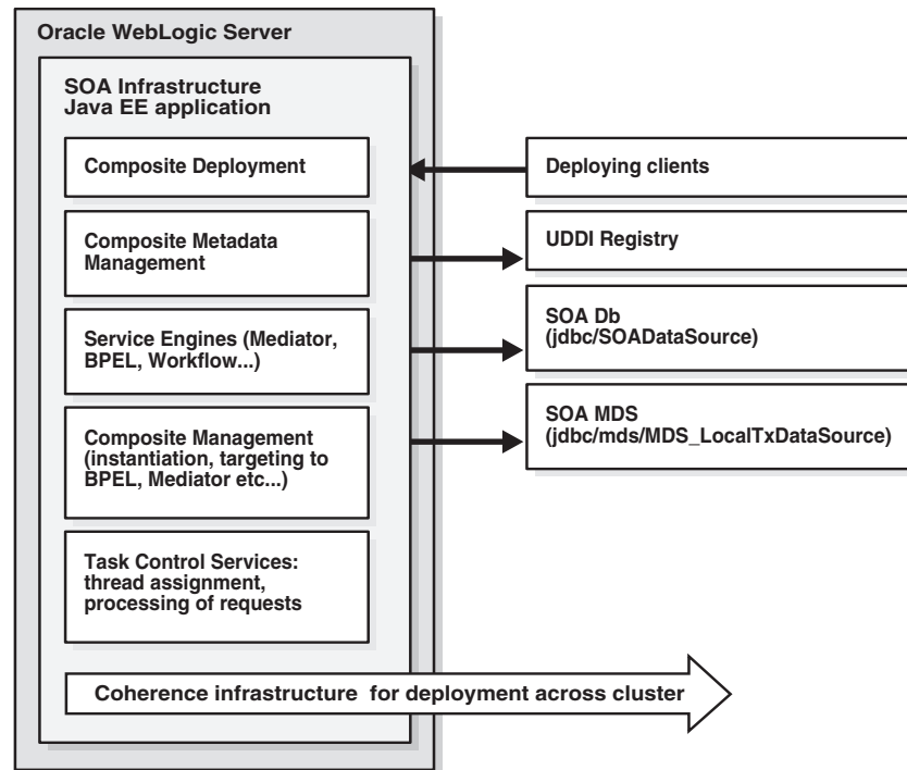
Figure 5–3 Basic Single-Node Oracle SOA Service Infrastructure Architecture
