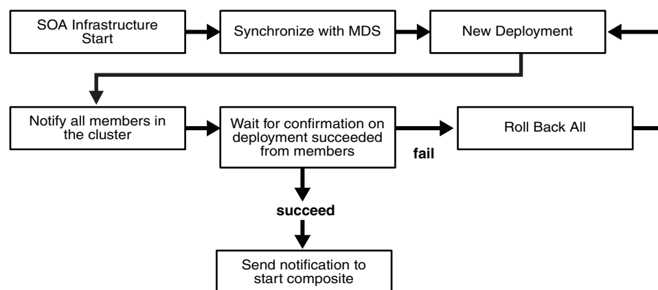
Figure 5–6 Cluster-Wide Deployment of Oracle SOA Suite Composites
