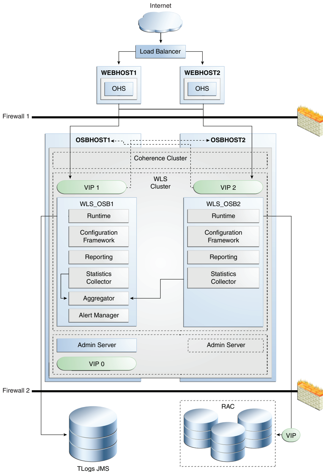
Figure 5–47 shows a two-node Oracle Service Bus cluster running on two Oracle WebLogic Servers. The Oracle WebLogic Servers are frontended by Oracle HTTP
