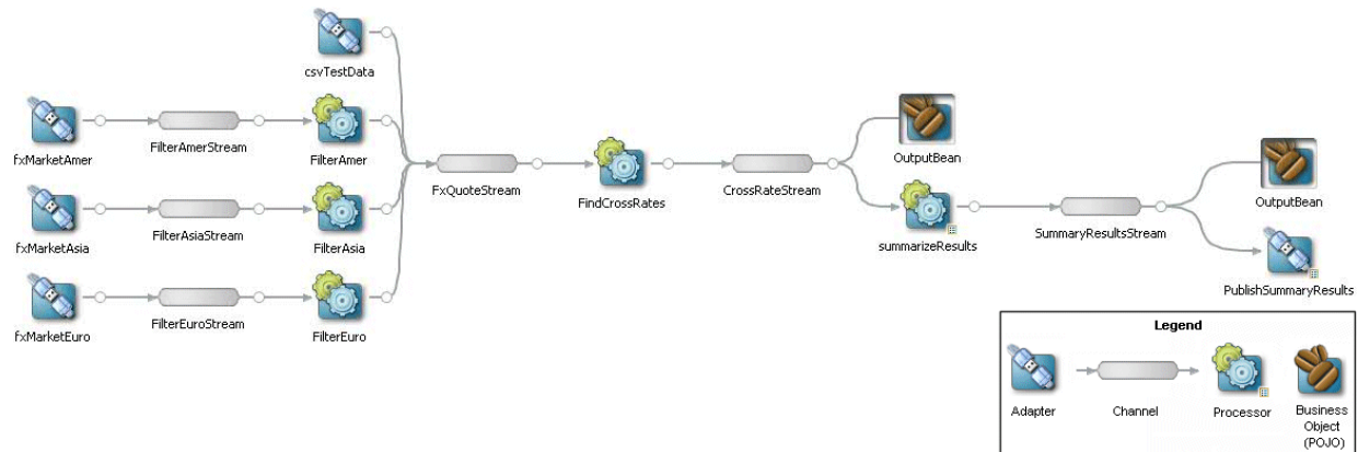
Figure 2–75 FX Example Event Processing Network
