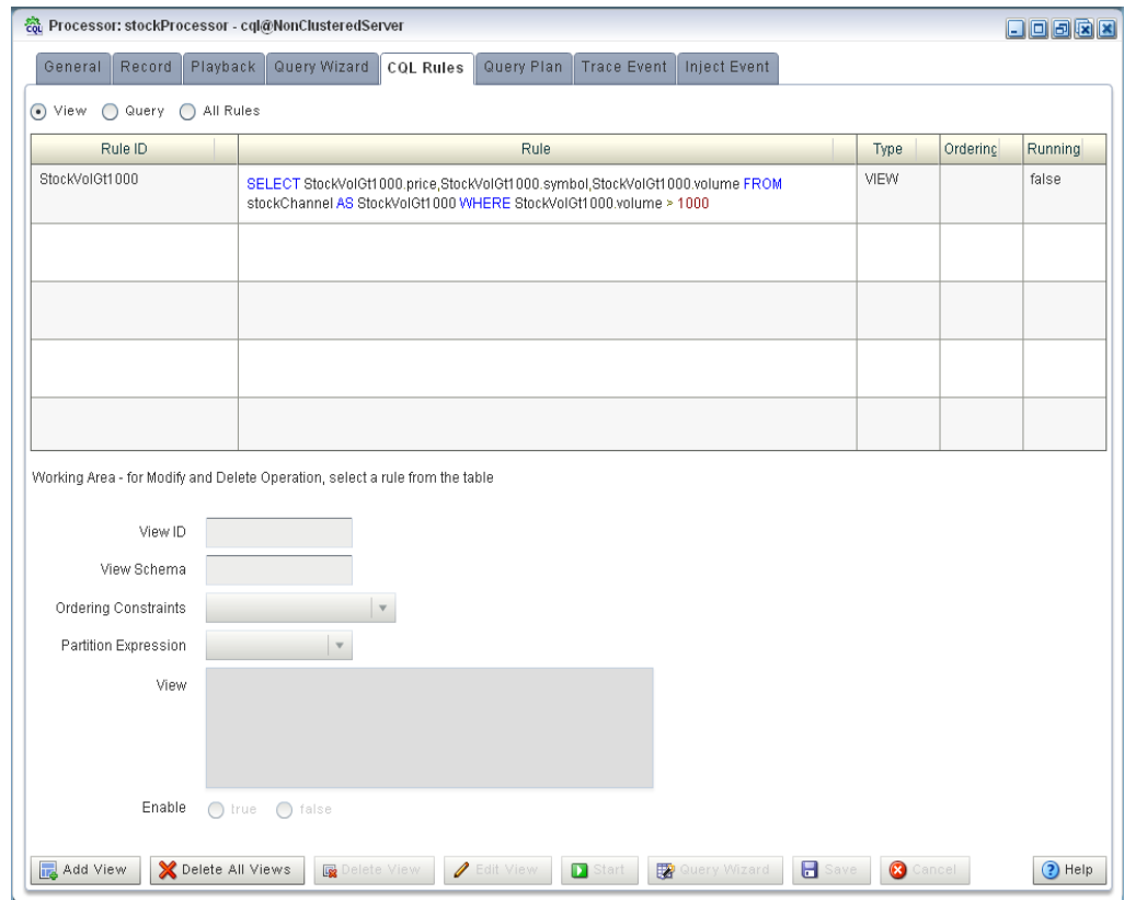
Figure 2–46 CQL Rules Tab With View StockVolGt1000
