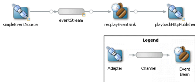
Figure 2–78 The Event Record and Playback Example Event Processing Network
