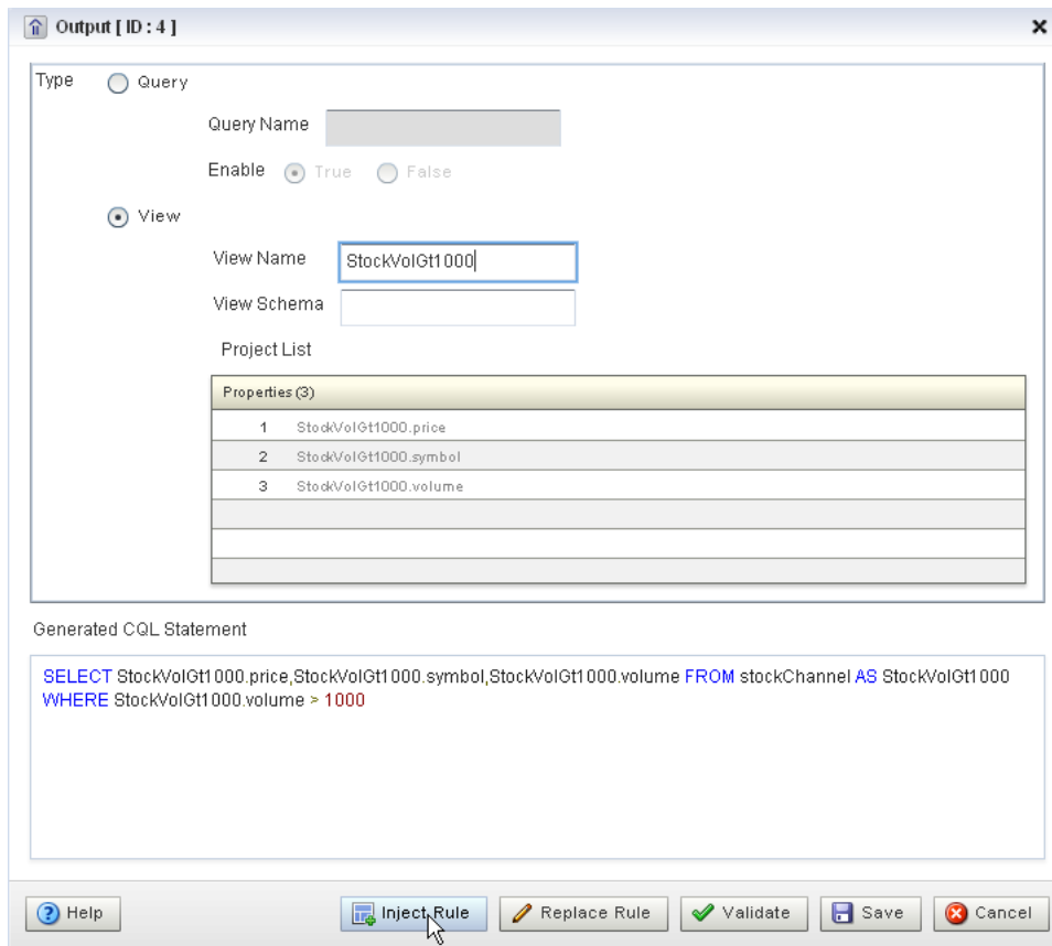
Figure 2–44 Output Configuration Dialog
