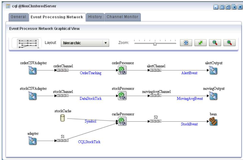
Figure 2–31 CQL Application: Event Processing Network Tab
