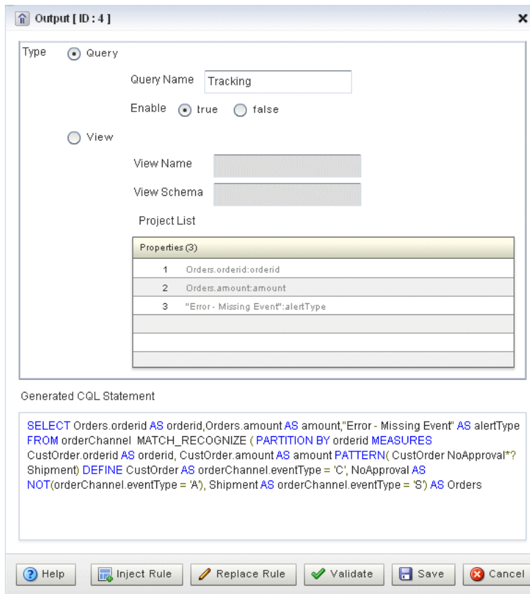
Figure 2–24 Output Configuration Dialog
