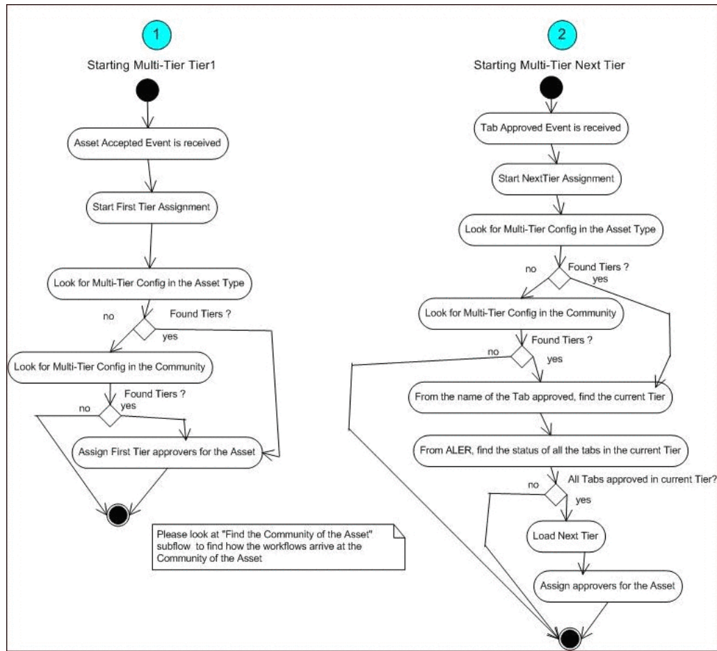
Figure 9–38 Multi-tier Automatic Assignment Flowchart
