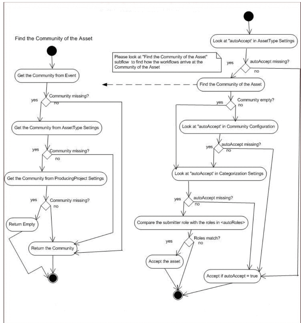
Figure 9–35 Automatic Asset Acceptance Flowchart
