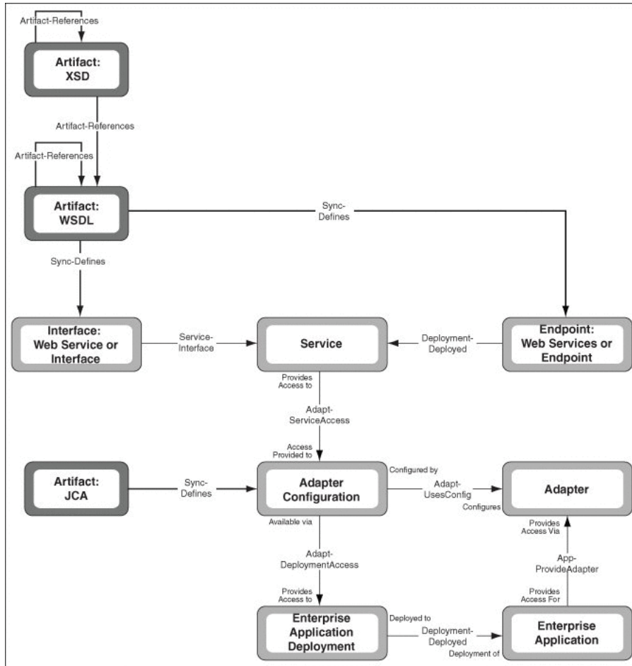
Figure 6-4 A Sample Asset Model Diagram
