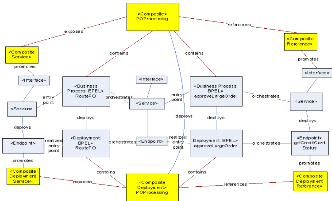
Figure 6-4 A Sample Asset Model Diagram
