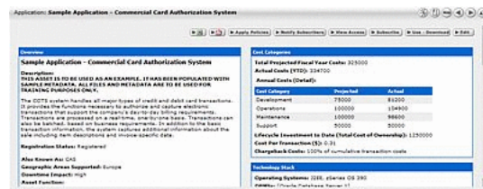
Figure 16–11 Sample Application
