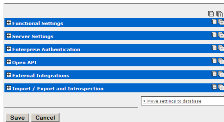
Figure 16–2 Functional Settings
