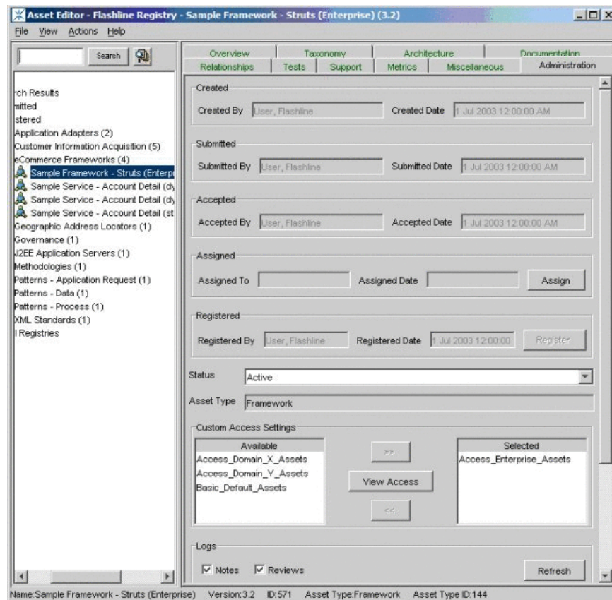
Figure 4–40 Asset Editor
