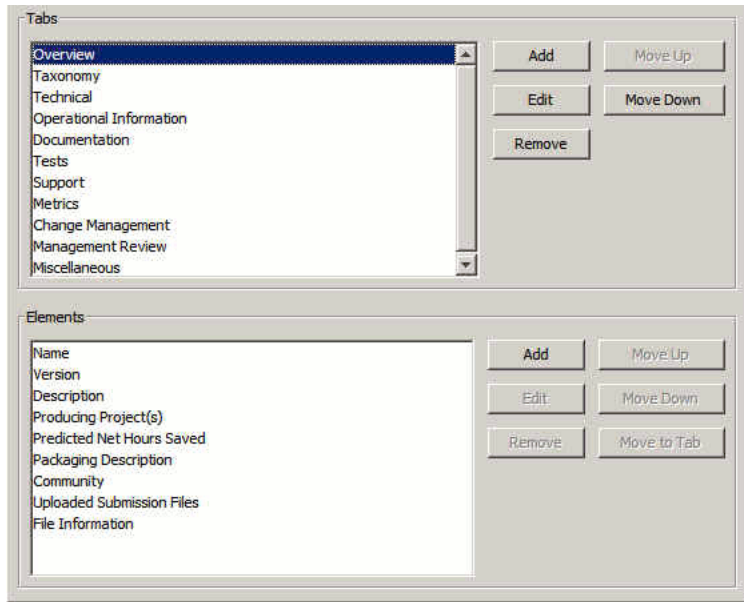
Figure 13–4 Tabs List
