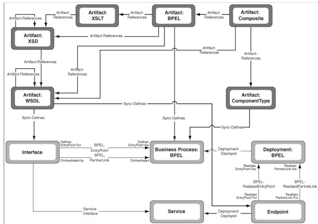
Figure 6-3 Asset Model
