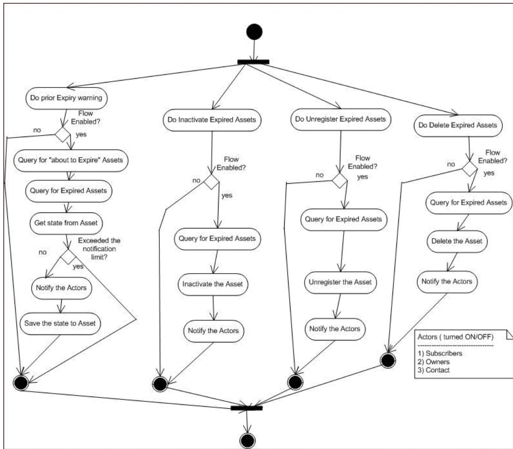
Figure 9-42 Validation Expiration Flowchart
