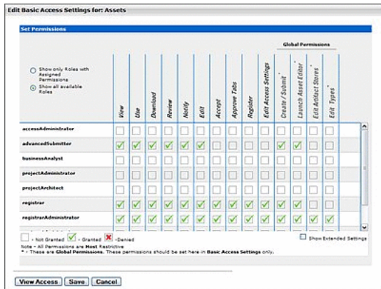
Figure 1–36 Set Permissions
