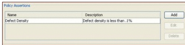
Figure 14–12 Policy Assertions
