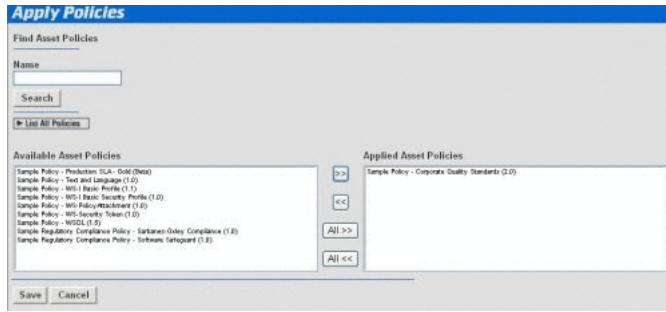
Figure 14–14 Apply Policies
