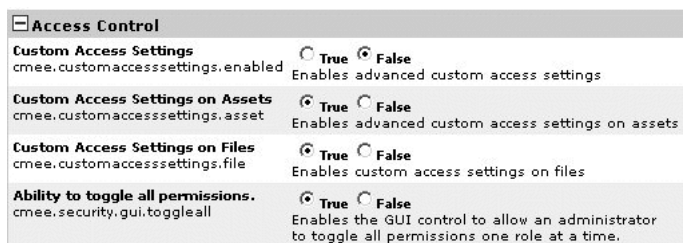
Figure 16–37 Access Control
