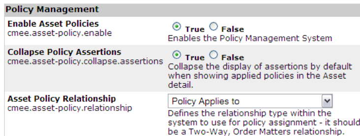
Figure 14–2 Policy Management
