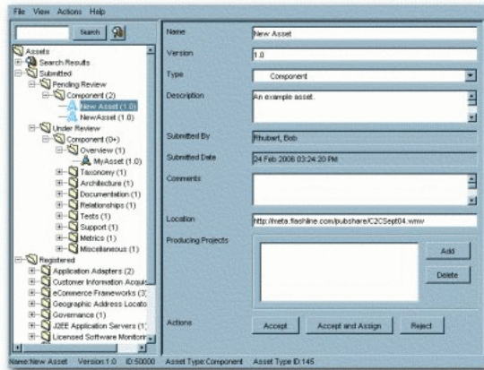
Figure 9–2 Asset Editor
