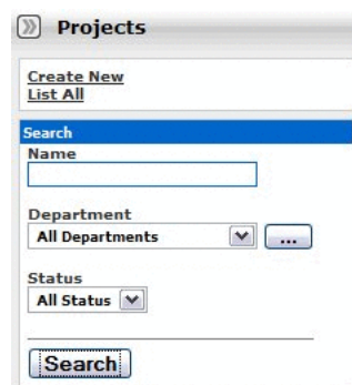
Figure 11–14 Projects Screen
