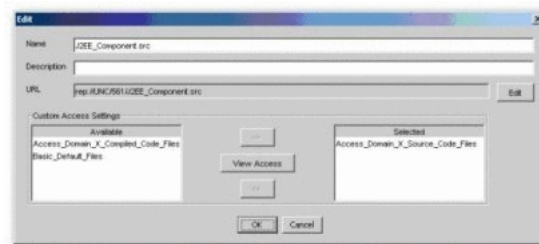
Figure 4-53 Edit Dialog
