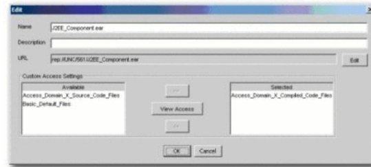
Figure 4-52 Edit Dialog
