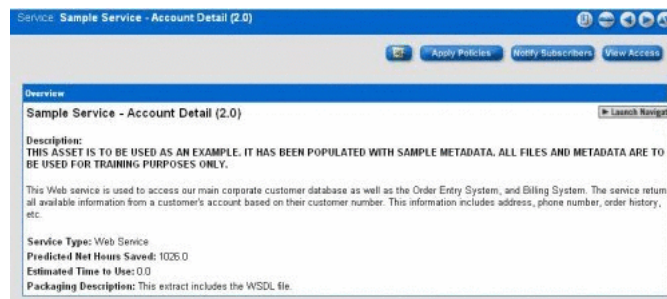
Figure 14-13 Overview
