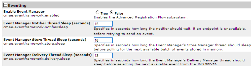
Figure 16–76 Eventing
