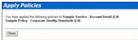
Figure 14–15 Apply Policies
