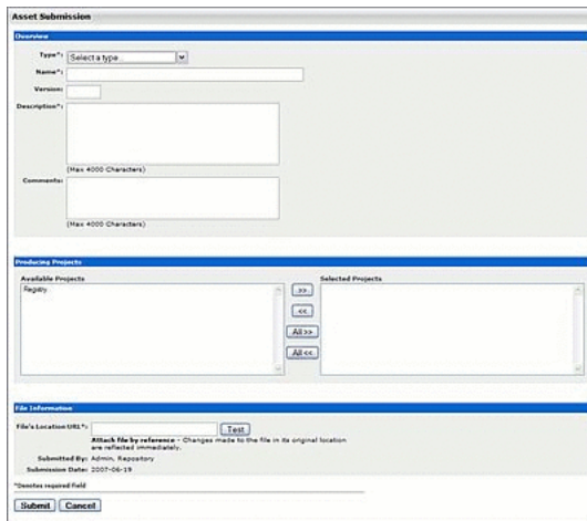
Figure 16–29 Asset Submission
