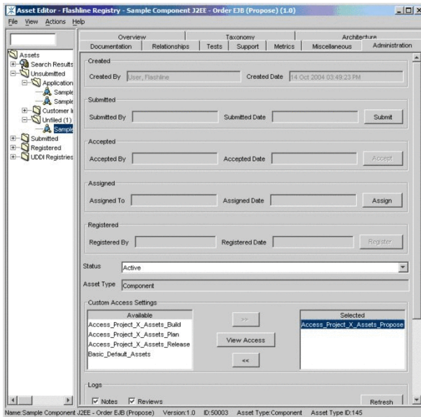
Figure 4–49 Asset Editor
