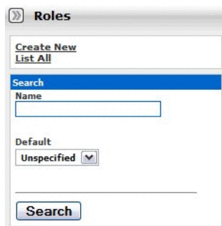
Figure 4–18 Roles Section
