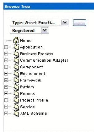
Figure 16–7 Browse Tree
