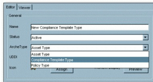
Figure 11-3 Editor Tab
