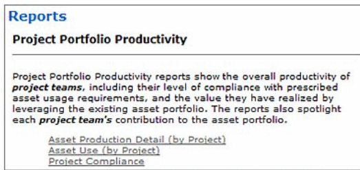
Figure 11–19 Reports Section
