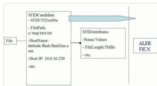
Figure 13–10 Object Model
