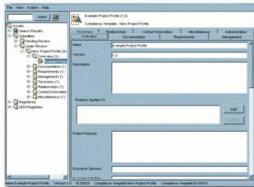
Figure 11–11 Asset Editor
