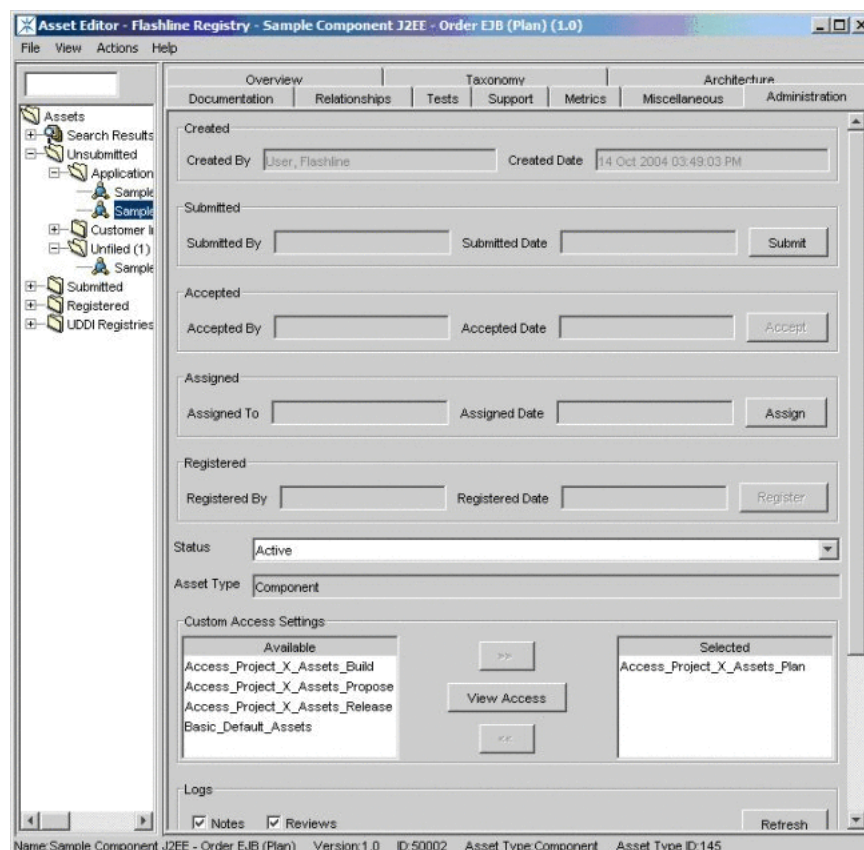
Figure 4–51 Asset Editor
