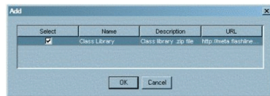
Figure 13–8 Add Dialog
