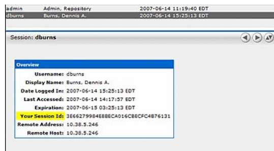
Figure 1–41 Sessions Pane
