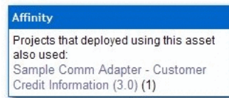
Figure 16–51 Affinity
