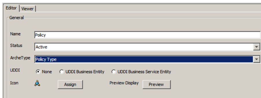
Figure 14–5 Type Manager
