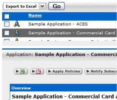
Figure 16–50 Export Assets
