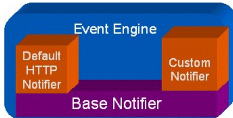
Figure 9–51 Notifier Plug-in
