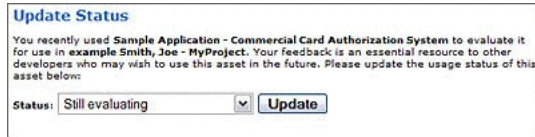
Figure 16–36 Update Status
