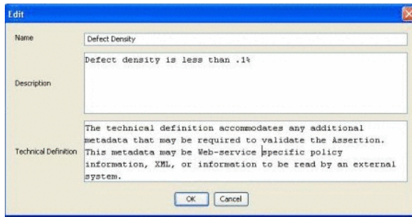
Figure 14–11 Edit Dialog
