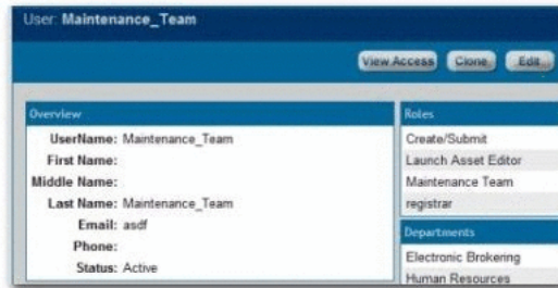
Figure 4-55 User: Maintenance_Team
