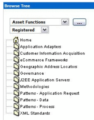
Figure 16–6 Browse Tree
