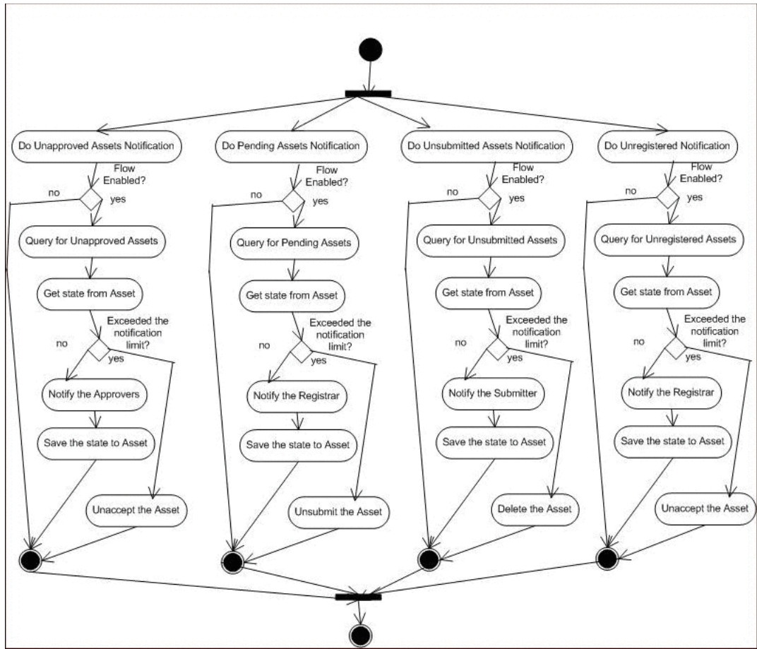
Figure 9-41 Time-based Escalation Flowchart
