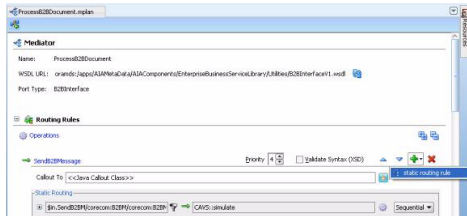
Figure 17–13 Addition of Custom Routing Rules to AIAB2BInterface/ProcessB2BDocument.mplan
