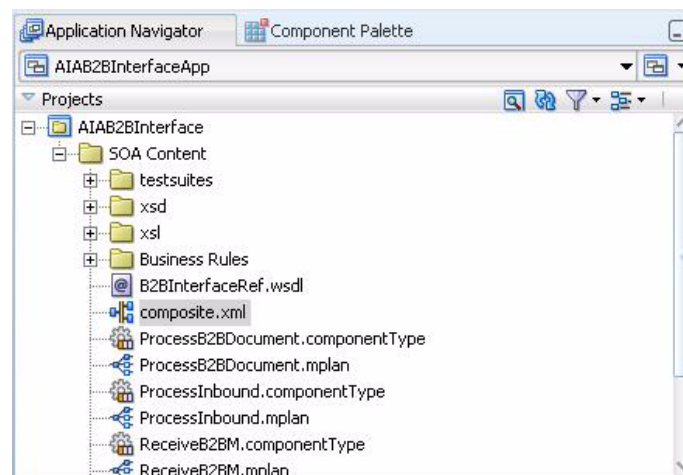
Figure 17–10 AIAB2BInterface/composite.xml in the Composite Editor
