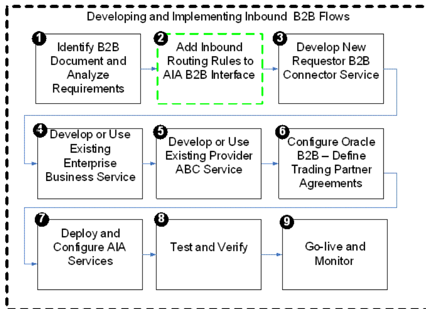
Figure 18–3 Step 2: Adding Inbound Routing Rules to an AIA B2B Interface
