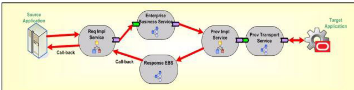
Figure 25-7 Example of the Asynchronous Delayed Response Pattern
