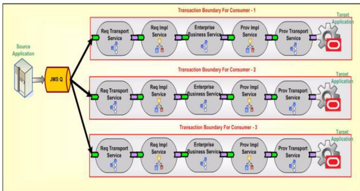
Figure 25–6 Setting Up Multiple Consumers or Listeners Connected to the Source Queue
