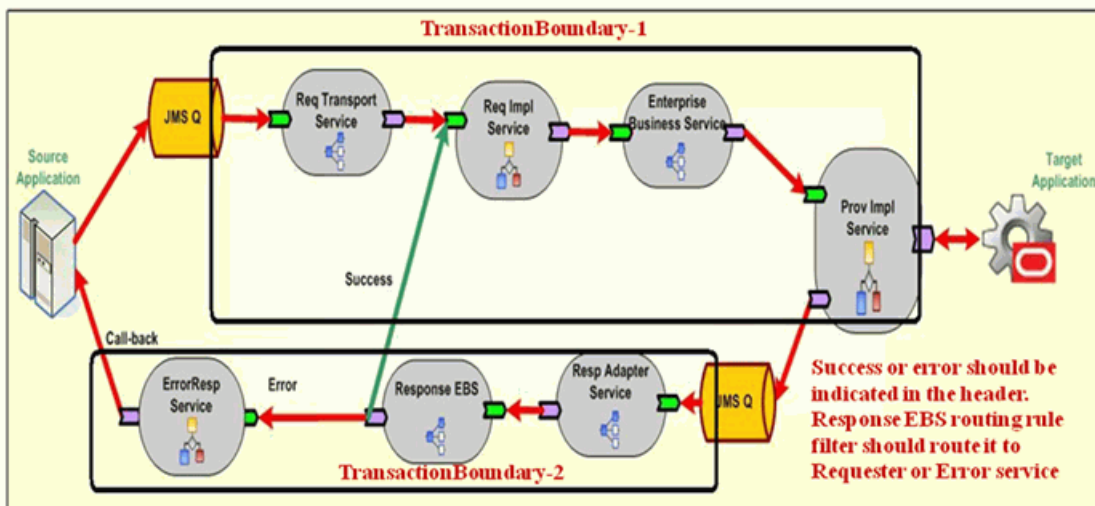
Figure 12-8 Programming Model 1: Using a Separate Service for Error Handling
