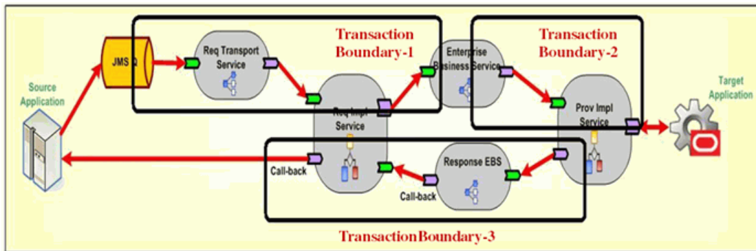
Figure 12–10 Programming Model 3: Using a Parallel Routing Rule in the EBS
