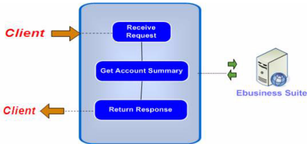
Figure 20-4 Example of Integration Flow Leveraging Provider Services
