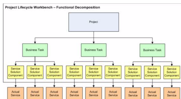
Figure 2-1 Functional Decomposition of a Project into Actual Implemented Services
