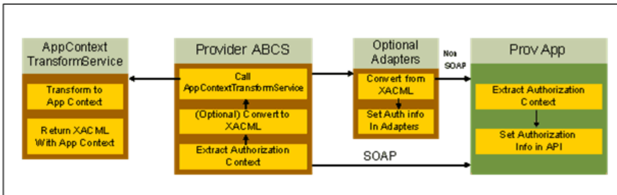
Figure 26–4 Provider Application Flow
