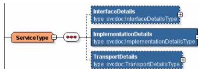
Figure 9–2 Example Of Annotation Elements
