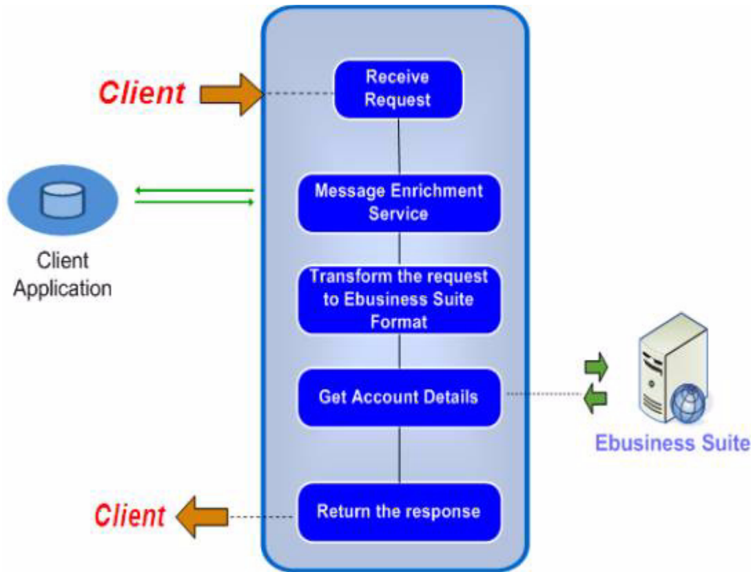
Figure 20–3 Example of Integration Flow with Native Application Services
