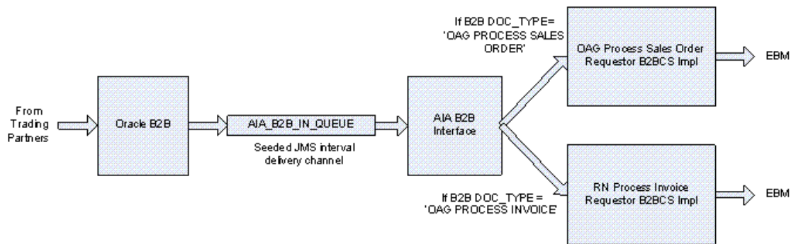
Figure 18–4 Oracle B2B Routing New B2B Documents to Requester B2B Services
