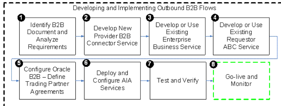
Figure 17-42 Step 8: Going Live and Monitoring
