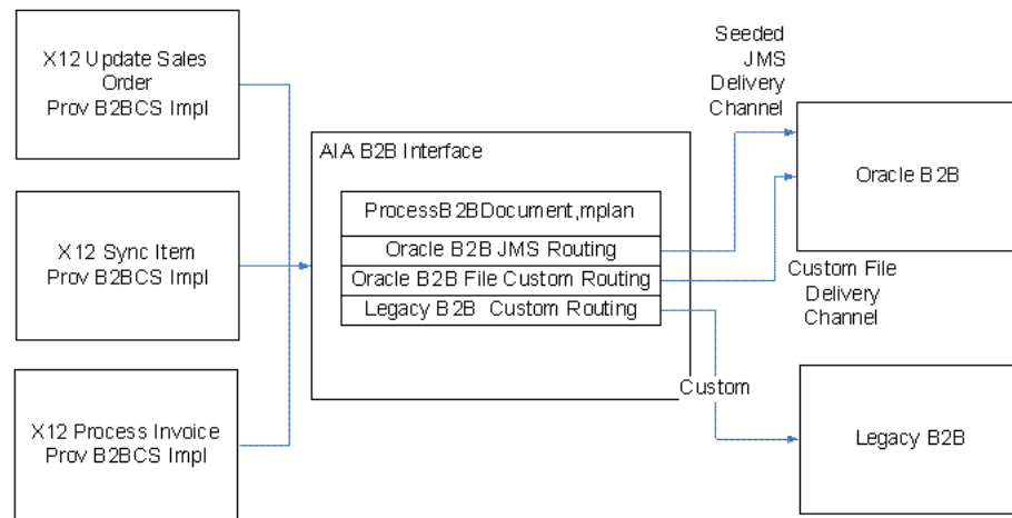
Figure 17–9 AIA B2B Interface Support for Custom Internal Delivery Channels and Legacy B2B Connectivity
