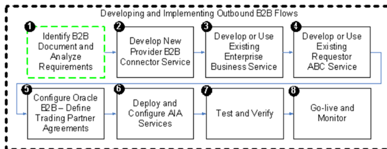
Figure 17–2 Step 1: Identifying B2B Document and Analyzing Service Requirements
