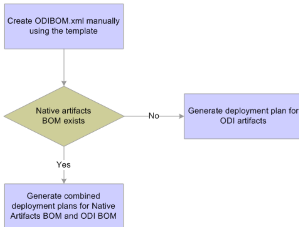
Figure 7-1 Generate Deployment Plans for ODI
