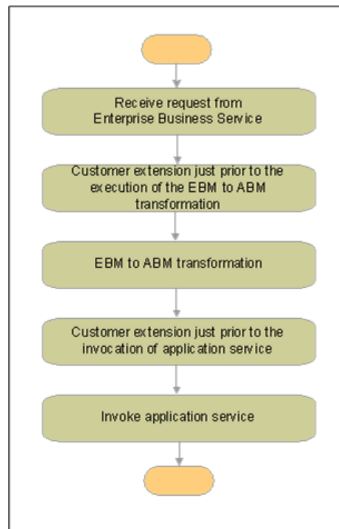
Figure 13-4 Provider-Specific ABCS Using Fire-and-Forget Interaction Style
