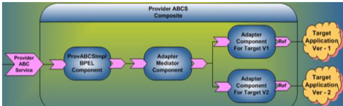
Figure 13–9 Introducing a Version Adapter
