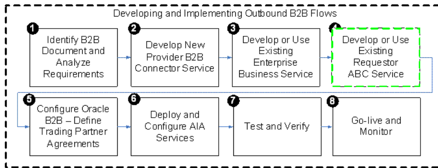
Figure 17-34 Step 4: Developing or Extending an Existing Requester ABCS
