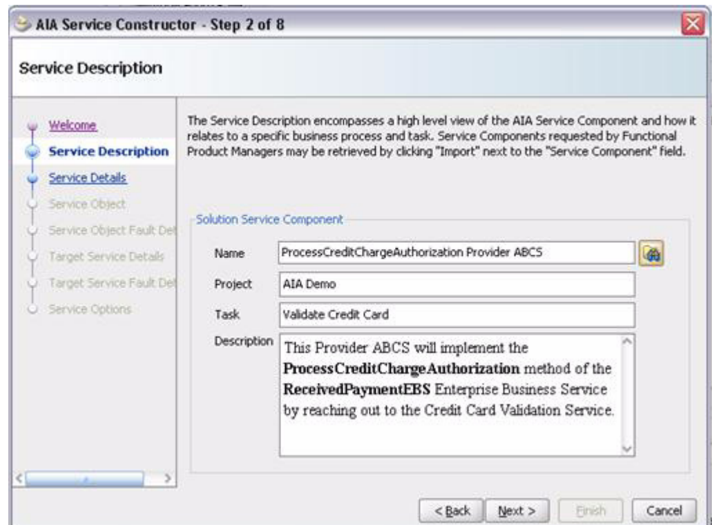
Figure 19–10 Service Description Populated from Project Lifecycle Workbench Service Solution Component Request
