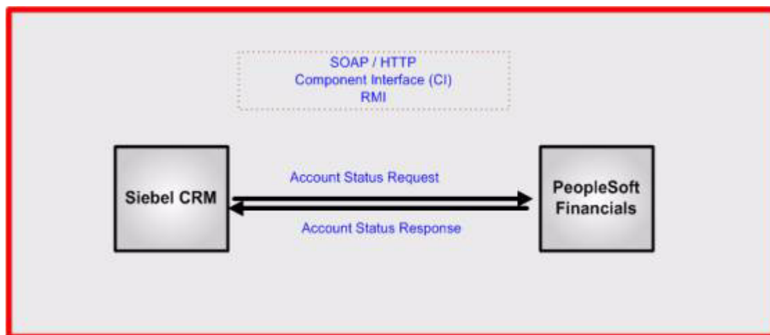
Figure 20–2 Example of a Requester Application Interacting Directly with a Provider Application
