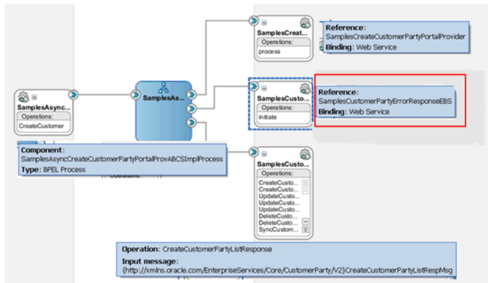
Figure 12–12 Async Provider ABCS Composite with a Second Reference to ResponseEBS
