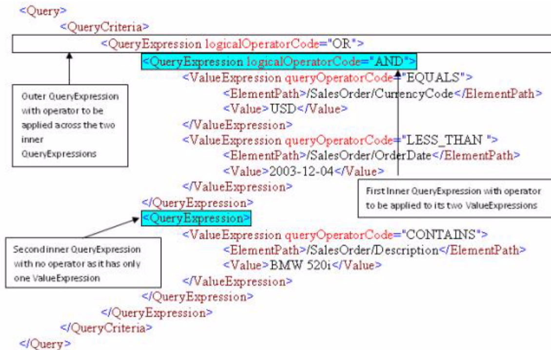
Figure 12–13 Example of Query with Nested Query Expressions
