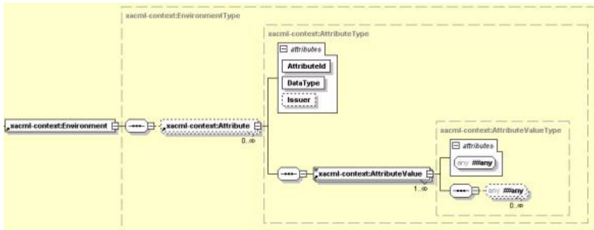
Figure 26–9 Structure of XACML Environment
