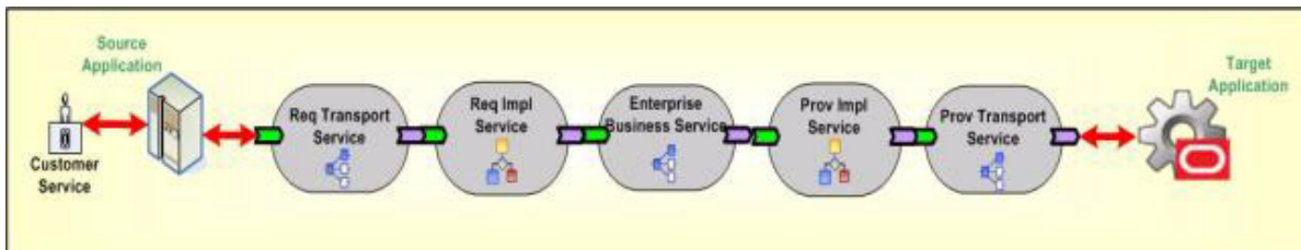
Figure 25–1 Invoking an EBS Synchronously by the Requester Application
