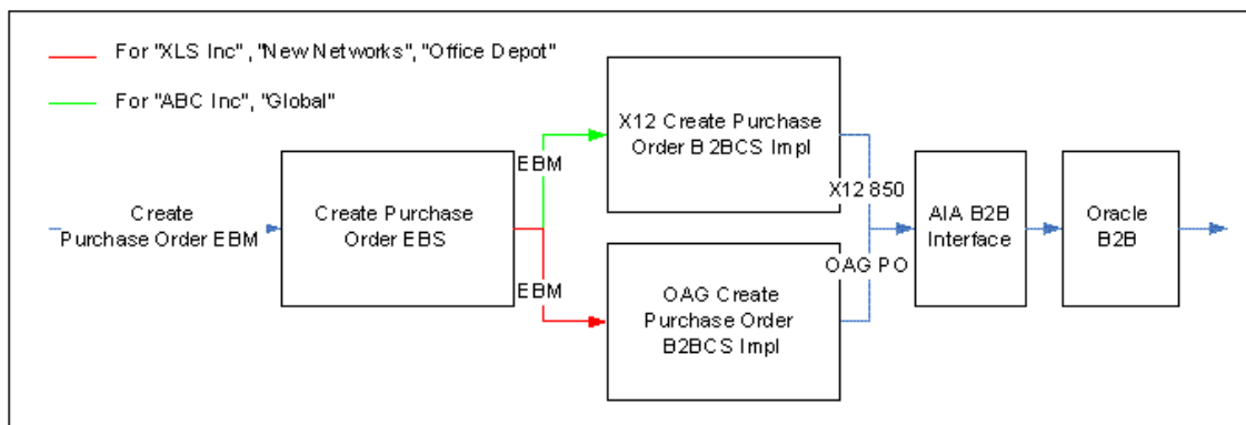
Figure 17–30 B2B Implementation in which Trading Partners Need the Same EBM Data Sent Using Different B2B Document Protocols
