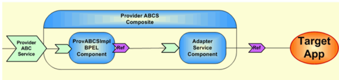
Figure 27–3 Example of ABCS and Transport Adapter Service in the Same Composite
