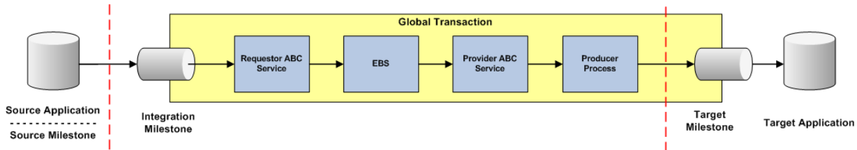
Figure 24–3 Integration Flow in Which the Receiver Target Milestone is Within the Global Transaction Space
