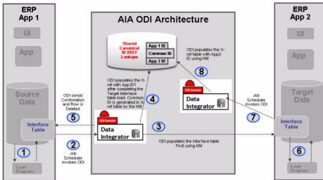
Figure 22–1 Initial Data Loads
