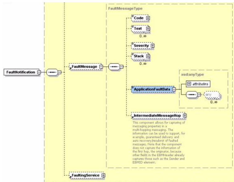
Figure 24–11 ApplicationFaultData Element Highlighted in Meta.xsd
