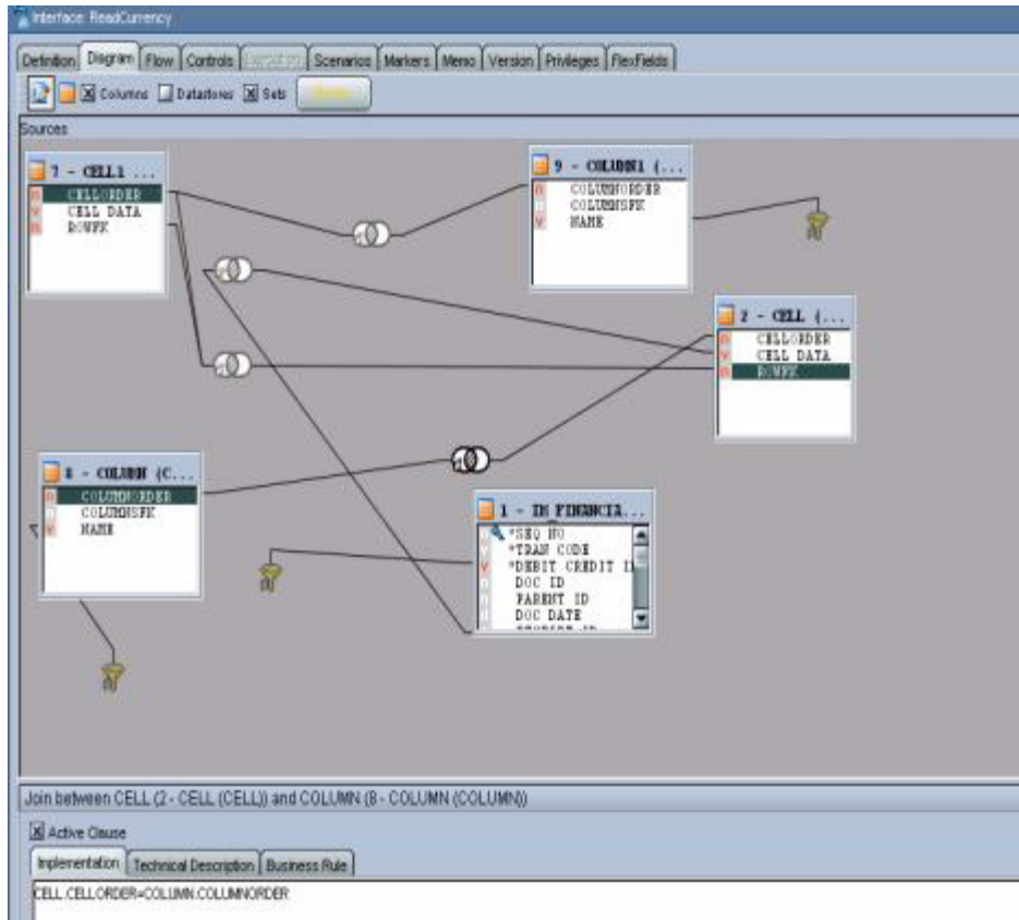
Figure 22–15 Join of the CELL Table with the COLUMN Table
