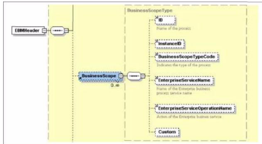
Figure 23–11 Structure of the BusinessScope Element
