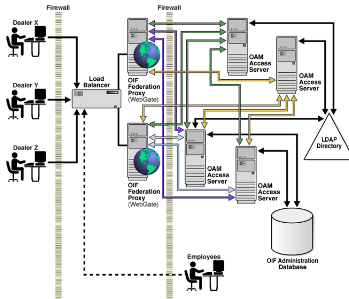
Figure 2–11 A Typical Federation Deployment Architecture
