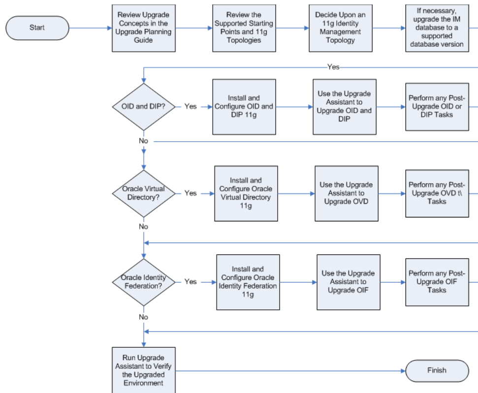
Figure 2-1 Flow Chart of the Oracle Identity Management Upgrade Process
