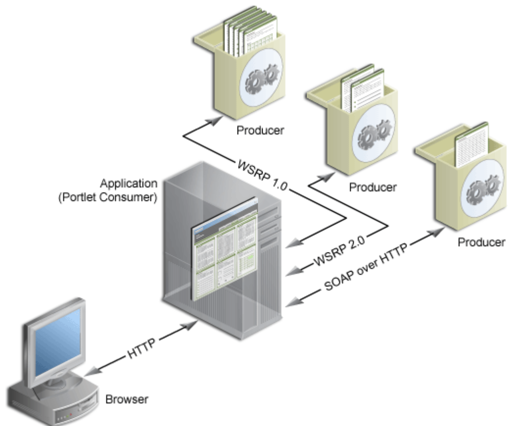
Figure 57-9 Producer Architecture
