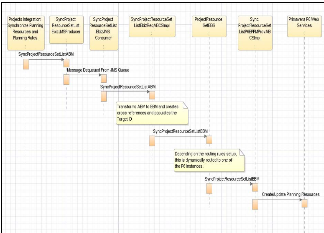
Synchronization of Resources, Roles, and Expense Categories integration flow sequence diagram
