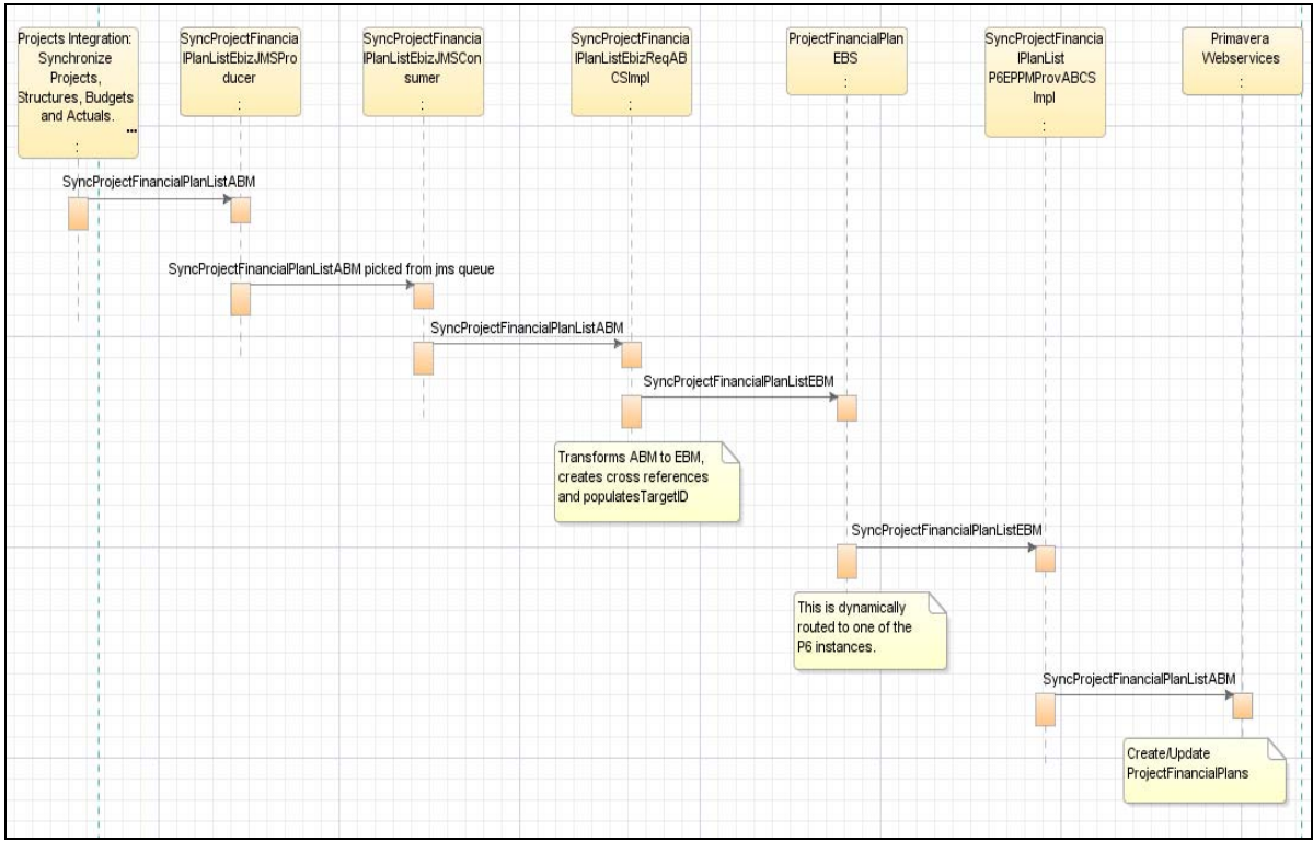
SyncProjectFinancialListEbizReqABCSImpl sequence diagram
