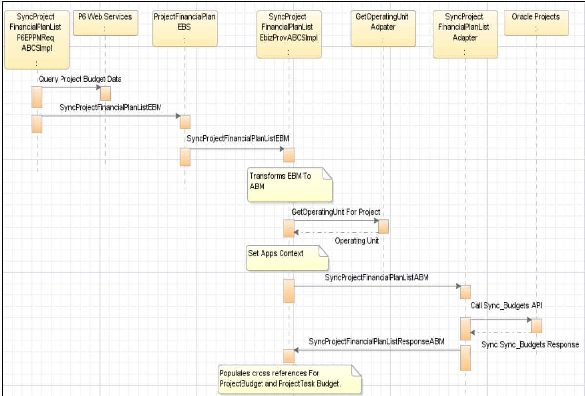
SyncProjectFinancialListEbizProvABCSImpl sequence diagram
