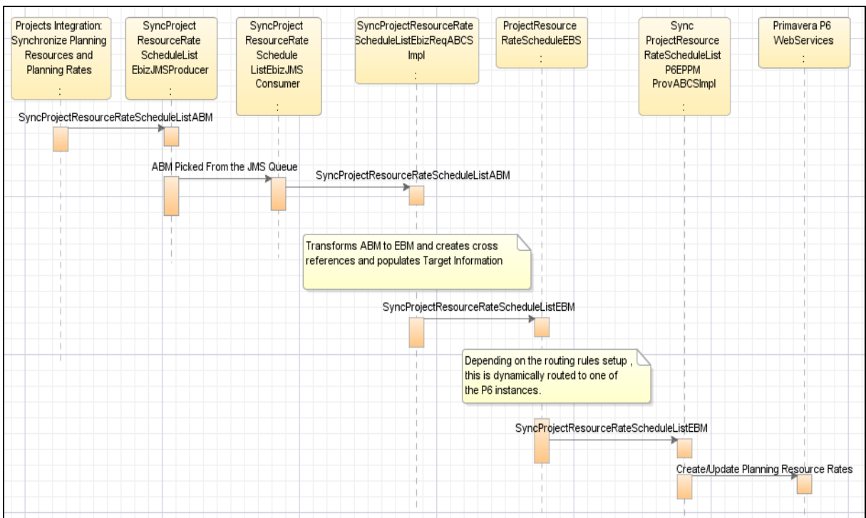
Synchronization of Planning Resource Rates or Role Rates integration flow sequence diagram
