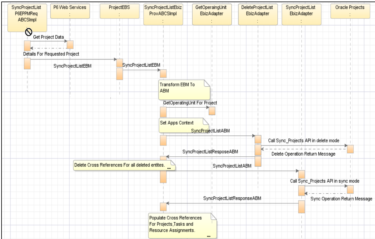
SyncProjectListEbizProvABCSImpl sequence diagram
