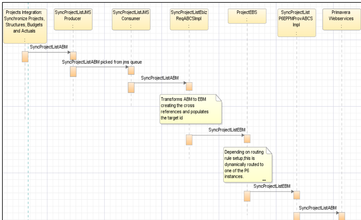
SyncProjectListEbizReqABCImpl sequence diagram
