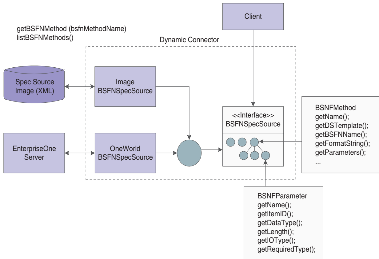
Figure 10–1 Relationships among BSFNSpecSource, BSFNMethod, and BSFNParameter
