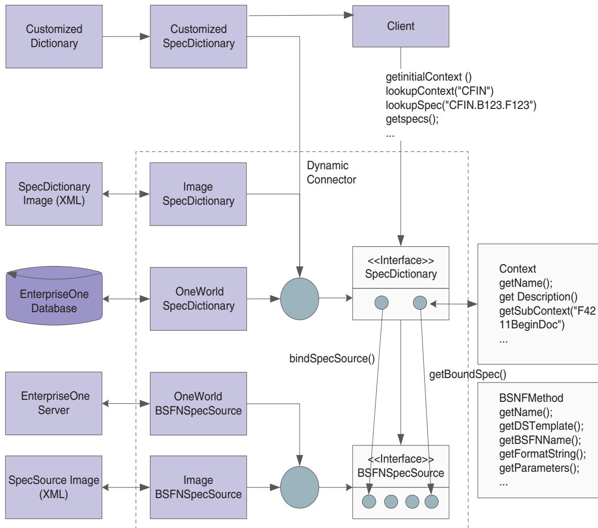
Figure 10–2 Relationship between SpecDictionary and BSFNSpecSource
