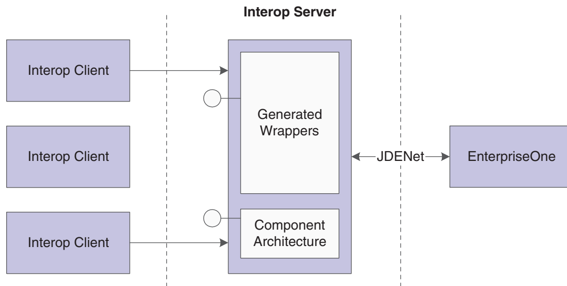
Figure 4–1 COM server deployment
