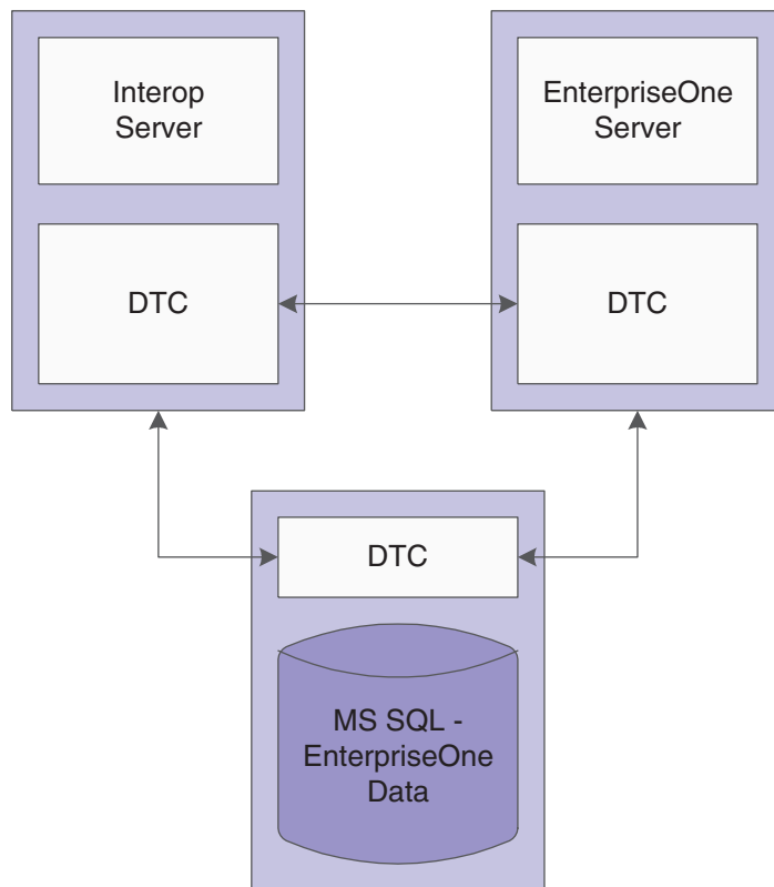
Figure 5–1 COM+ Environment Configuration
