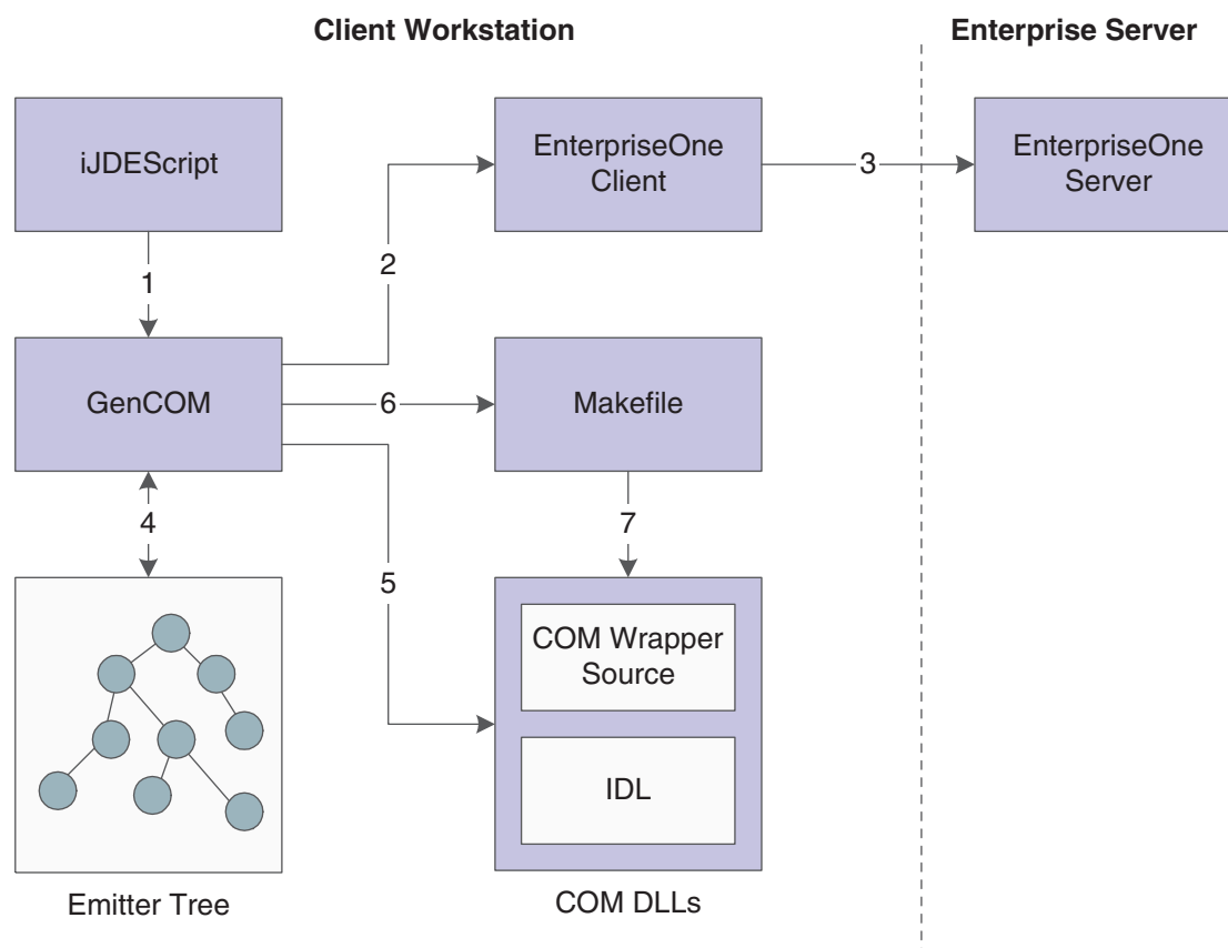
Figure 3–2 GenCOM process
