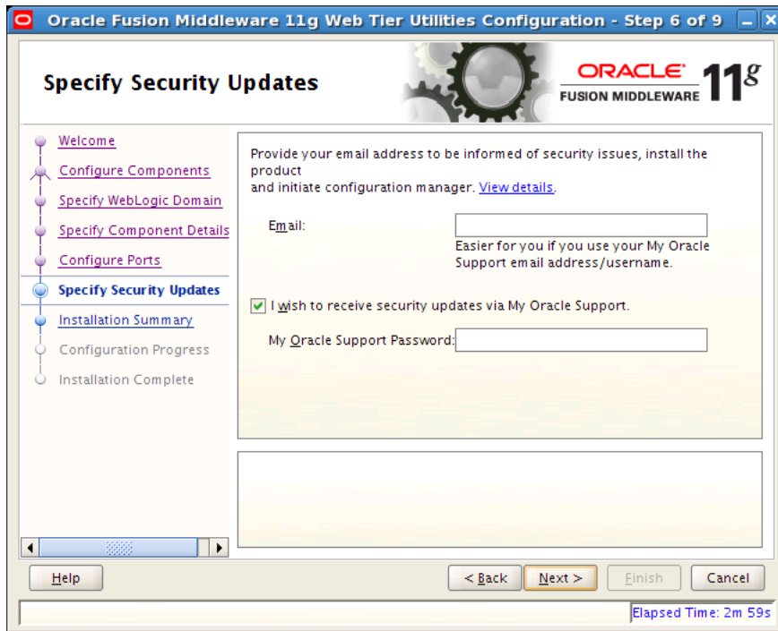
Figure 5–18 Specify Security Updates
