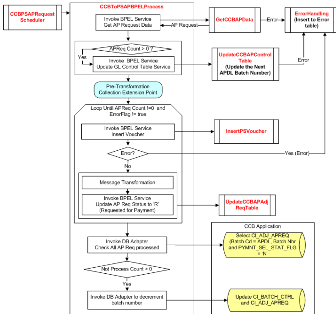
Main BPEL Process - CCBToPSAPBPELProcess
