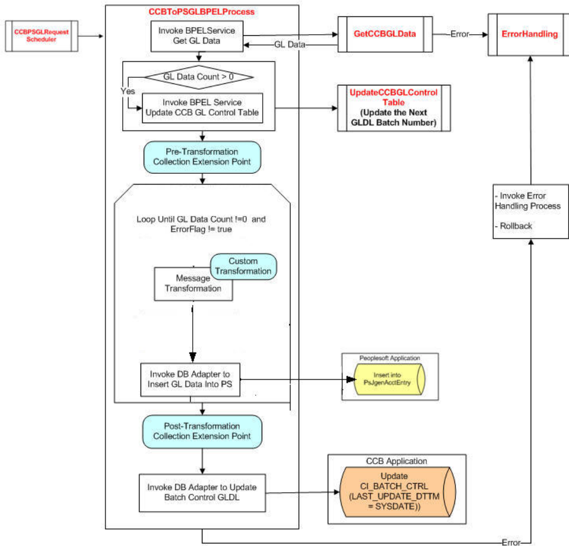
Main BPEL Process - CCBToPSGLBPELProcess
