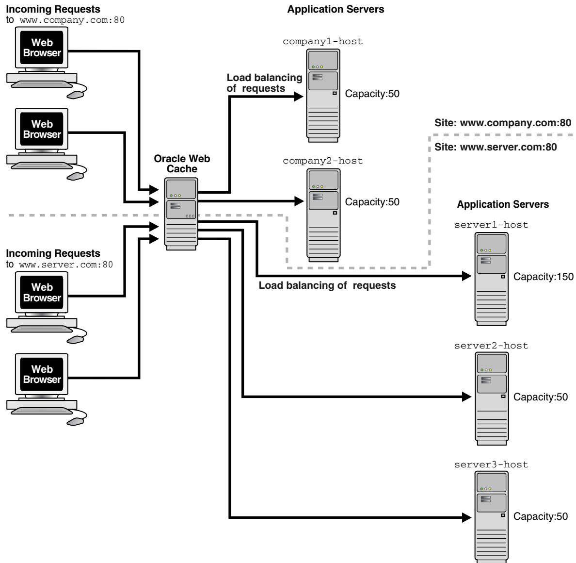
Figure 9–5 Load Balancing
