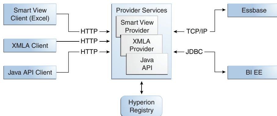
Figure 15–4 Provider Services Single Instance Architecture
