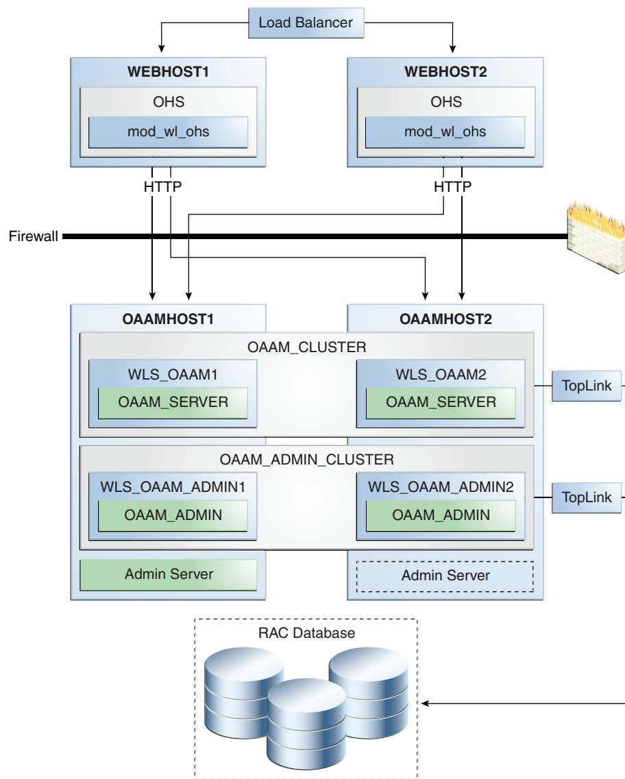
Figure 8–19 Oracle Adaptive Access Manager High Availability Architecture
