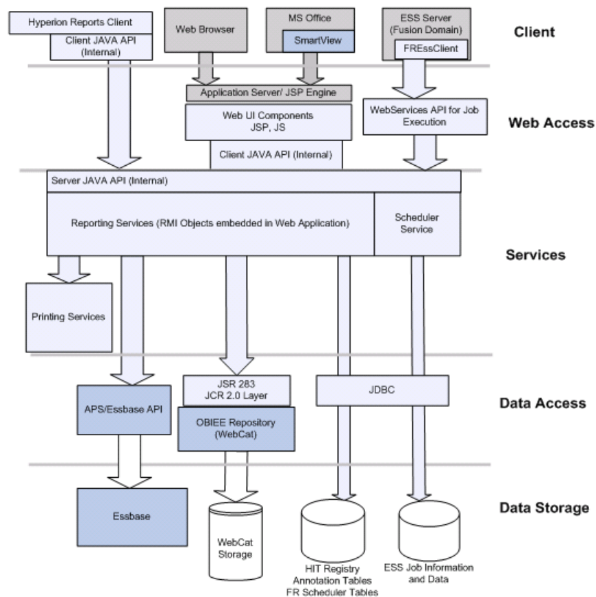
Figure 15–6 Financial Reporting Single Instance Architecture
