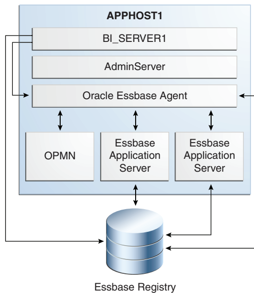
Figure 15–3 Oracle Essbase Single Instance Architecture
