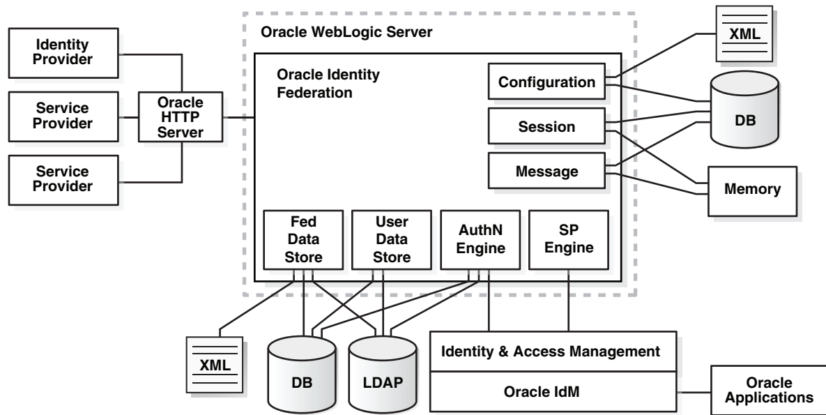
Figure 8–20 Oracle Identity Federation Non-High Availability Architecture
