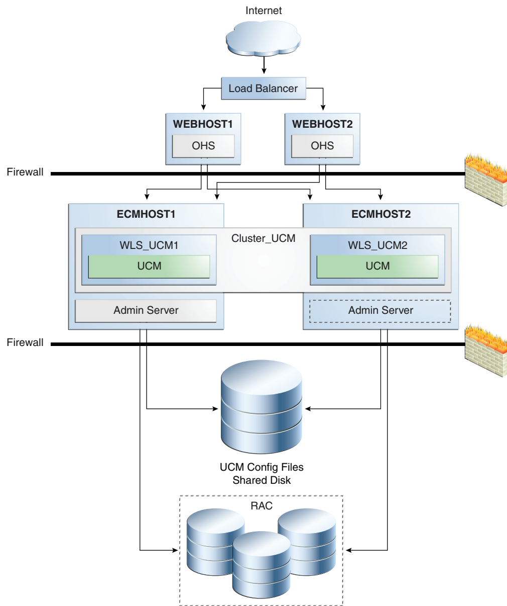
Figure 11–4 Oracle Universal Content Management Two-Node Cluster
