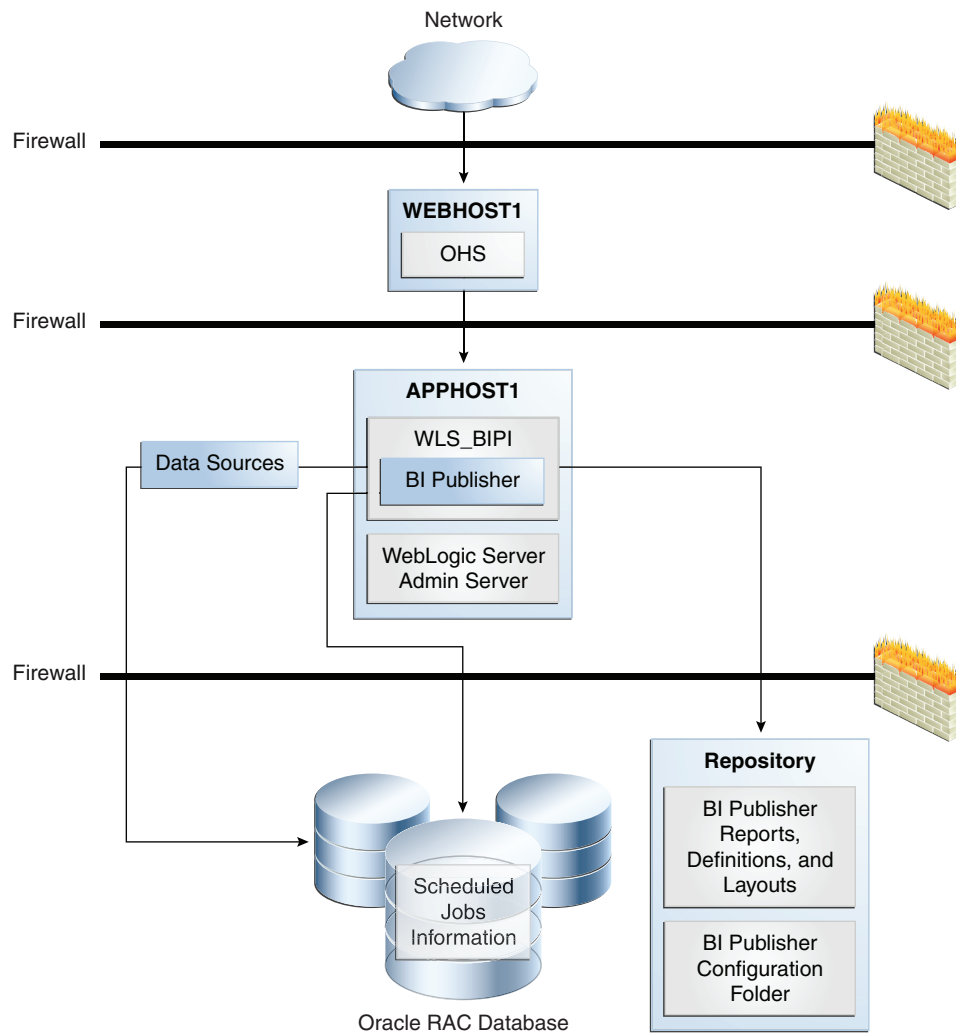
Figure 15–11 Oracle BI Publisher Single Instance Architecture
