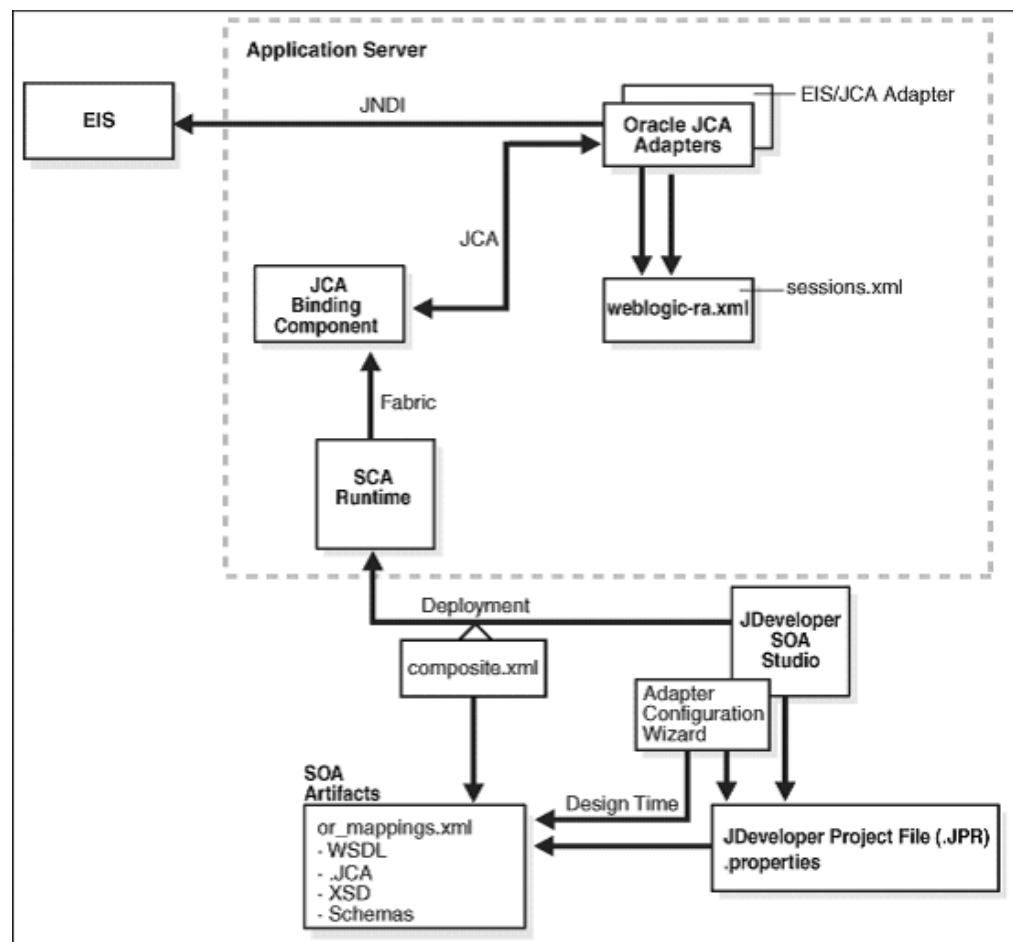
Figure 5–30 Oracle JCA Adapters Single Instance Architecture
