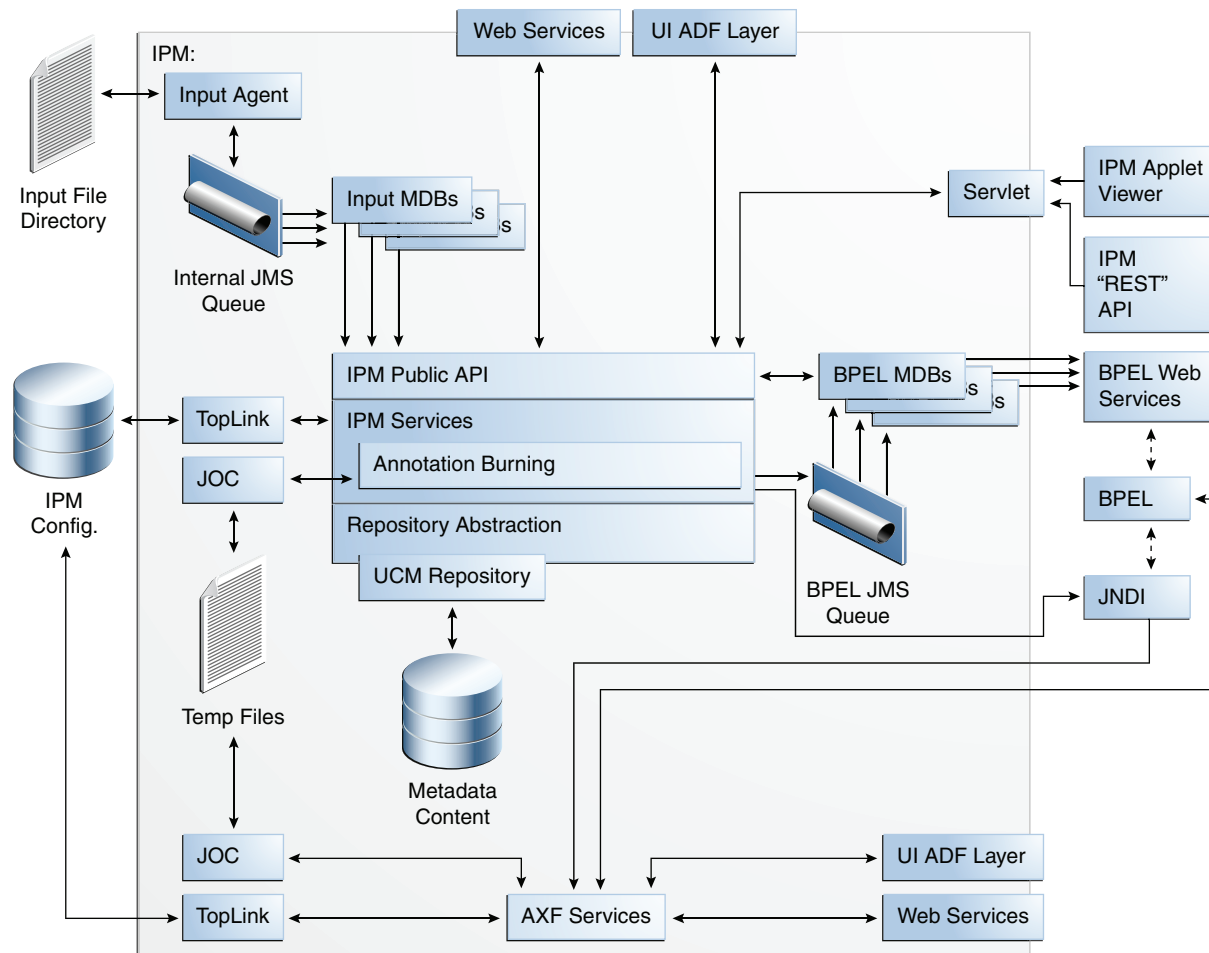
Figure 11–1 Oracle I/PM Components for a Single Instance
