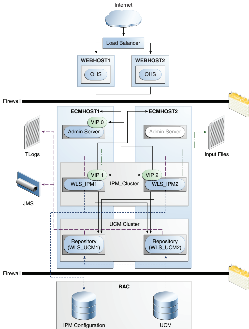
Figure 11–2 Oracle I/PM High Availability Architecture Diagram
