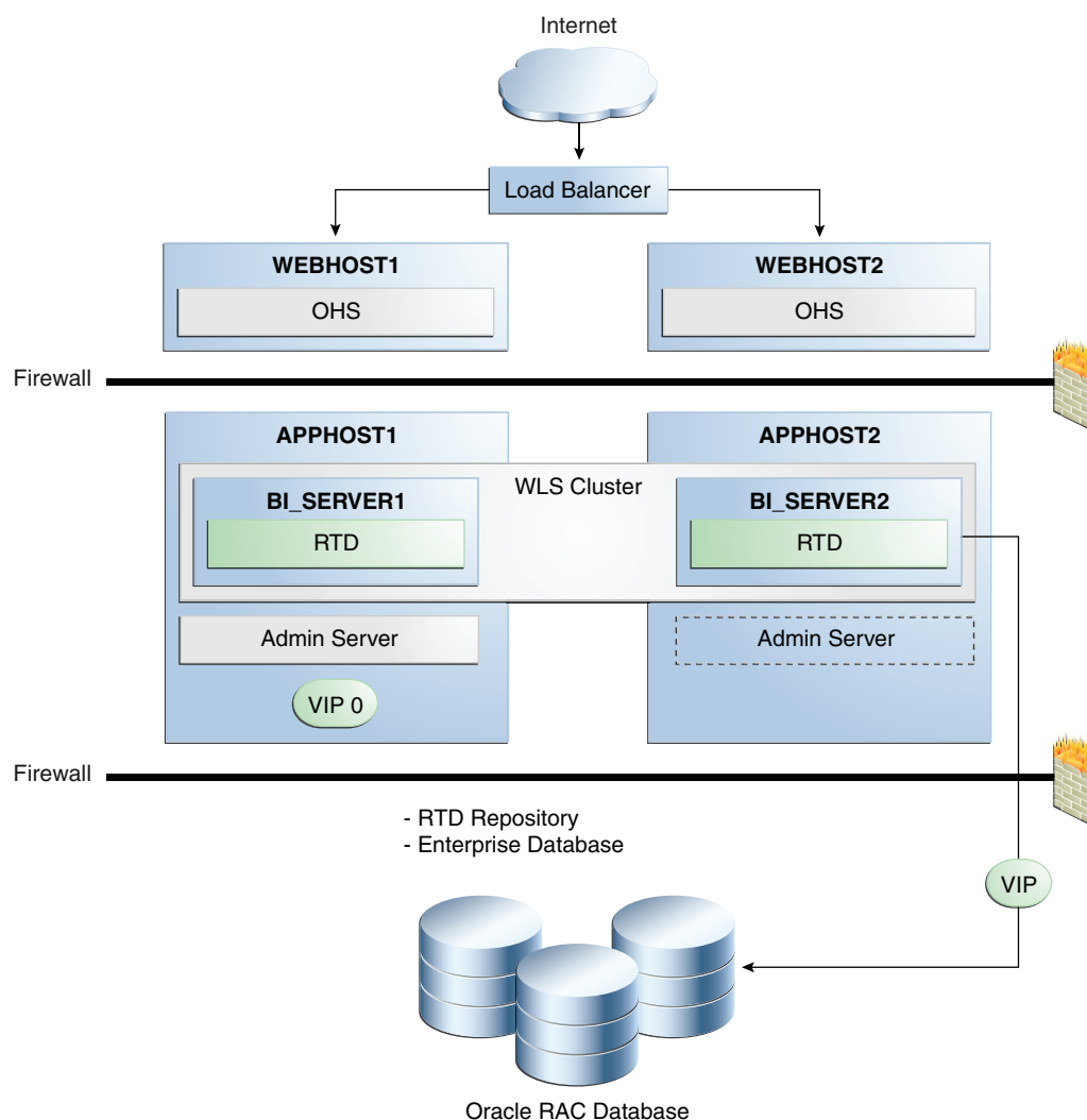
Figure 15-14 Oracle RTD High Availability Architecture
