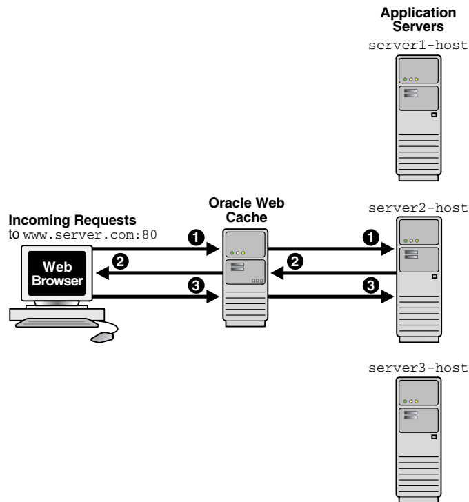
Figure 9–7 Session Binding
