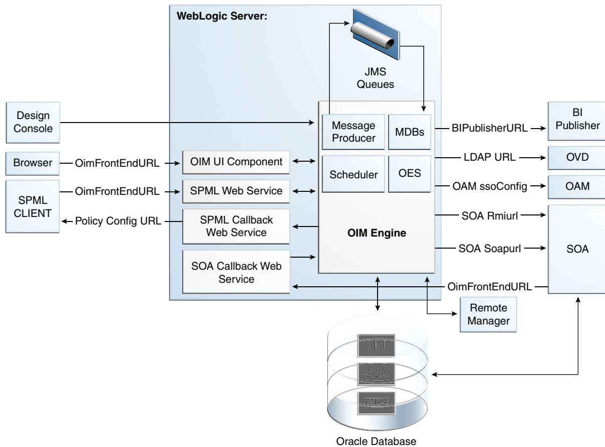
Figure 8–16 Oracle Identity Manager Component Architecture
