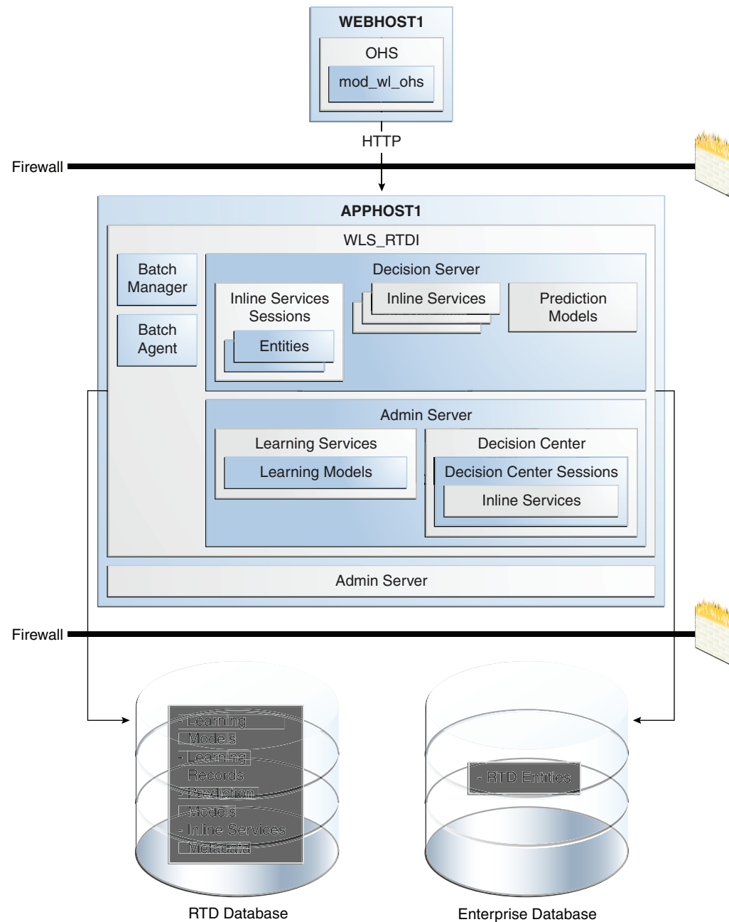
Figure 15–13 Oracle RTD Single Instance Architecture
