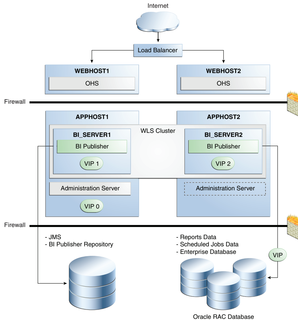
Figure 15–12 Oracle BI Publisher High Availability Architecture
