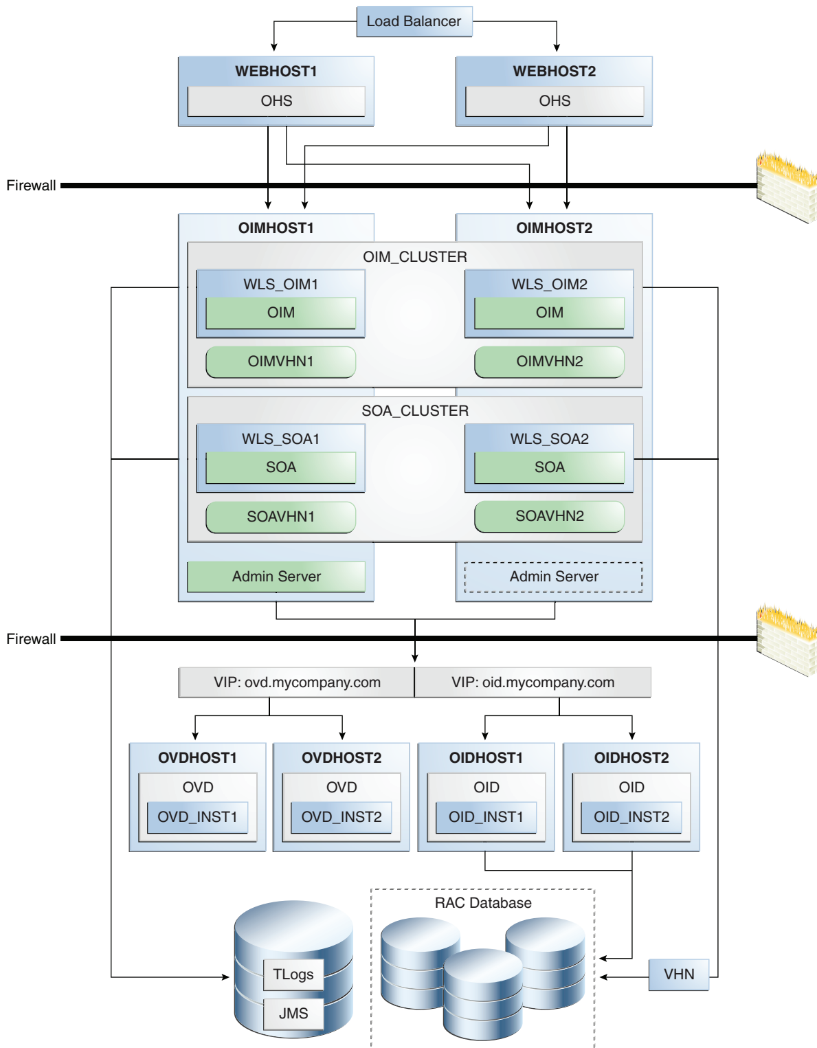
Figure 8–17 Oracle Identity Manager High Availability Architecture
