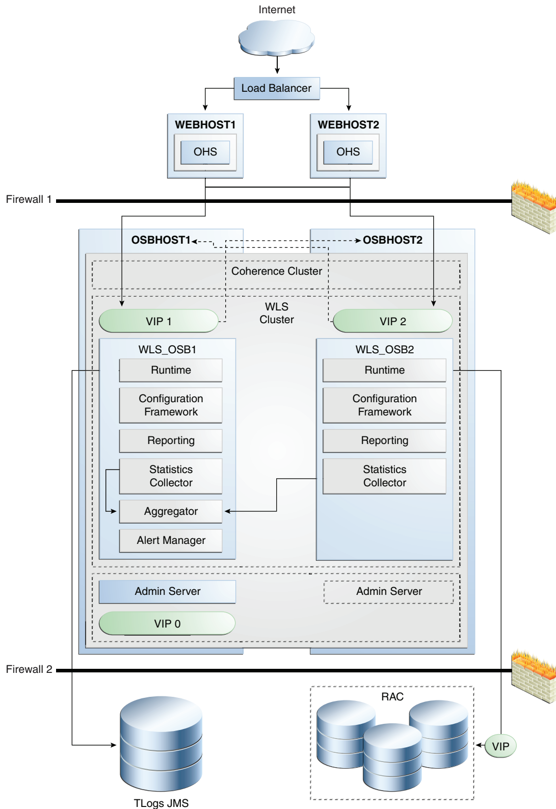
Figure 5–48 Oracle SOA Service Infrastructure, Component Services Engines, and Oracle Service Bus High Availability Architecture
